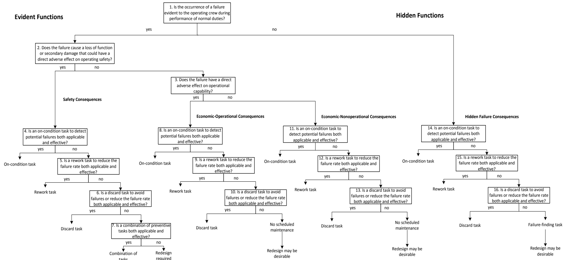
Figure 1. RCM decision diagram (after Nowlan and Heap 1978, 92–93)
