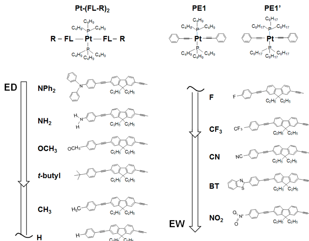
Figure 1. Chemical structures of the Pt complexes \text{Pt}(\text{FL-R})_2 , corresponding ligand chromophores FL-R, and Pt-core model chromophores PE1 and PE1'. Arrows indicate increase of EW ability.
