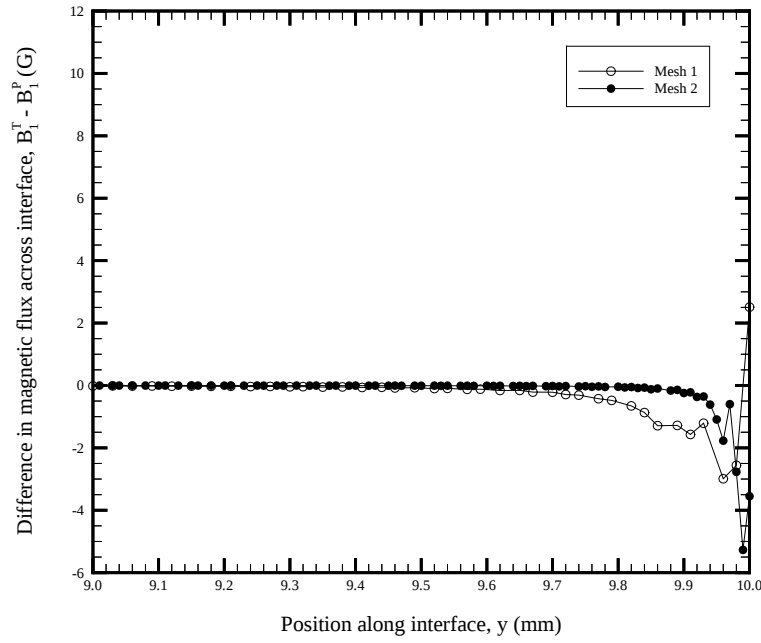
Figure 4.5: Difference in magnetic flux, B_1 , across interface at upper 10% of the composite cylinder model.
