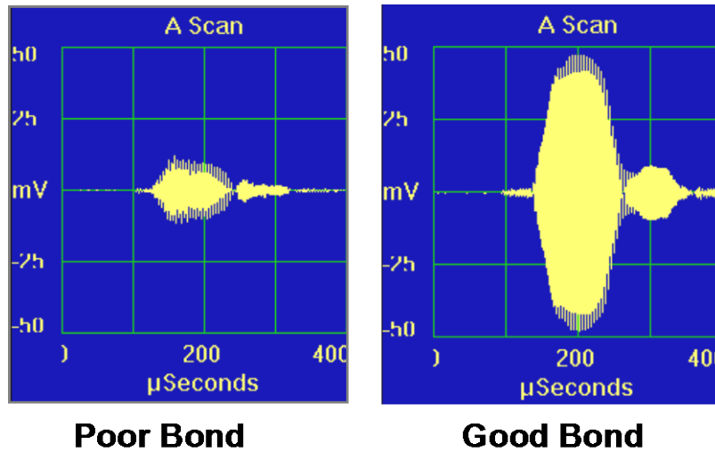
Figure 8. A-scan graph showing amplitude response.
