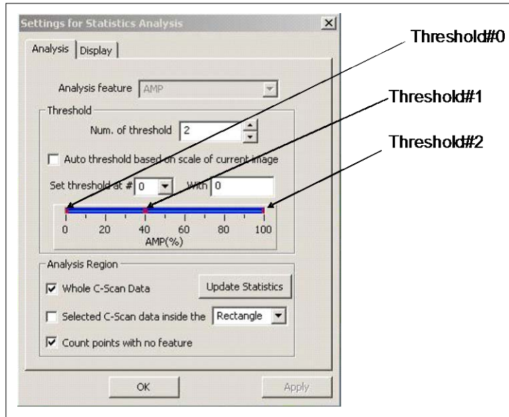
Figure 11. Statistical toolbox.
