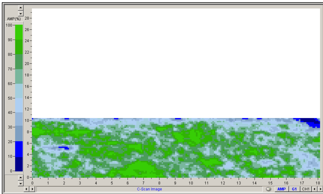
Figure 9. C-scan image.
