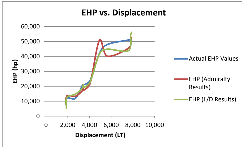
Figure 17. EHP versus Displacement.
