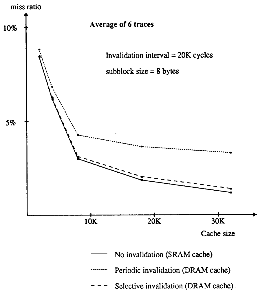
Figure 3-10. Effect of selective invalidations for different size of sub-block
