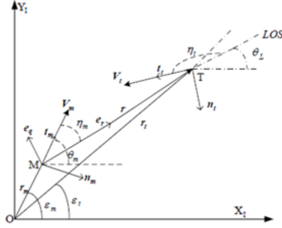
Figure 2. Typical DG encounter geometry (after [12]).
