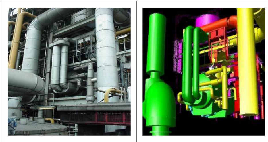
Figure 10. 3D Model of Industrial Piping (from Quintero et al., 2008)
