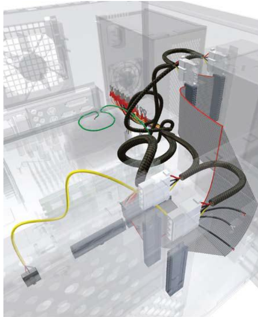
Figure 20. Digital Prototype Example (from Autodesk, 2009)
