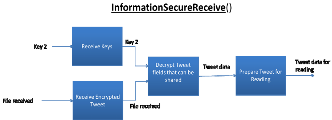
Figure 38. InformationSecureReceive() algorithm.
