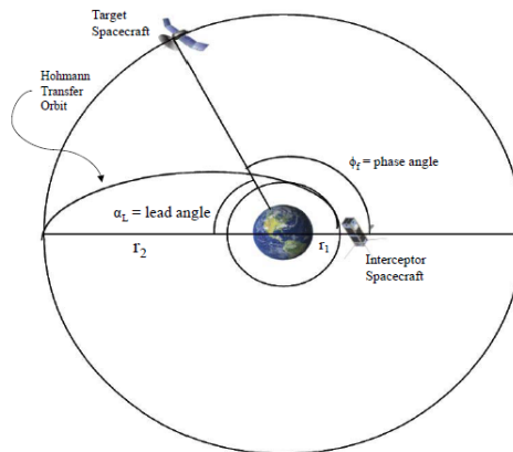
Figure 21. Geometry Depicting Rendezvous between Two Circular, Coplanar Orbits. 102
