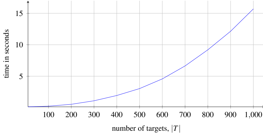
Figure 2.3: Convex Hull LP Run Time - For small numbers of targets the LP runs very quickly. Run Times, however, grow very quickly with the number of targets.
