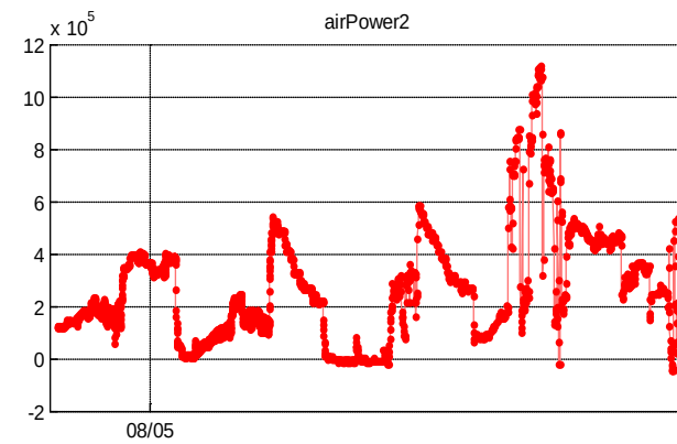
Figure B.3.20 AHU cooling system fault detection results without using T_out_chw and direct AHU air flow measurement
