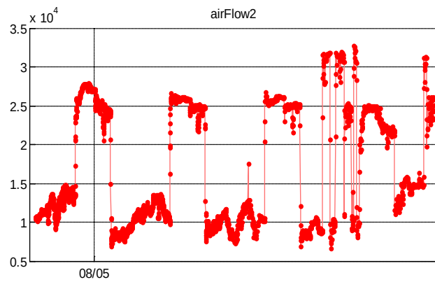
Figure B.3.20 AHU cooling system fault detection results without using T_out_chw and direct AHU air flow measurement
