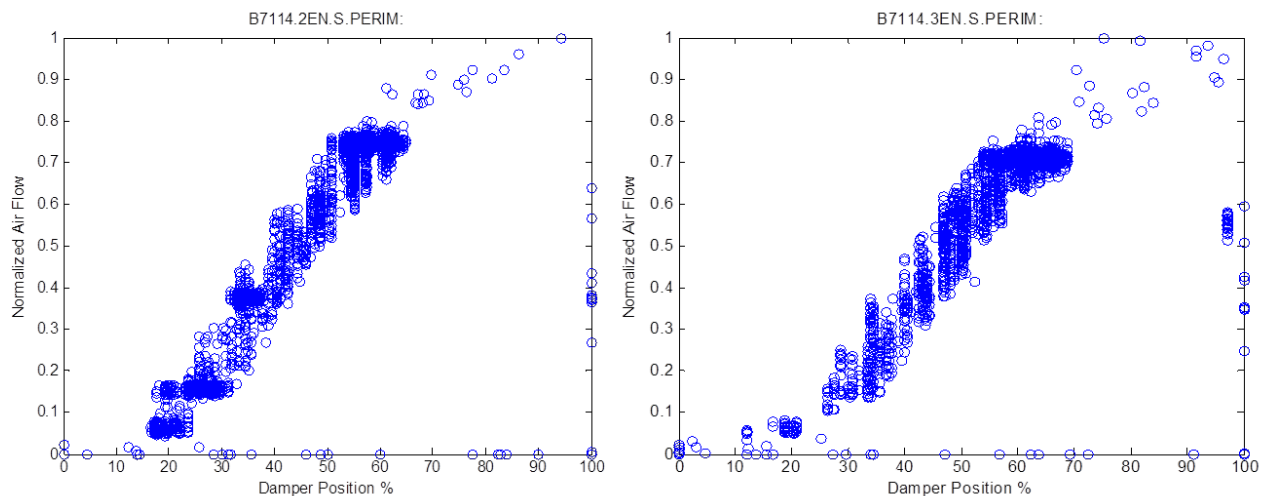
Figure B.3.2 Nominal VAV air flow characteristics
