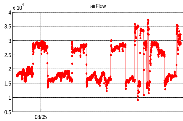
Figure B.3.18 AHU cooling system fault detection results without using T_out_chw
