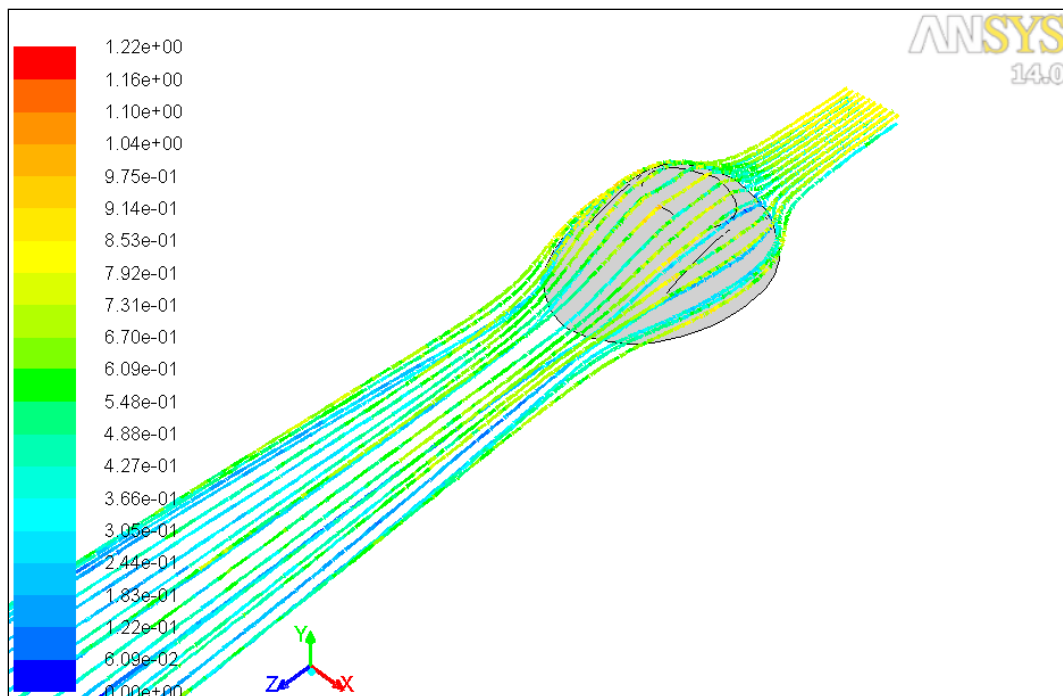
Figure 45: Flow Pathlines for Indented Shell at 10m/s
