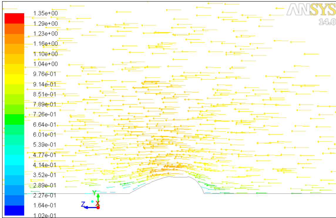
Figure 46: Velocity Vectors for Indented Shell at 10m/s
