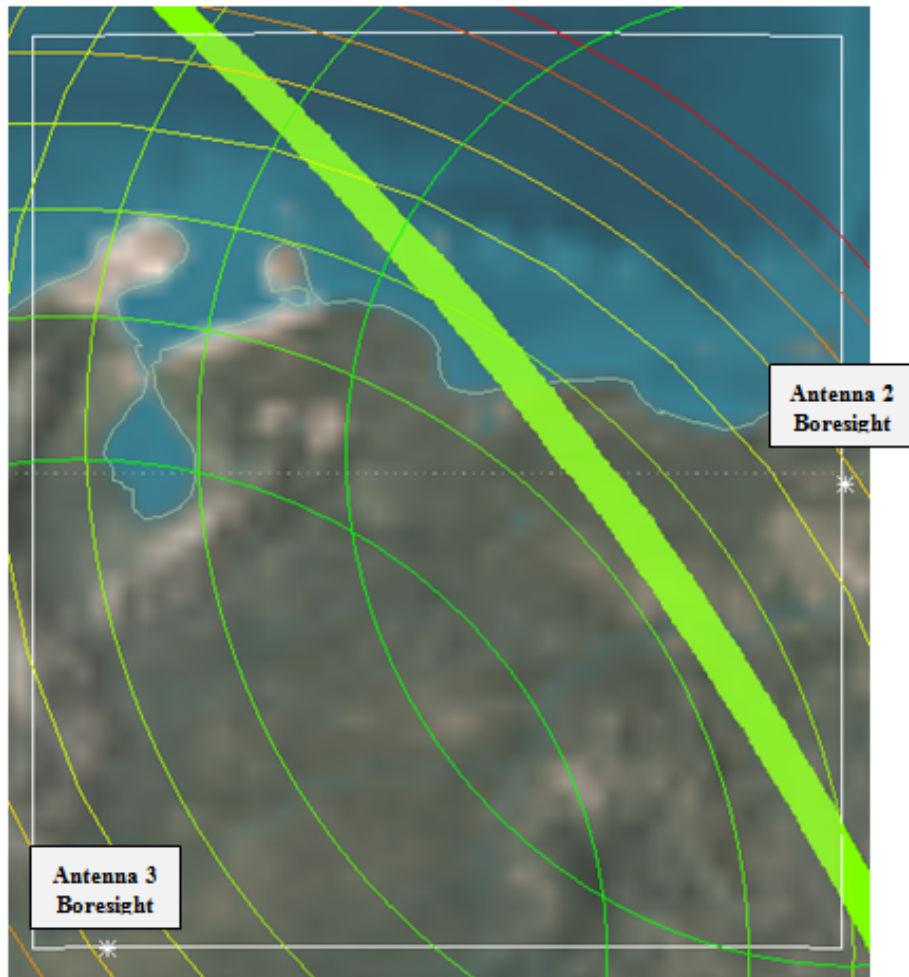
Figure 25. Single Difference Contour ( G_2 - G_3 ).
