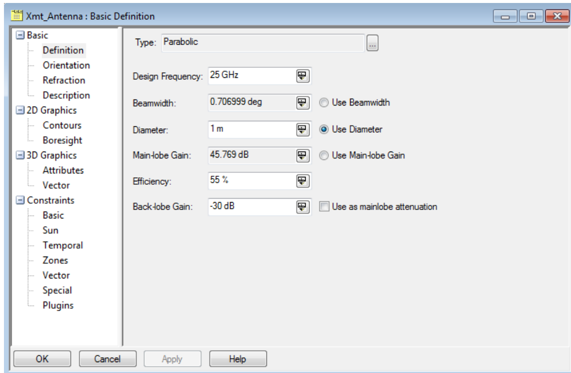
Figure 37. Modeling the Ka Band Transmitter Antenna in STK.
