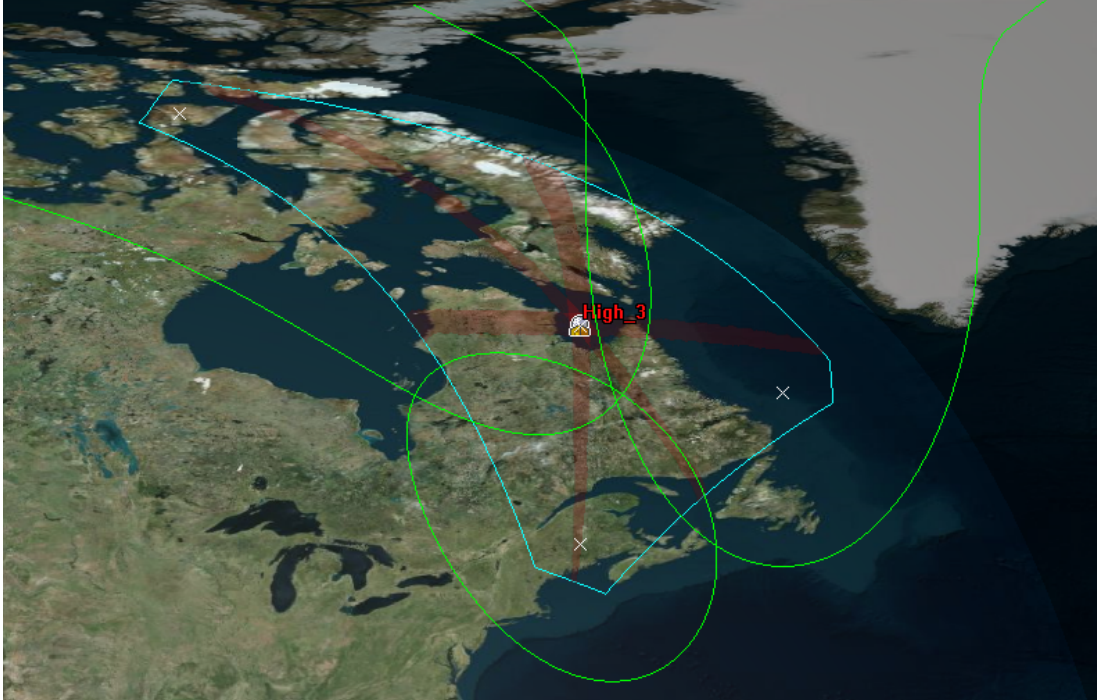
Figure 91. High Latitude Model – Geolocation of Interfering Transmitter #3.
