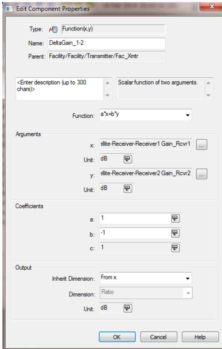
Figure 43. STK Analysis Workbench User Defined Function (x, y) Component.
