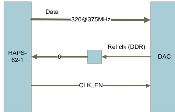
Figure 72 TIPD-3200 architecture
