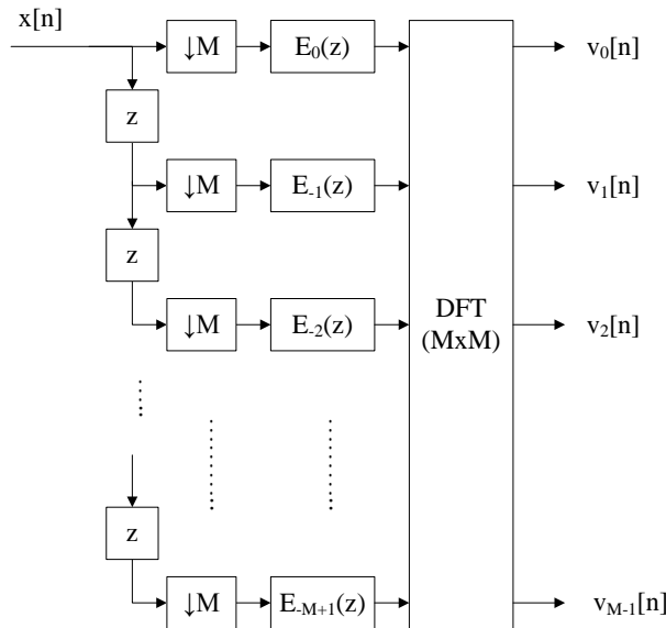
Figure 79 Apply Noble identity to polyphase representation
