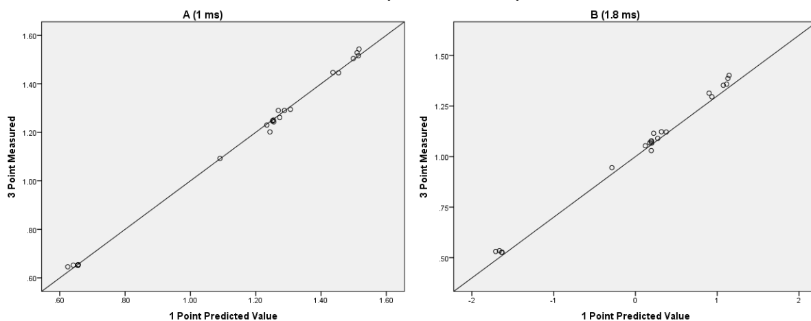
Figure 2. Predictions of clo using 1 point estimation method compared to 3 point measured for a) 1 m/s and b) 1.8 m/s
