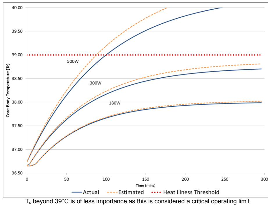
Figure 5. Impact of using estimated and actual aV^g values to model desert conditions (48.89°C; 20% RH, 1 m/s) at three work intensities (180, 300, 500W)
