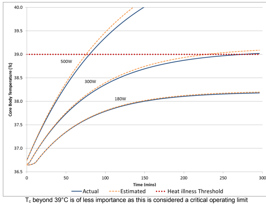
Figure 4. Impact of using estimated and actual aV^g values to model jungle conditions (35°C; 75% RH, 1 m/s) at three work intensities (180, 300, 500W)
