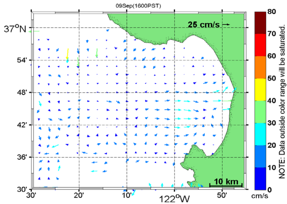
Figure 61. Surface Current Map at 4 p.m. on September 9, 2009.
