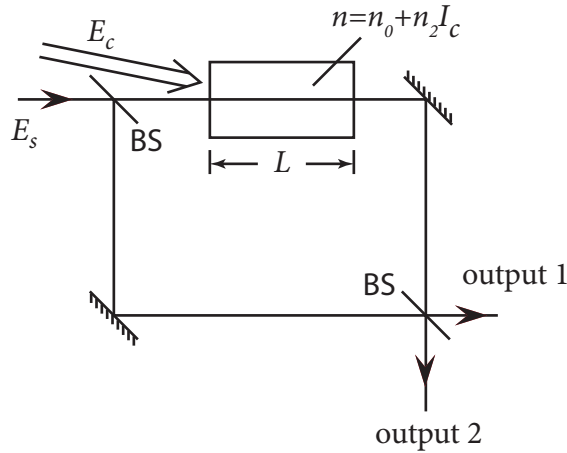
Figure 1.1: The intensity-dependent phase shift experienced by a beam propagating through a nonlinear medium can be used to construct an all-optical switch by placing a nonlinear medium in one arm of an interferometer. A strong control beam affects the nonlinear phase shift and thus the interferometer output.
