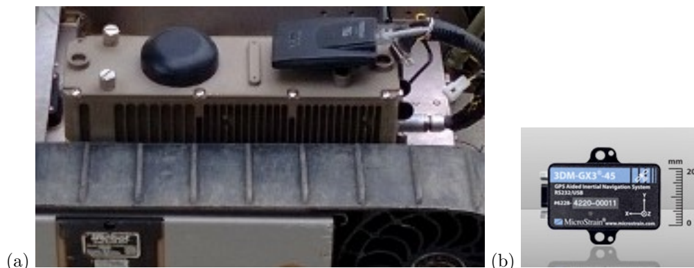
Figure 3. (a) IMU payload on an iRobot PackBot , (b) MicroStrain 3DM-GX3 ® inertial sensor. (Figure courtesy of www.microstrain.com )
