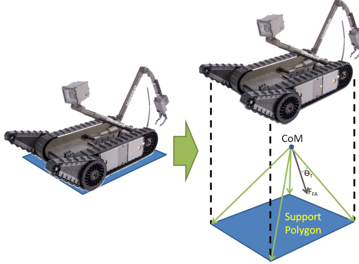
Figure 2. Tip-over angle definition in Force-Angle stability measure
