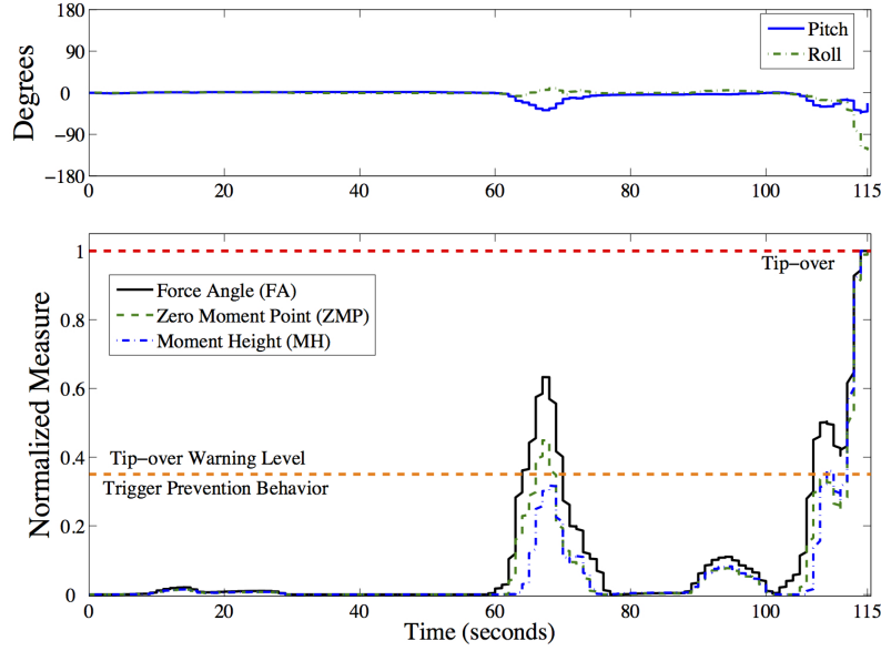
Figure 8. Tip-over detection measures
