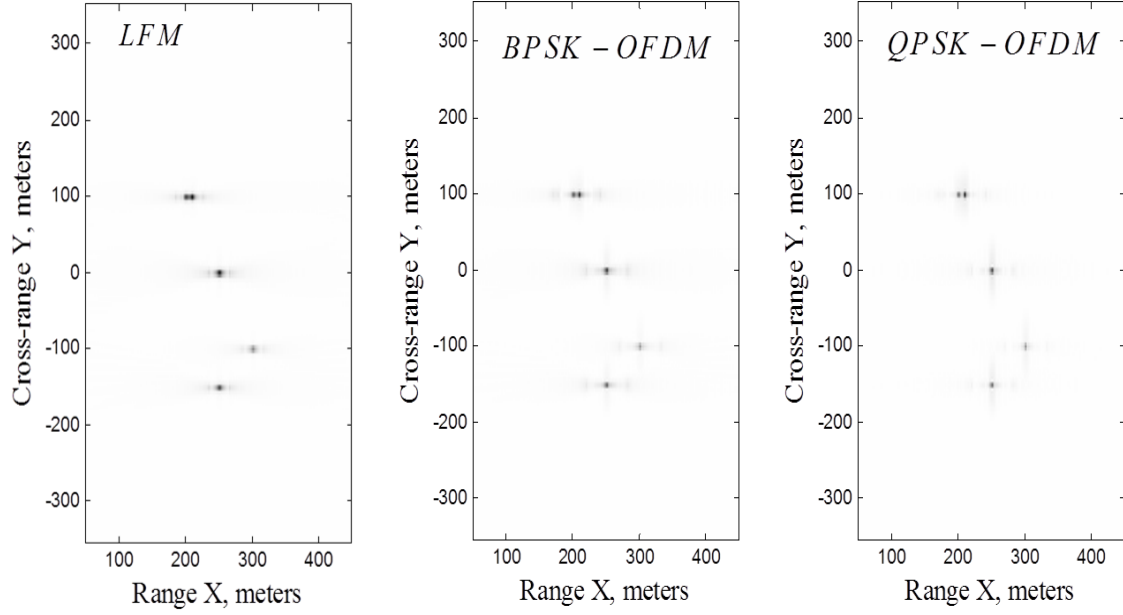
Figure 55. Reconstructed target function for simulation eight with T_p = 0.2 \mu s .
