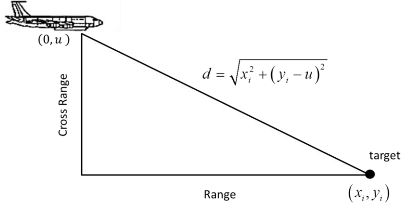
Figure 9. Depiction of slant range distance using Pythagorean theorem.
