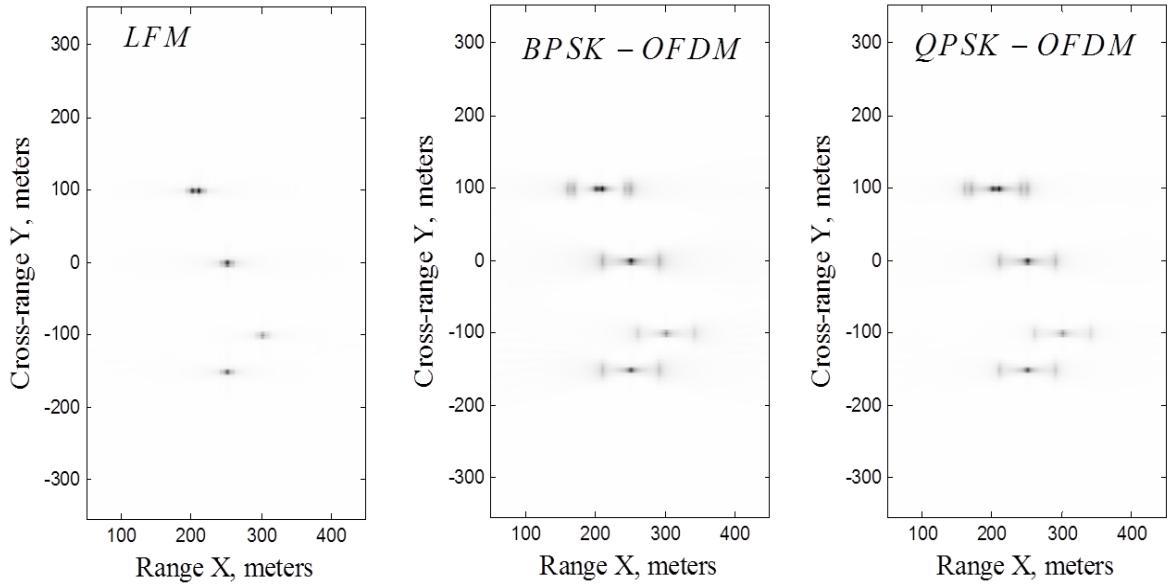
Figure 56. Reconstructed target function for simulation eight with T_p = 0.26667 \mu s .
