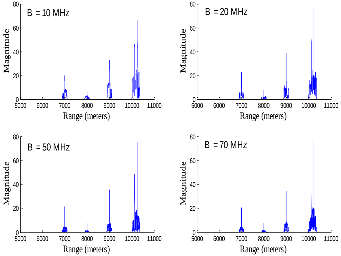
Figure 29. BPSK-OFDM reconstructed range target function: N = 8 , B = 10 MHz, 20 MHz, 50 MHz, and 70 MHz.
