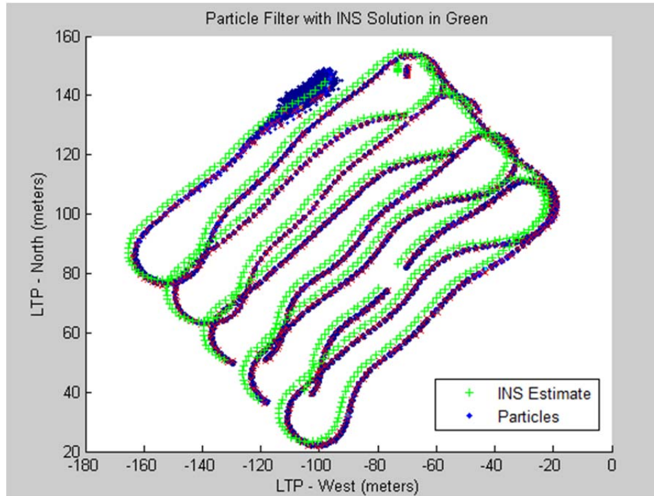
Figure 28. Particle filter with 1,000 particles compared to INS estimation
