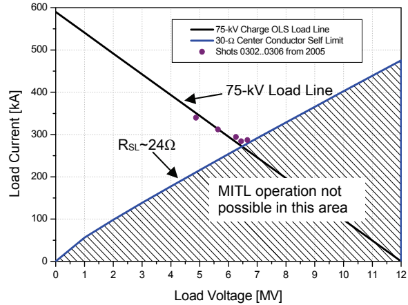
Figure 3. The load line of Mercury from its simple Thevenin equivalent, the self limit curve from the original, 30- \Omega center conductor and actual data from Mercury shots with different load impedances.
