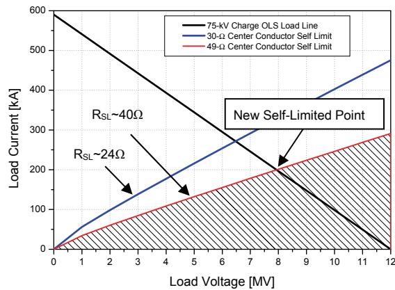
Figure 4. The Mercury 75-kV charge load line with the new self-limited curve given by a new center conductor with vacuum impedance increase from 30 to 49 \Omega to give a 40- \Omega self-limited impedance at 8 MV.
