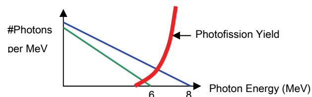
Figure 1. Idealized bremsstrahlung spectra at 6 (green) and 8 MV (blue) output voltage along with a sketch of a photofission yield curve (red).
