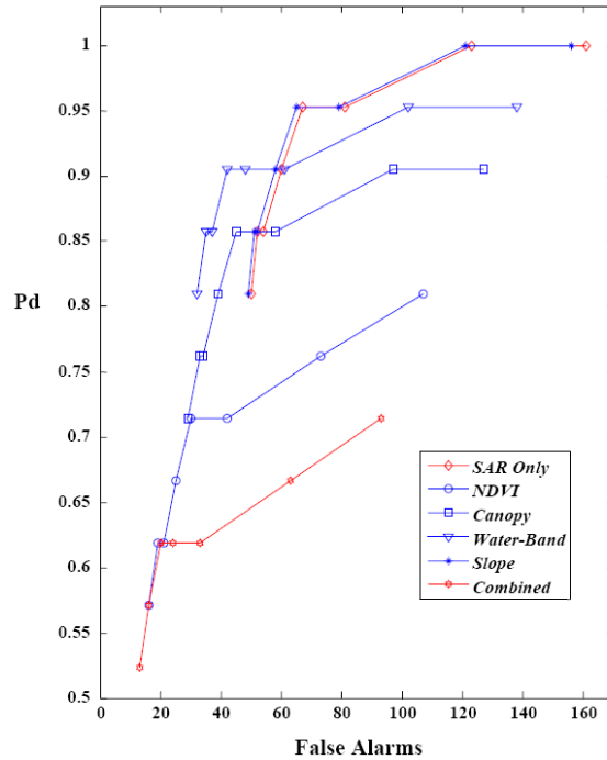
Figure 14. ROC curves for metal targets in the SimOrd calibration area illustrating false alarms and the probability of detection for 21 simulated ordnance targets at various SAR signal amplitude thresholds and using HSI-derived vegetation discrimination masks singly and in combination.
