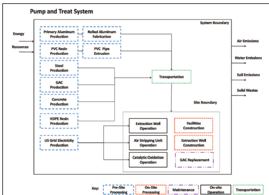
Figure 1: LCA Schematic for Pump and Treat Remedy (Higgins and Olson, 2009)
