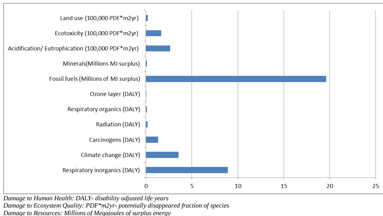
Figure 12: Eco Indicator 99 (E) Impact Assessment for CRREL Alternative 1
