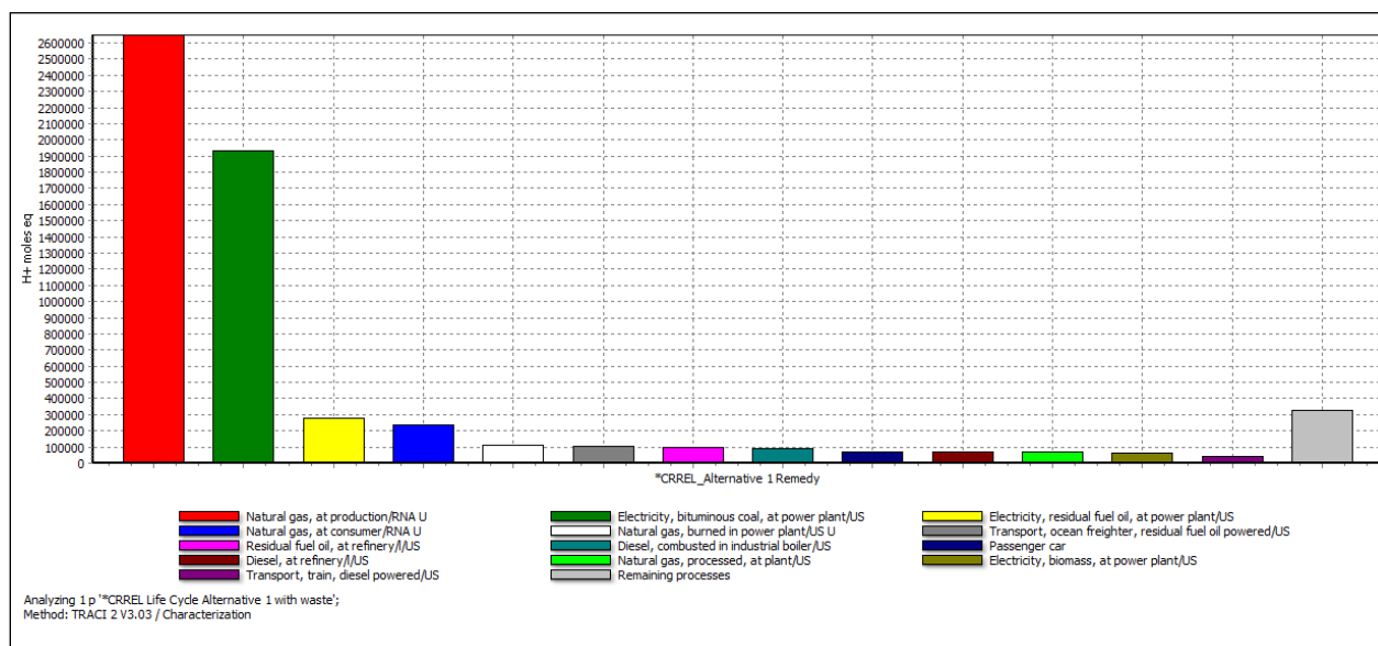
Figure 10: Contributions to the Acidification Impacts for CRREL Alternative 1 Using the TRACI Method
