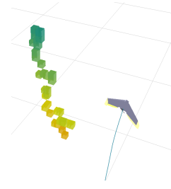
Fig. 9: Obstacle detection from Figure 8 rendered in a 3D visualizer. While we do not endeavor to build maps, our system outputs pointclouds providing compatibility with many existing planning, visualization, and control tools.
