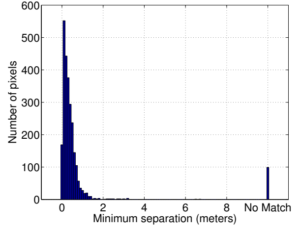
Fig. 10: Results of the comparison as described in Figure 6 (a). Our system produces few outliers (74.8% and 92.6% within 0.5 and 1.0 meters respectively), even as we integrate our state estimate, and the obstacle positions, forward. No Match indicates points that pushbroom stereo detected but there were no block-matching stereo detections on that frame.
