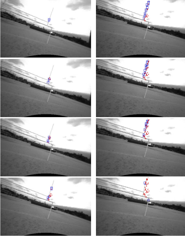
Fig. 8: Sequence of stills from an obstacle detection. Each image is 0.02 seconds (20ms) after the previous. The entire set captures 0.16 seconds. Here, the fieldgoal is detected in the first frames (blue boxes). Afterwards, the position of those detections is estimated via the state estimator and reprojected back onto the image (red dots).
