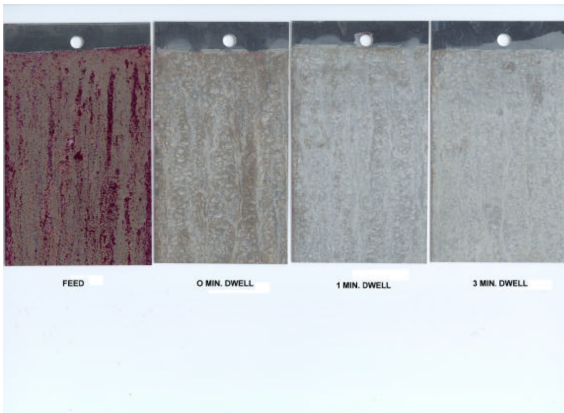
Figure 7.3.5 Optical Photographs of Panels Exposed to 14 Hours of Salt Fog at Various Stages of the Cleaning Process.
