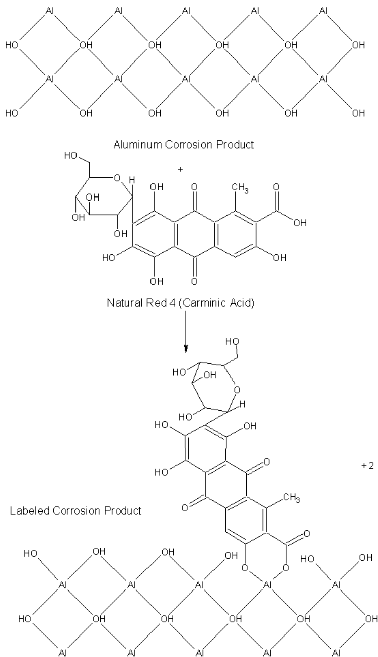
Figure 9.1 Metal Corrosion Product Labeling Chemistry
