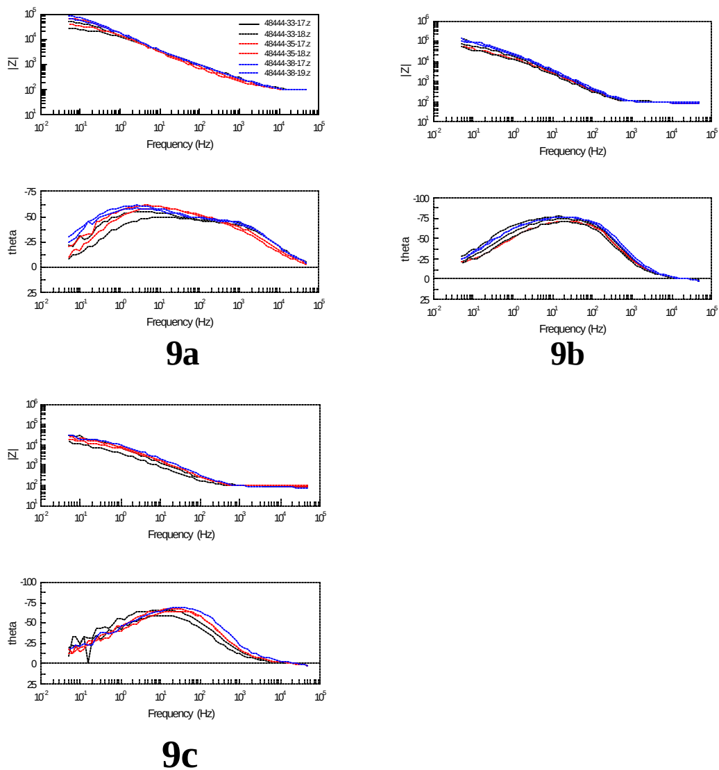
Figure 7.3.1 Bode Magnitude and Phase Angle Plots of Replicate Panels for: 9a) reference, no CRC; 9b) blank, 3 minute CRC dwell; 9c) labeled, 1 minute CRC dwell.
