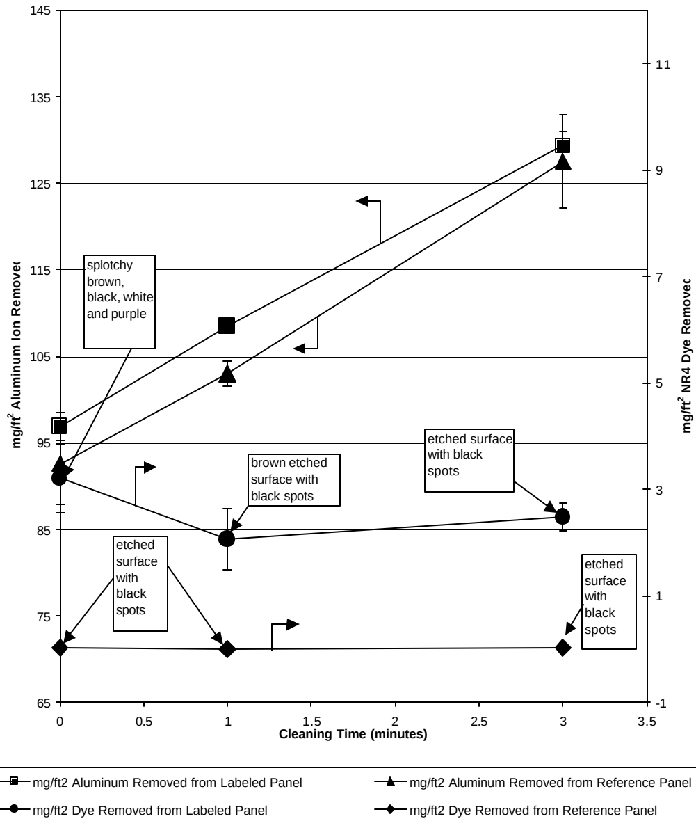
Comparison of Aluminum Ion Removal and Dye Removal v.s. Cleaning Time for Aluminum 2024 Substrate Contaminated with Corrosion and Labeled with NR4
