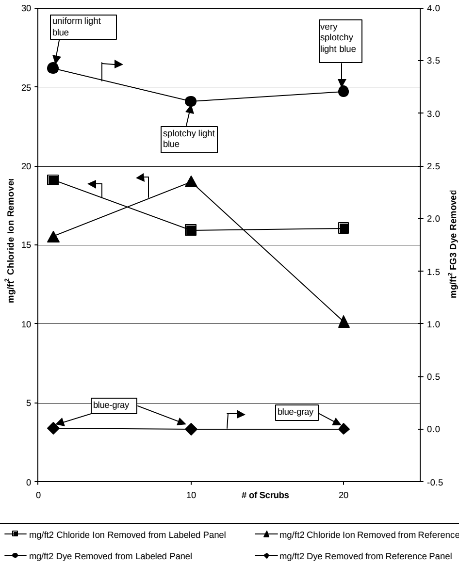
Comparison of Chloride Ion Contaminant Removal and Dye Removal v.s. Cleaning Scrubs for Painted FeHY80 Steel Panels Contaminated with Seawater and Labeled with FG3
