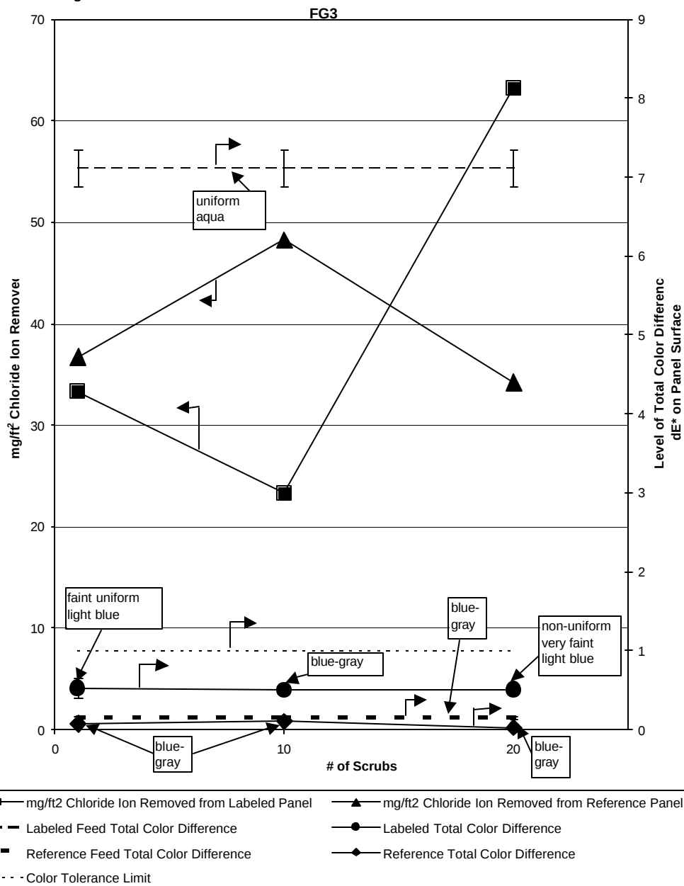
Comparison of Chloride Ion Contaminant Removal and Total Color Difference, dE*, v.s. Cleaning Scrubs for Painted PCMS Tiles Contaminated with Seawater and Labeled with
