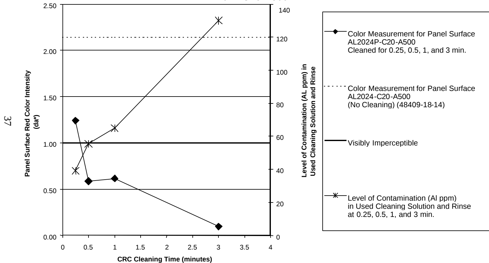
Figure 7.2.1.9 Al2024 Corrosion Product Cleaning MIL-C-38334 (CRC) Cleaner
