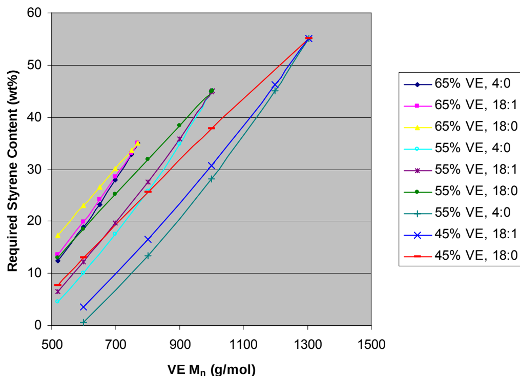
Figure 93. The minimum styrene content required to achieve VE resin viscosities below 500 cP as a function of fatty acid chain length, VE content, and VE molecular weight at 30°C. The operating window is any styrene content above the curve for any molecular weight along the curve. Legend: [Carbon atoms: Unsaturation sites].
