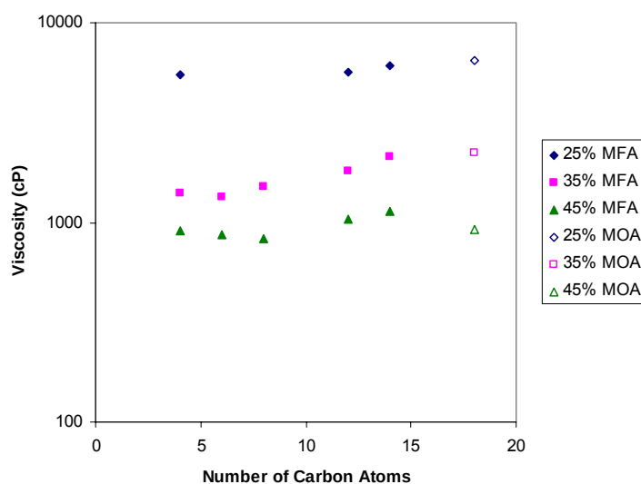
Figure 83. The viscosity of VE/MFA as a function of fatty acid chain length at 25°C.
