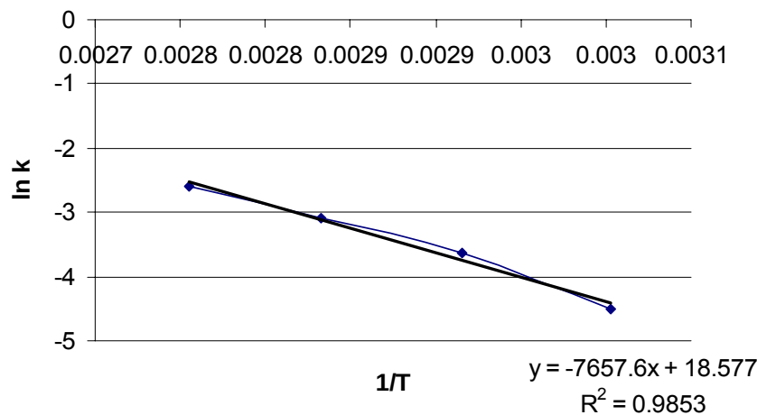
Figure 144. Plot of \ln(k) versus 1/T used to determine E_a and A_0
