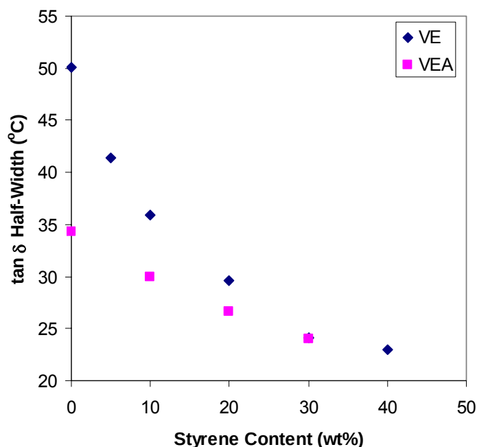
Figure 122. The width of the \tan \delta peak at half-height for VE and VEA resins using 45% reactive diluent (MLau and styrene) as a function of styrene content.
