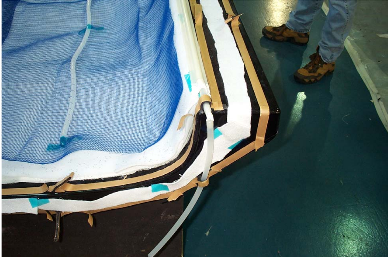
Figure 169. Photograph showing the two rows of tacky tape, the breather cloth, and the method with which the inlet and outlet lines enter the inner mold area.
