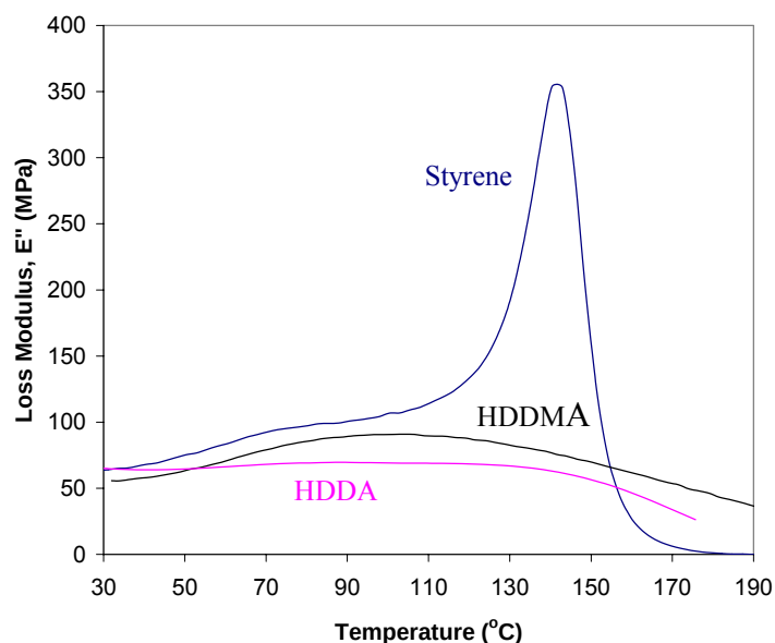
Figure 64. The loss modulus as a function of temperature for VE/HDDA relative to VE/HDDMA and VE/styrene.
