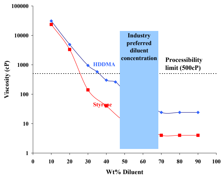
Figure 59. The viscosity of VE 828 resins as a function of styrene and HDDMA content at 30°C.
