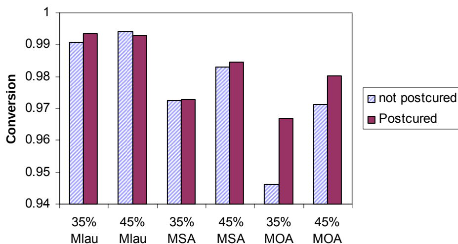
Figure 104. The effect of post-cure on the conversion of E-beam cured VE/MFA polymers.
