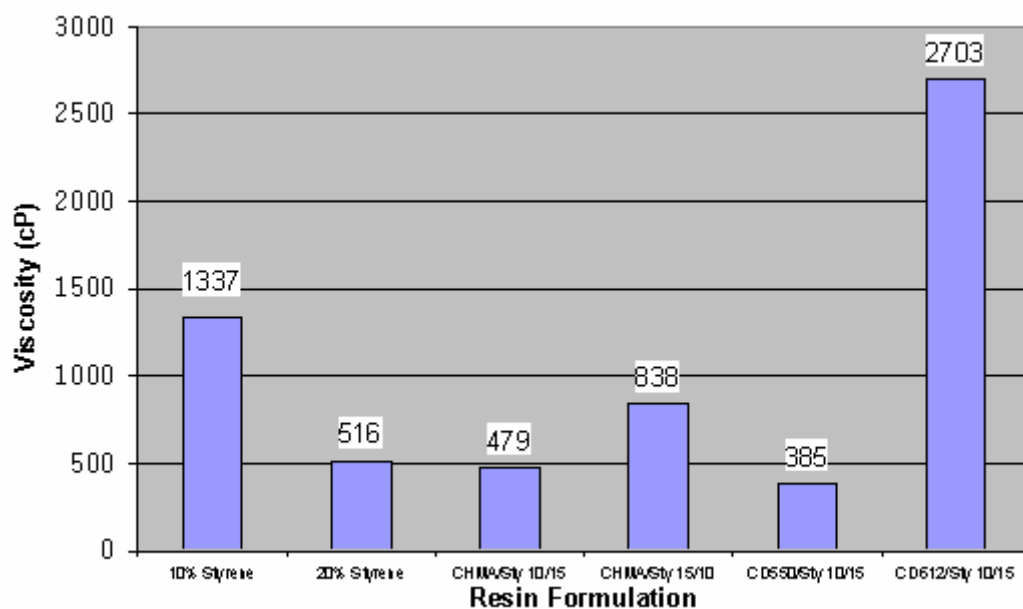
Figure 132. Viscosity as a function of mono-functional resin formulation for resins with 65% CN151.
