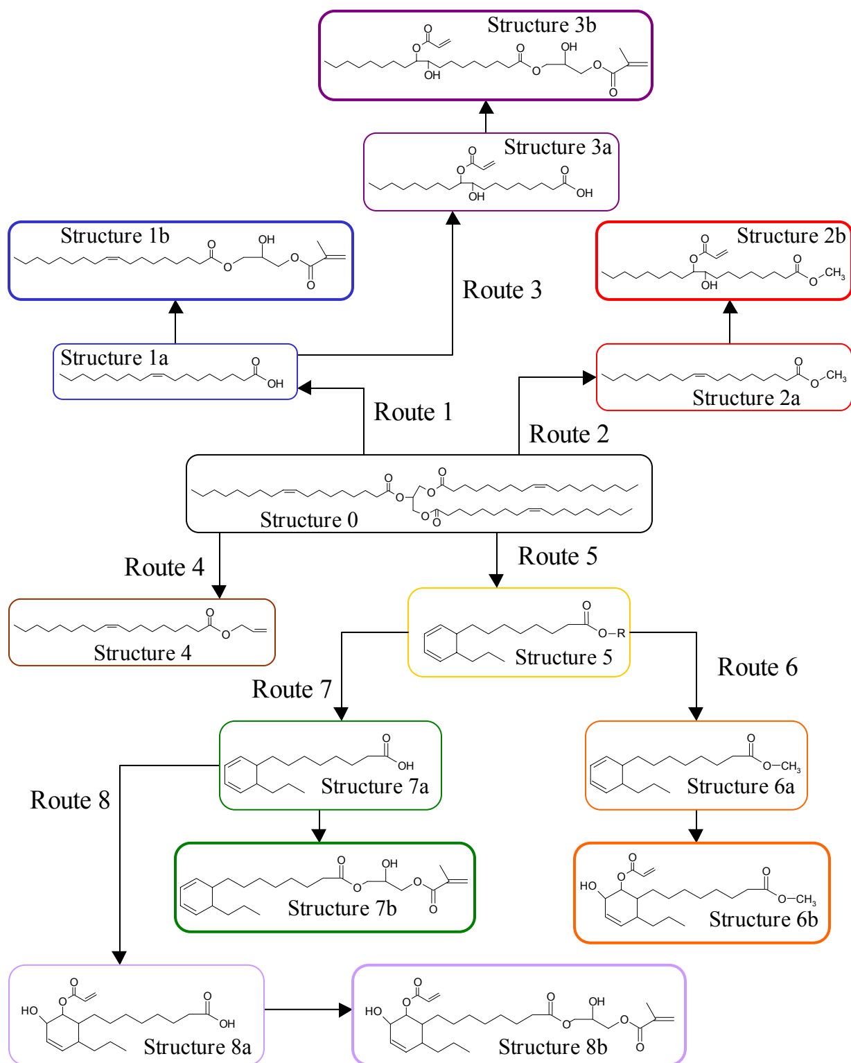
Figure 66. The proposed synthetic routes to produce fatty acid-based monomers [43].
