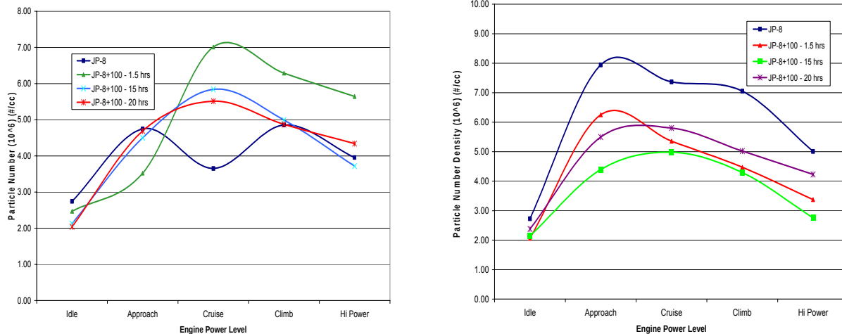
Figure 193. PND as a Function of Power Setting for T-43 Engines 607 and 613.
