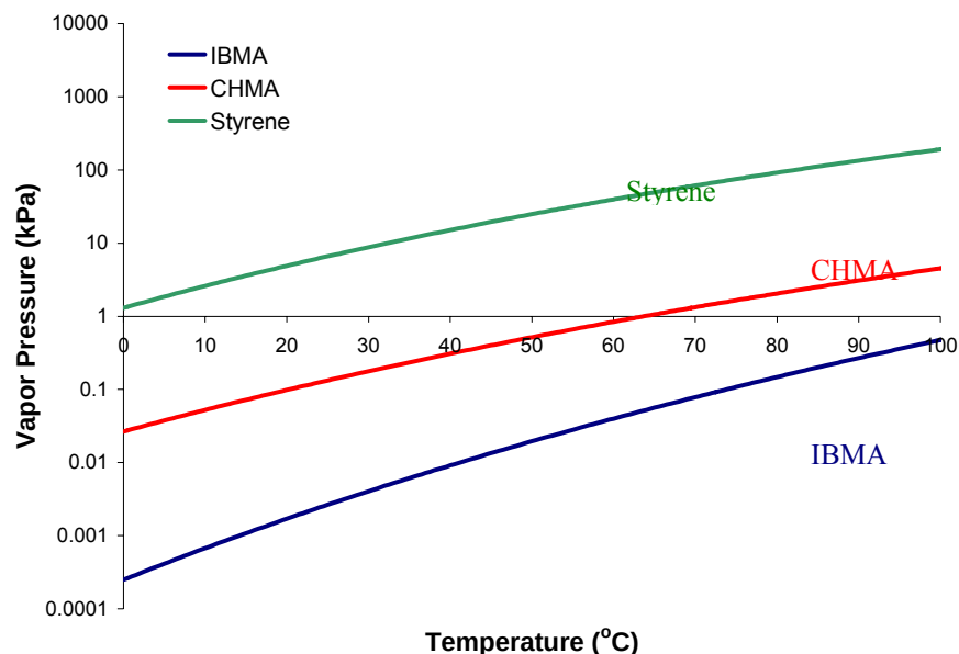
Figure 57. The vapor pressure of styrene, cyclohexyl methacrylate, and isobornyl methacrylate as a function of temperature as calculated with the Antoine Equation.
