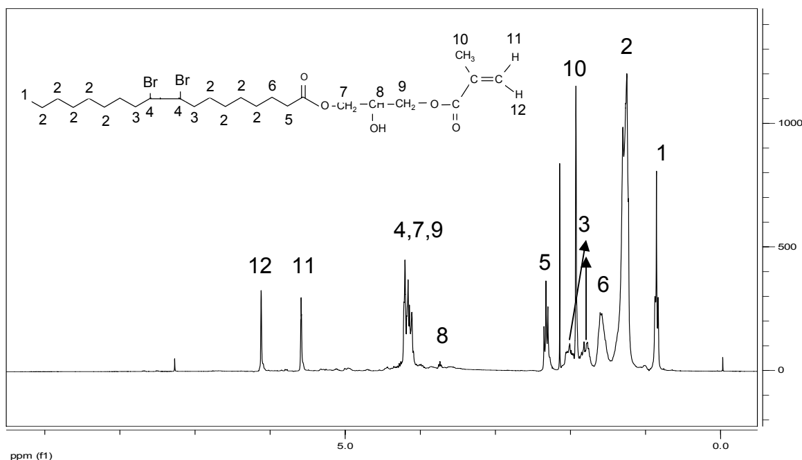
Figure 74. The ^1\text{H-NMR} spectrum of dibromo stearyl glycidyl methacrylate (Di-BrMSA)
