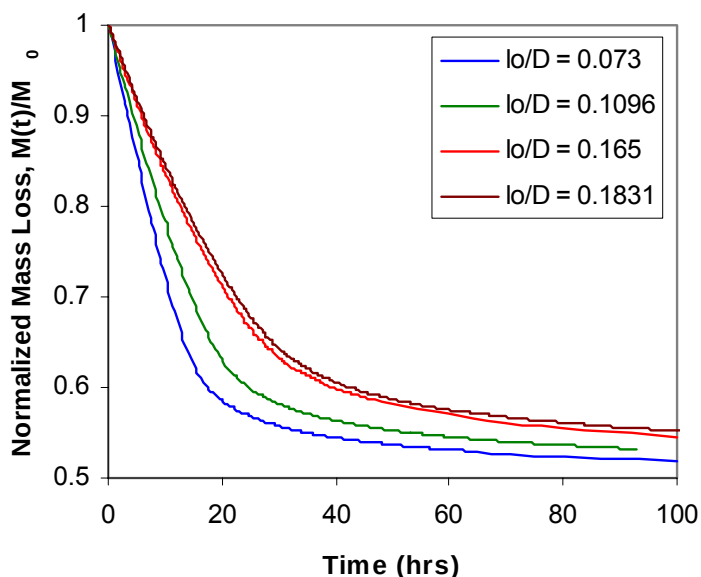
Figure 17. Fractional mass loss of styrene in the VE 828 resin system under 40°C isothermal conditions in the study of depth variation.
