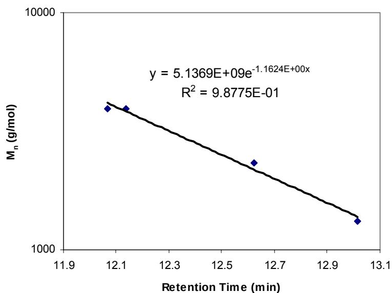
Figure 7. SEC Calibration curve for resin MBBn BBas a function of retention time.
