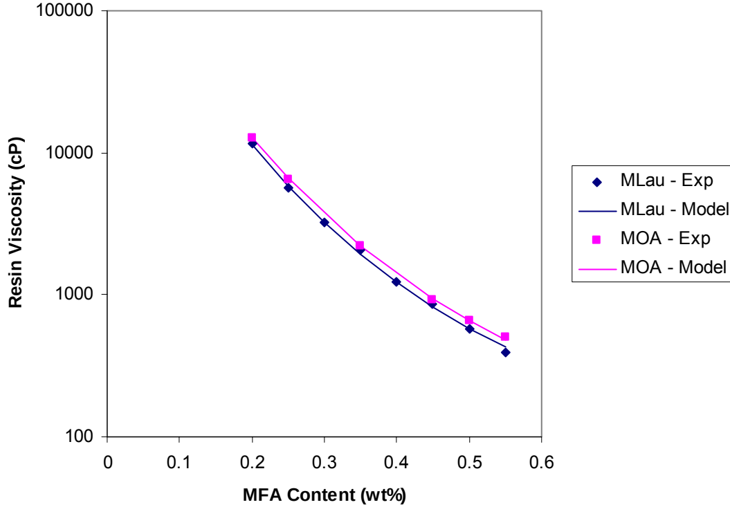
Figure 85. Viscosity of VE resin as a function of MLau content, showing the exponential fit to the data.
