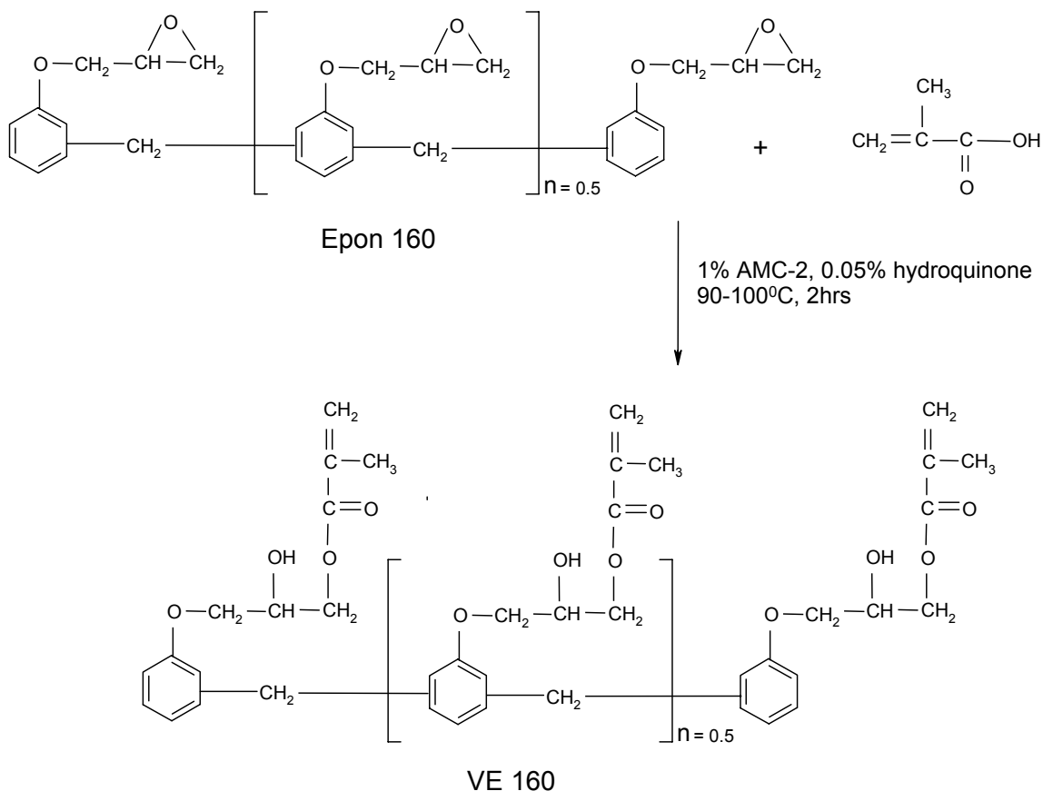
Figure 153. The synthesis of VE 160 from Epon 160 and methacrylic acid.
