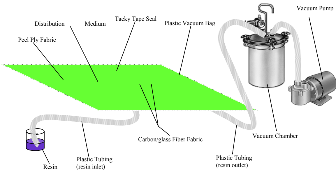
Figure 158. Schematic representation of the VARTM process used to fabricate composites in this work.
