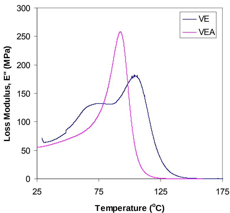
Figure 123. The loss modulus as a function temperature for VE/MLau/Sty and VEA 55/15/30.
