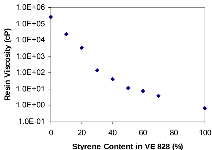
Figure 32. The viscosity of vinyl ester 828 resin as a function of styrene content.
