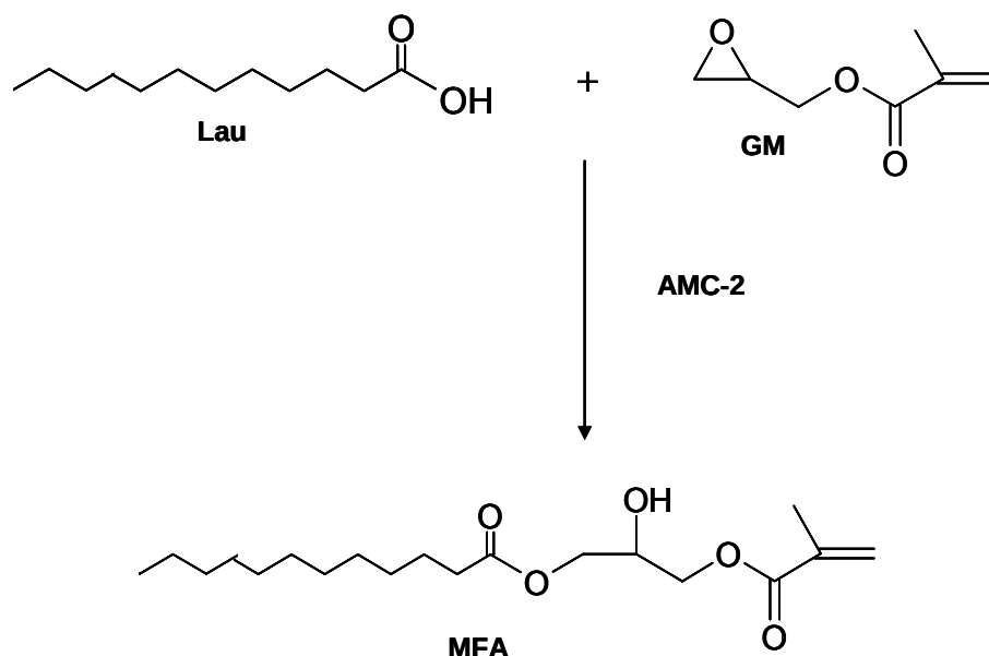
Figure 141. Methacrylated fatty acid synthesized from lauric acid and glycidyl methacrylate with AMC-2 catalyst.
