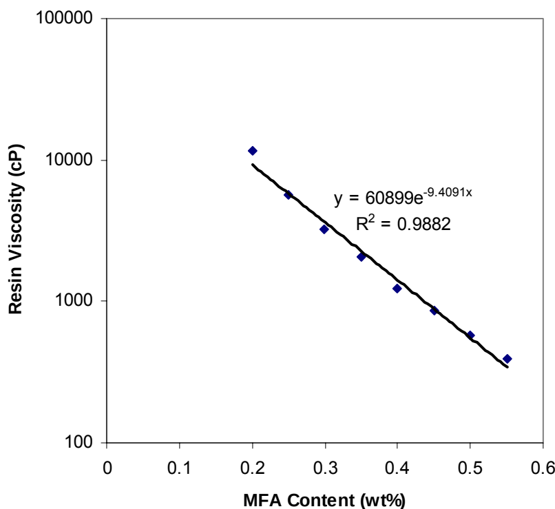
Figure 84. Viscosity of VE resin as a function of MFA content for MLau fatty acids, showing the exponential fit to the data.
