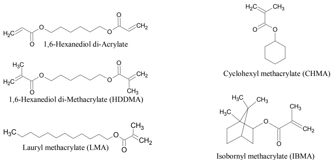
Figure 56. The molecular structure of tested petroleum-derived styrene replacements for VE resins.
