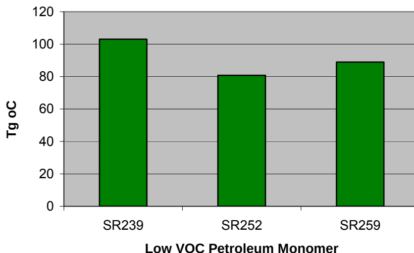
Figure 138. T g as a function of resin formulation for of low VOC di-functional monomers containing 55% CN151, 15% MLau, 10% low VOC petroleum monomer, and 20% styrene.
