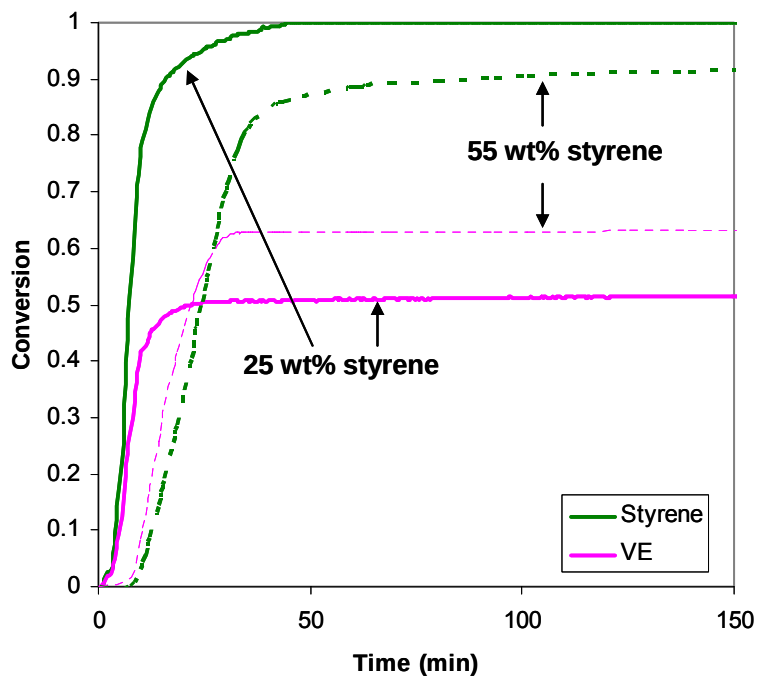
Figure 47. The styrene and VE monomer conversions as a function of cure time at 90°C for VE 828-1007F 65/35 with M_n = 780 g/mol with 25 wt% and 55 wt% styrene.
