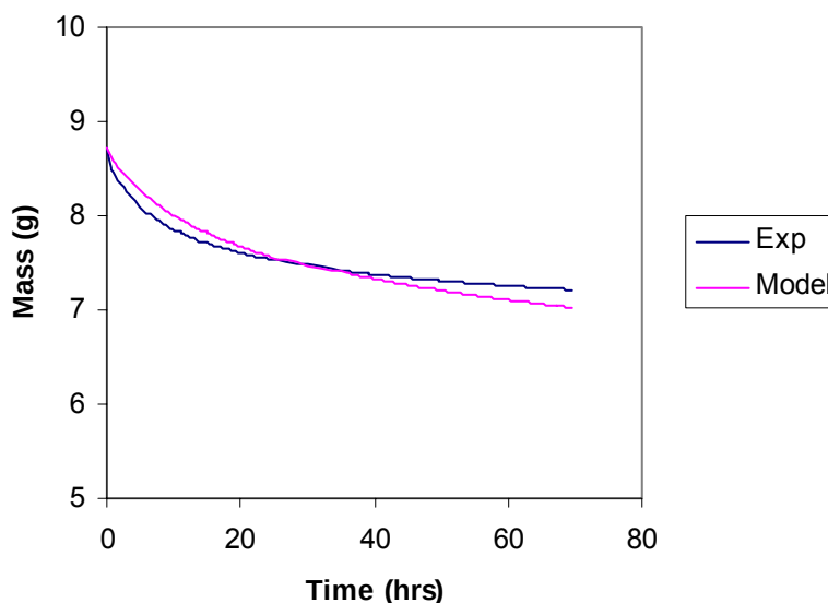
Figure 55. Model vs. experimental emissions profile for VE 828/1004F 43/57 + 30% styrene.
