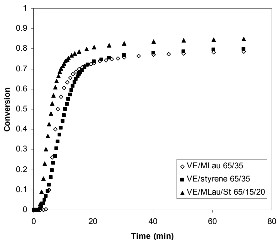
Figure 108. The conversion as a function of time for the cure of VE/MLau/Styrene 65/15/20 relative to VE/MLau 65/35 and VE/styrene 65/35. Samples were cured at 90°C.
