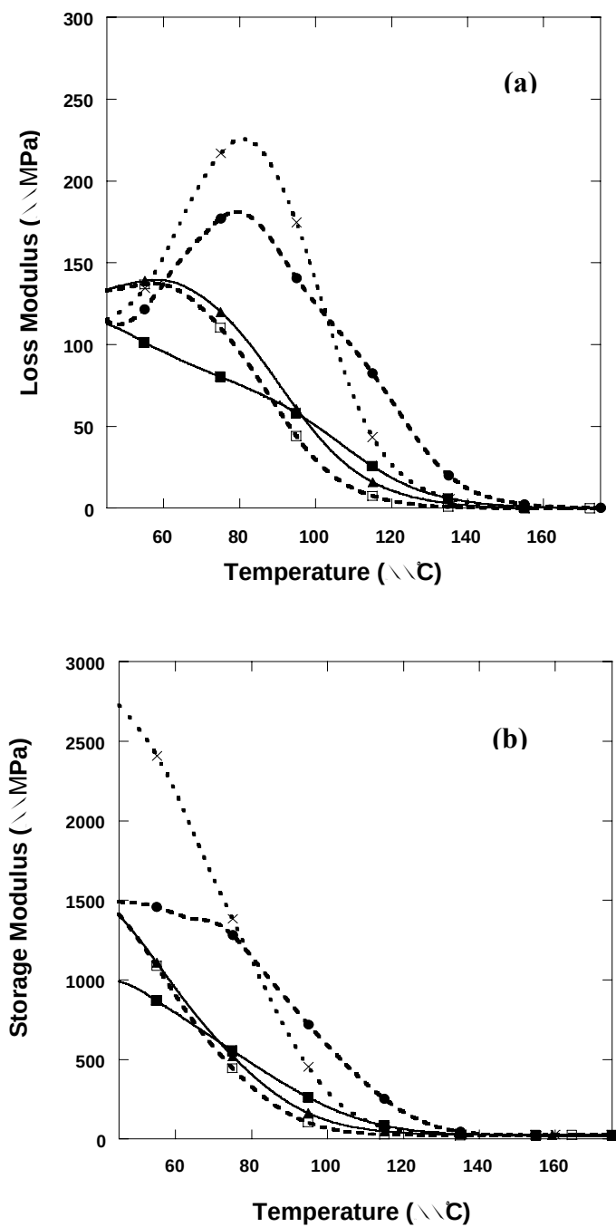
Figure 99. Loss (a) and Storage (b) modulus of 55 wt% VE with 45 wt% MFA. MBut (x), MHex (•), MOct (□), MLau (▲), MMyr(■)
