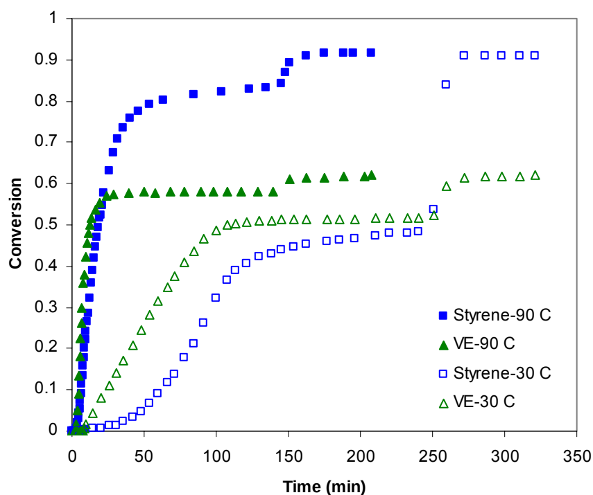
Figure 46. The conversion as a function of time for Derakane 411-350 resins at 30°C and 90°C.
