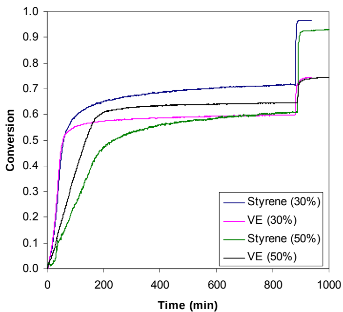
Figure 48. The styrene and VE monomer conversions as a function of cure time at 30°C for monodisperse VE 828 with 30 wt% styrene and 50 wt% styrene.
