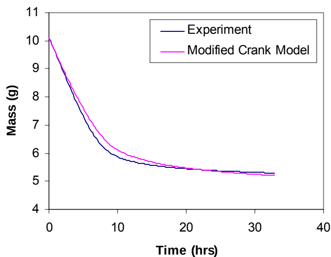
Figure 28. The emission profile from VE/Styrene 50/50 at 60°C as measured experimentally and as predicted from the modified Crank model.
