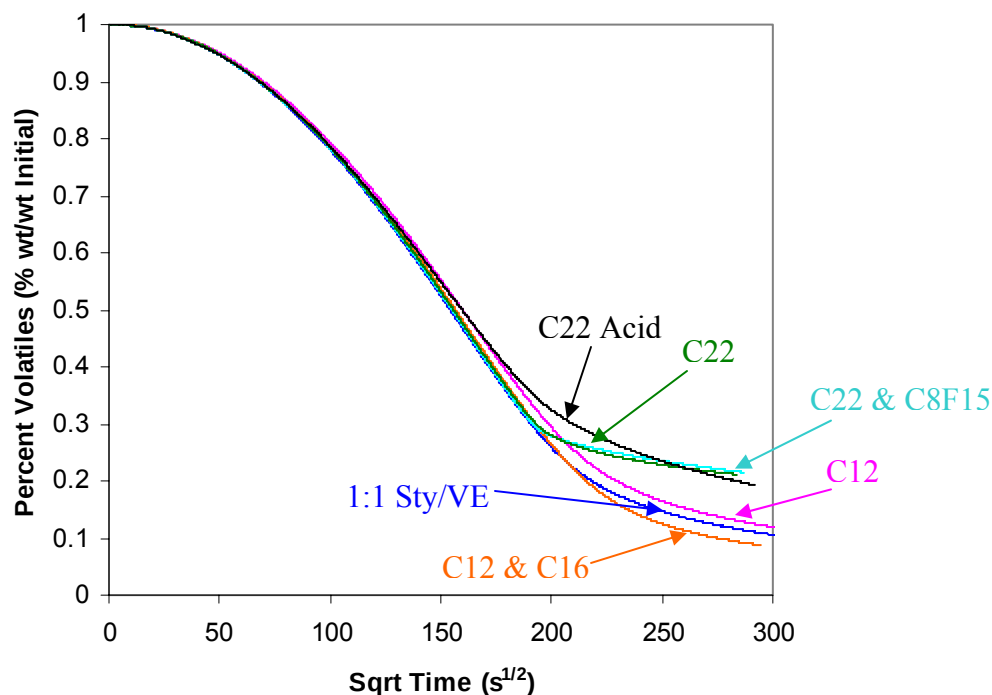
Figure 185. Emissions performance of polyester based suppressant candidates at 2% loading.
