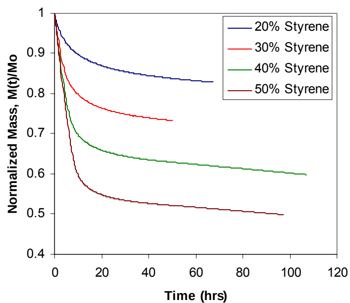
Figure 13. Mass loss of styrene in the VE 828 resin system as a function of time under 40°C isothermal conditions for four different initial styrene contents.
