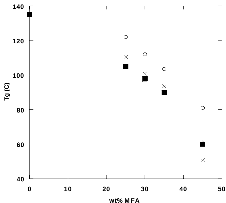
Figure 116. Glass transition temperature ( T_g ) of 55 weight% vinyl ester and 45 weight% of acids with styrene. MBut ternary blends ( \circ ), MHex ternary blends ( \times ), MOct ternary blends ( \Delta ), MLau ternary blends ( \blacksquare ).
