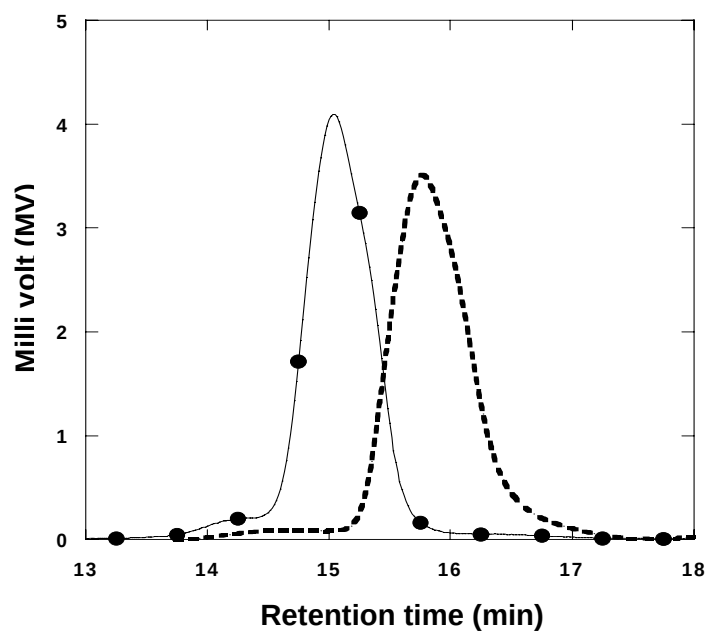
Figure 70. Shift of the peak of the (—) Pure lauric acid to (●) Methacrylated lauric acid.
