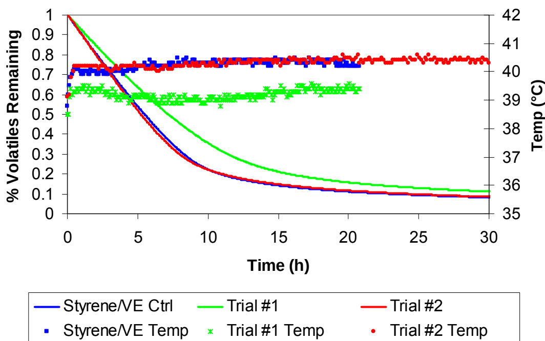
Figure 187. Emissions as a function of time from a VE/Styrene 50/50 resin showing that HB-polypropylene is not an effective suppressant and temperature control is paramount.
