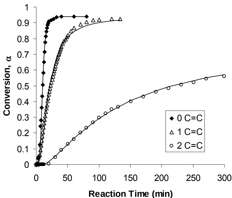
Figure 94. The conversion as a function of time for the homopolymerization at 90°C of MFA with 0, 1, and 2 residual unsaturation sites and their autocatalytic fit.
