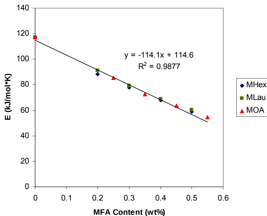
Figure 87. The activation energy as a function of diluent content and fatty acid type.
