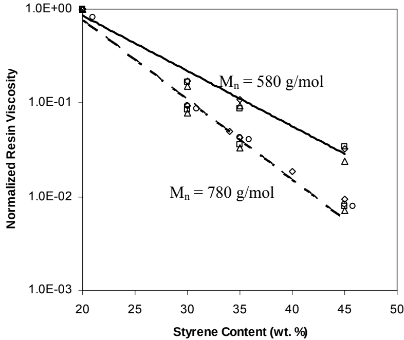
Figure 40. The resin viscosity as a function of styrene content at constant M_n . Styrene content affects the resin viscosity to the same extent for all bimodal resins with the same M_n , and the effect of styrene content on resin viscosity decreases as M_n decreases.
