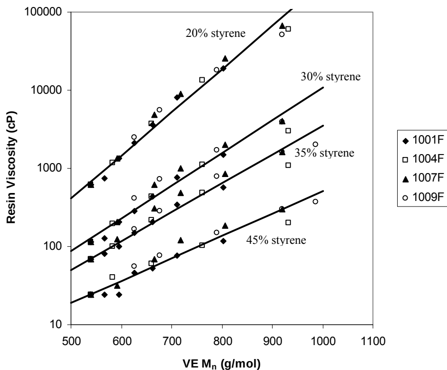
Figure 37. The resin viscosity as a function of VE M_n and styrene content, showing that resin viscosity is normalized by VE M_n .
