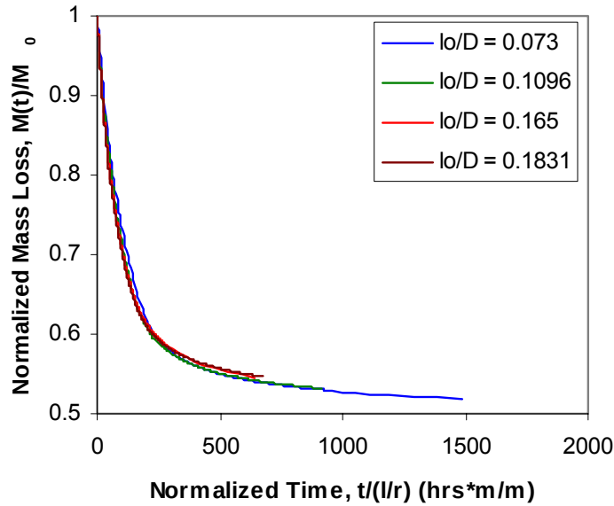
Figure 29. The normalized mass loss as a function of normalized time for different aspect ratios.
