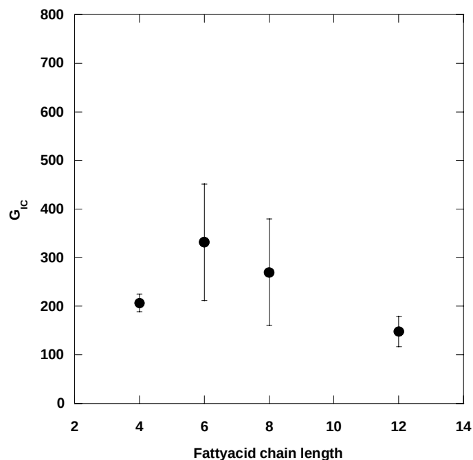
Figure 101. The fracture toughness of the 55%VE/25% MFA/20% Styrene ternary blends at increasing fatty acid chain lengths.
