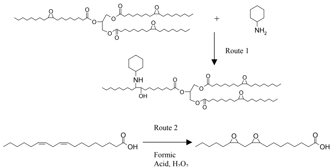
Figure 190. Potential methods of producing AB 2 monomers from triglycerides and fatty acids. In Route 1, epoxidized triglycerides are modified with cyclohexyl amine. In Route 2, linoleic acid is reacted to form epoxidized linoleic acid.
