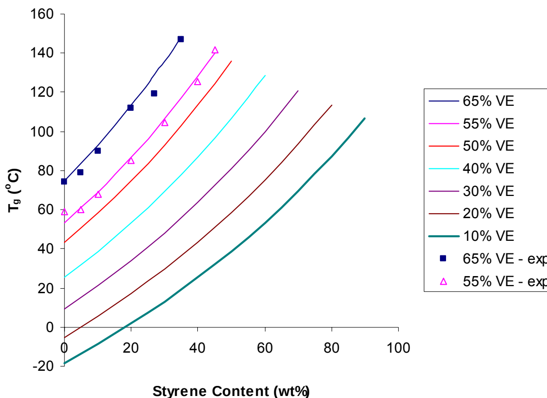
Figure 112. The Fox equation can be used to predict T_g of blends of VE, MLau, and styrene.
