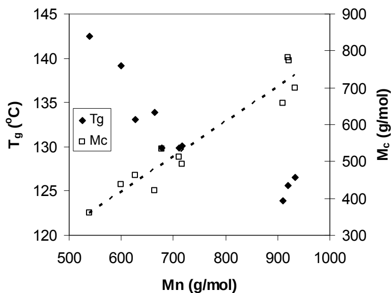
Figure 51. T_g and M_c as a function of M_n of bimodal VE blends with 45 wt.% styrene.
