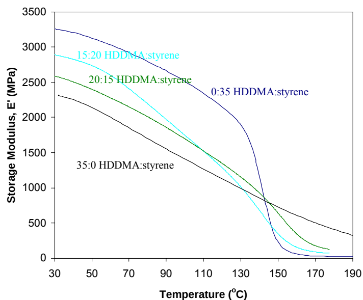
Figure 62. The storage modulus as a function of temperature for VE/HDDMA/styrene blends.
