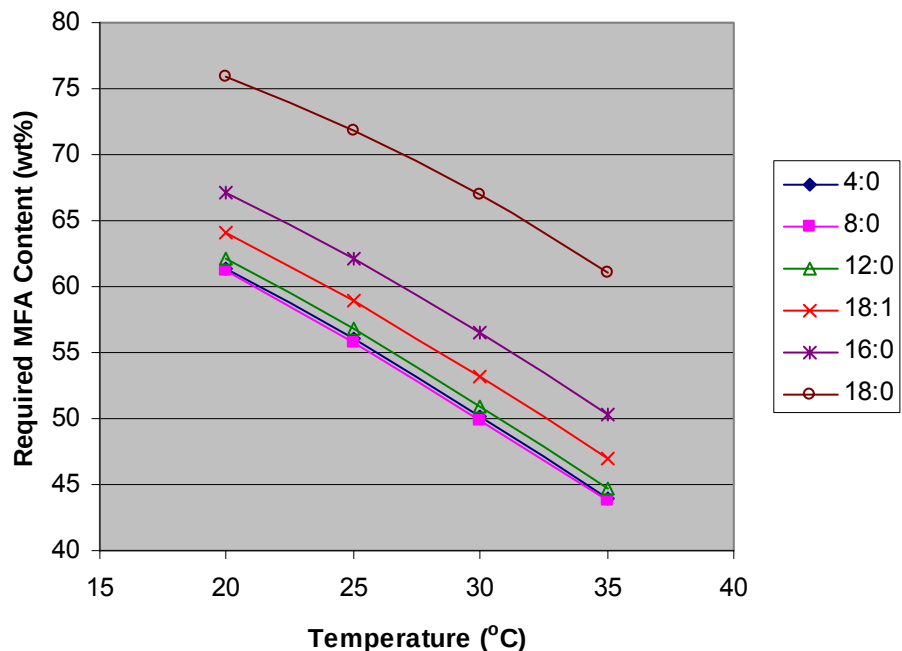
Figure 89. The minimum MFA content required to achieve VE resin viscosities below 500 cP as a function of temperature, fatty acid chain length, and unsaturation level. The operating window is any MFA content above the curve. Legend: [Carbon atoms:Unsaturation sites].
