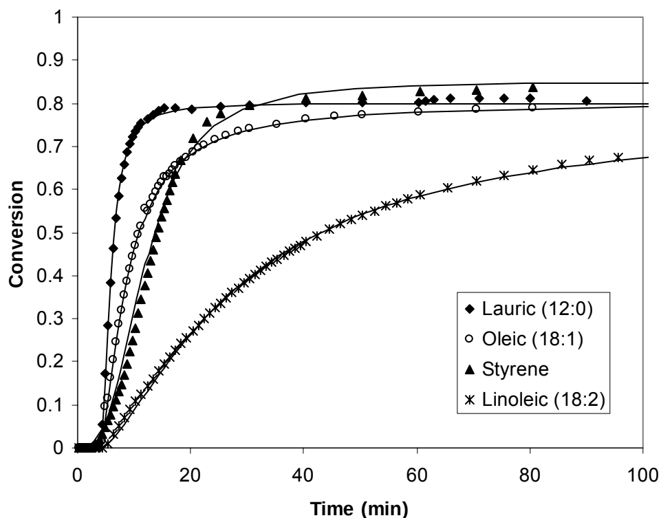
Figure 95. The overall conversion as a function of time for the cure of VE/MFA relative to VE/styrene and their autocatalytic fits using 45% reactive diluent. Samples were cured at 90°C and post-cured at 120°C once the cure reaction stopped.
