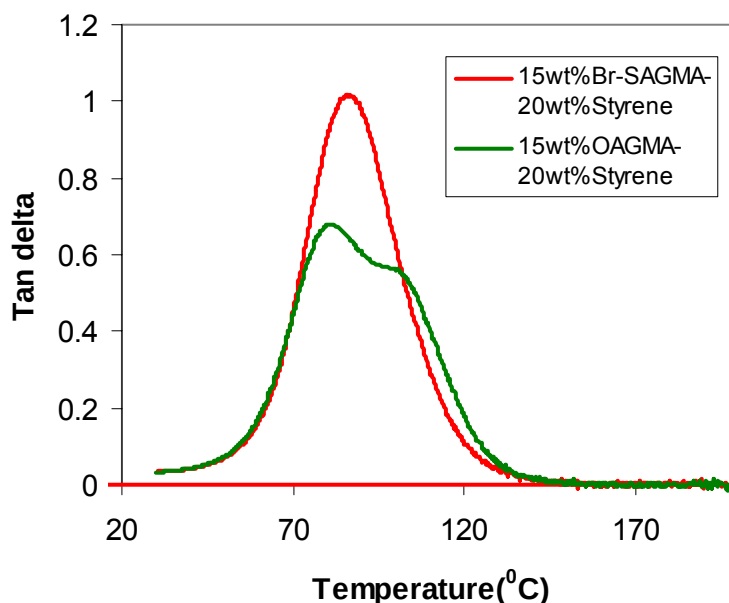
Figure 152. The tan delta curves of Viapal-MOA-Styrene and Viapal-Br-MSA-Styrene Polymers at 15 wt.% fatty acid comonomer content.
