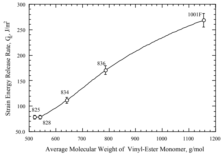
Figure 33. The fracture toughness as a function of VE molecular weight for vinyl esters with 40 wt% styrene.
