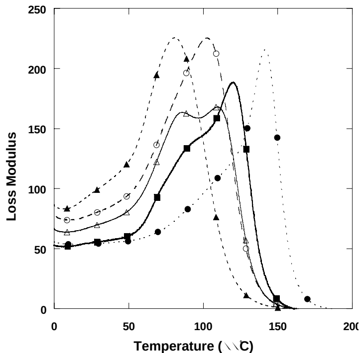
Figure 113. Loss modulus (MPa) behavior of 55 weight% VE and 45 weight% of methacrylated butyric acid and styrene combination. 45 wt% MBut (▲), 35 wt% MBut & 10 wt% Styrene (○), 30 wt% MBut 15 wt% Styrene (Δ), 25 wt% MBut & 20 wt% Styrene (■), 45 wt% Styrene (●).
