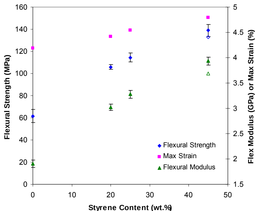
Figure 117. The flexural properties as a function of styrene content for resins containing 55% VE and using MLau and styrene as the reactive diluent. The open points show the results for Derakane 411-350.
