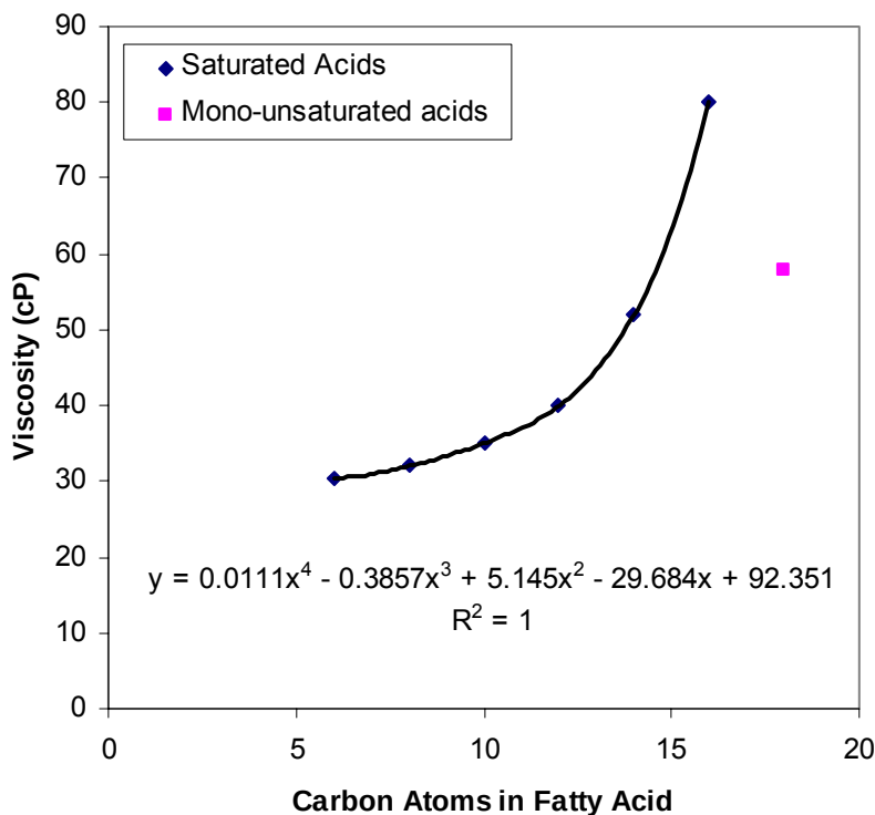
Figure 76. Viscosity of MFA monomers as a function of fatty acid chain length.
