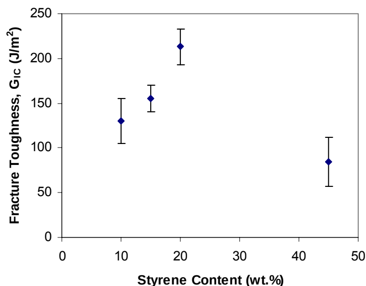
Figure 102. The fracture toughness of VE/MBut/Styrene ternary blends containing 55% VE as a function of styrene content.
