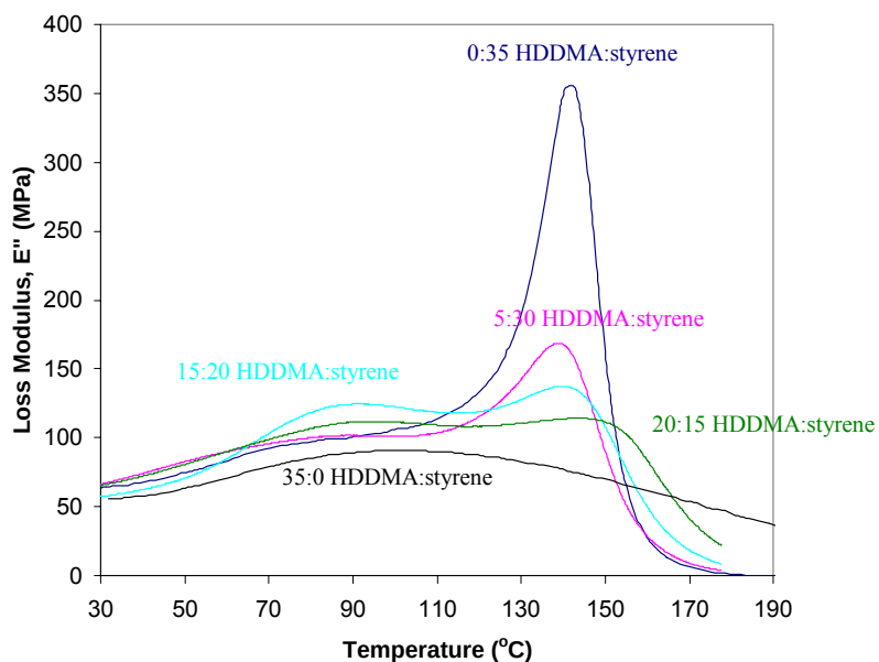
Figure 63. The loss modulus as a function of temperature for VE/HDDMA/styrene blends.
