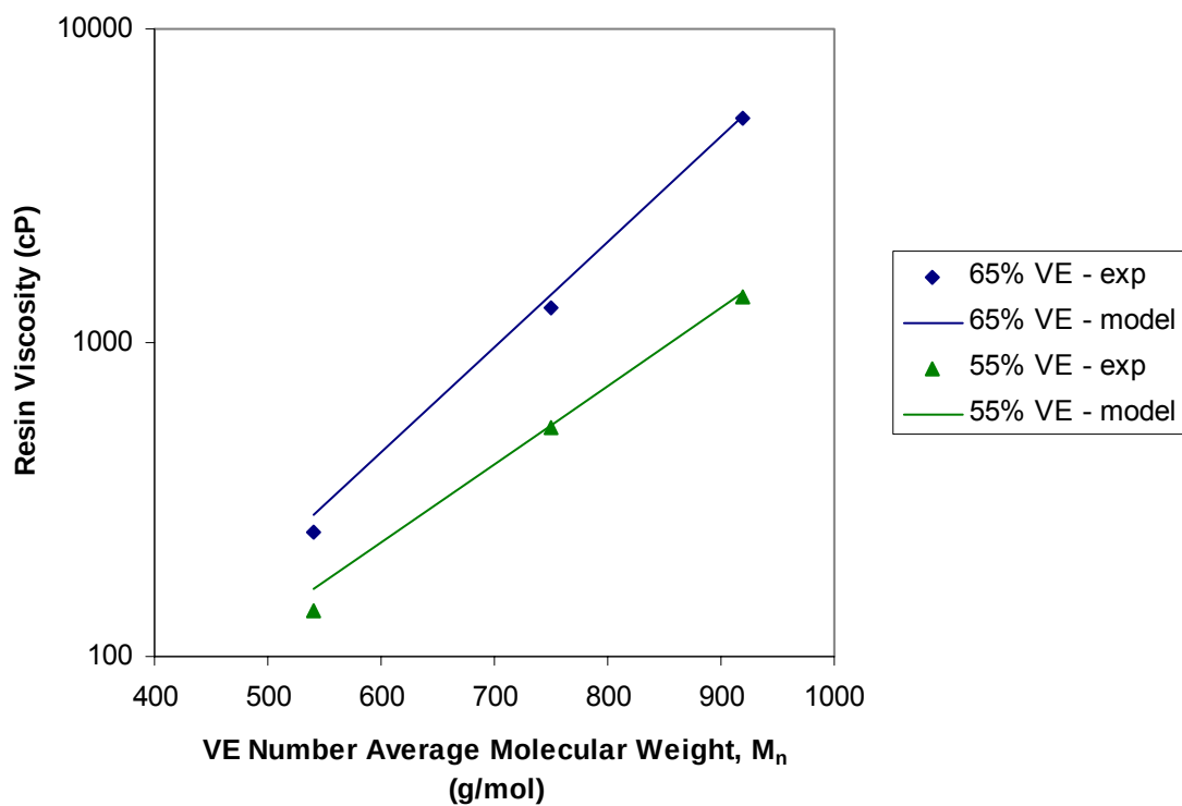
Figure 91. The experimental and model viscosities of VE/MHex/Styrene as a function of VE molecular weight and VE content for resins containing 20 wt% styrene.
