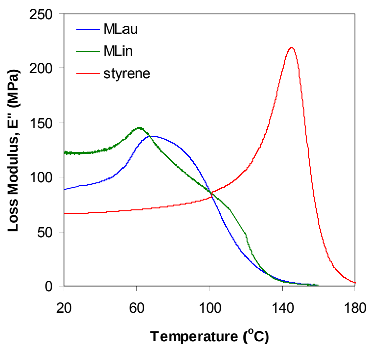
Figure 120. The loss modulus as a function of temperature for MLau, MLin, and styrene based vinyl esters using 35% reactive diluent.
