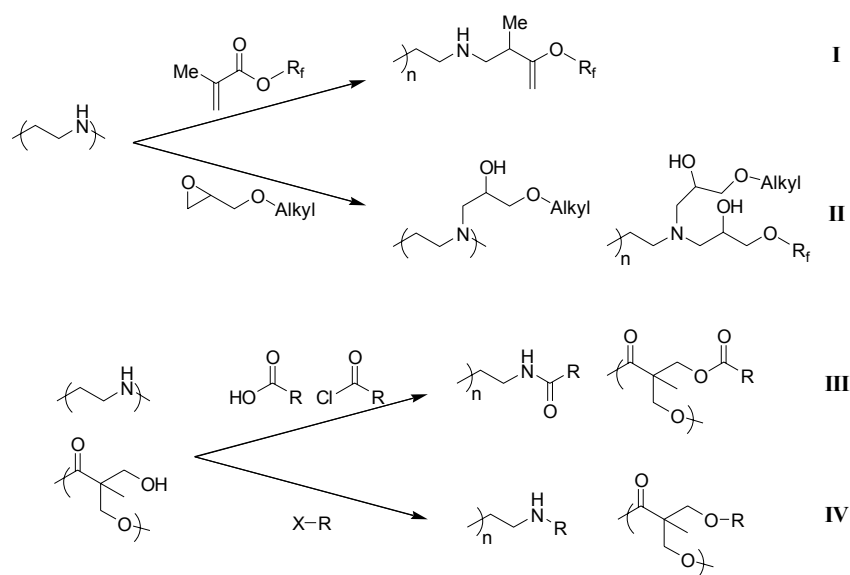
Figure 179. Potential methods of end-group modification. Routes I (Michael addition) and II (epoxide opening) are more suited to the PEI end-groups, while routes III (acyl condensation) and IV (halide displacement) should be applicable to either system.
