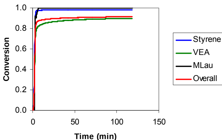
Figure 126. The component and overall cure of VEA/MFA/Styrene 65/15/20.
