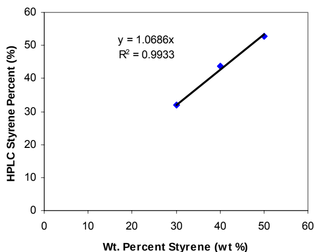
Figure 8. Calibration curve relating styrene content measured using SEC to the actual styrene content in the sample.
