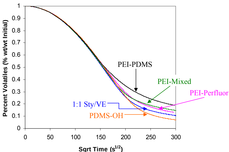
Figure 184. PEI-based suppressant candidates
