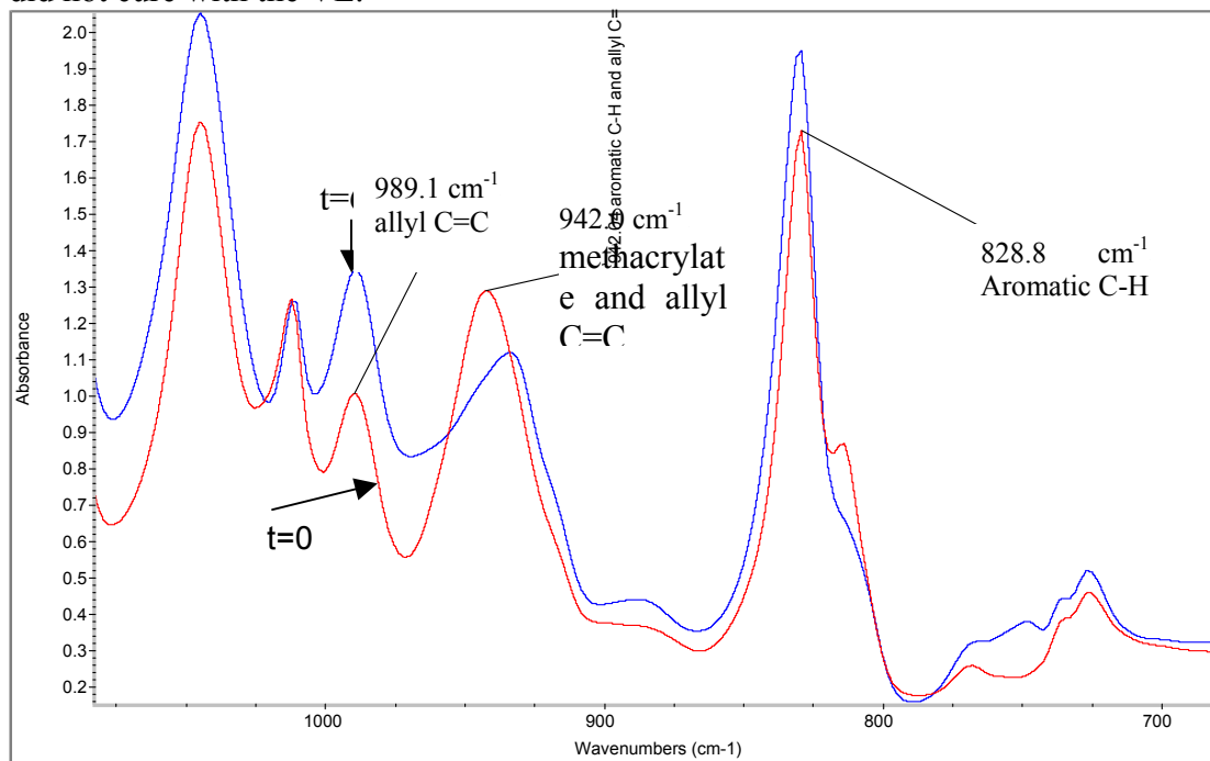
Figure 77. The FTIR spectra of VE/AOH-SBO with CoNap at t=0 and t=6 days.
