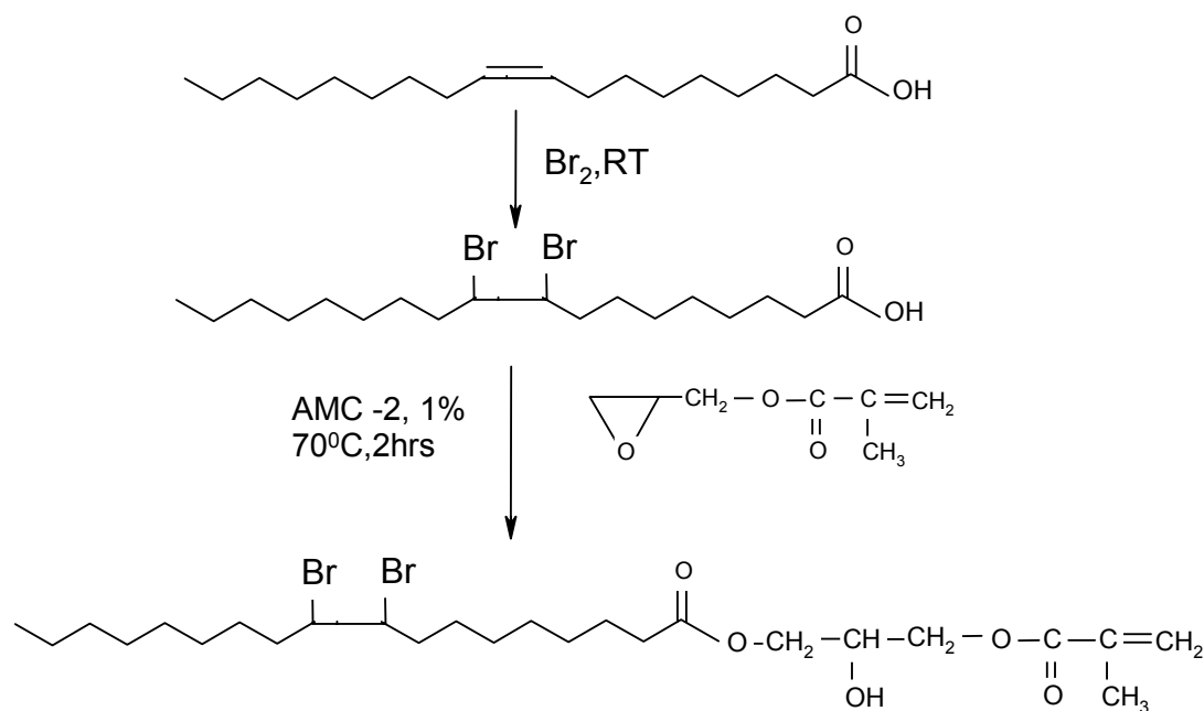
Figure 72. The reaction scheme for the synthesis of 9-10 di-bromo stearic acid glycidyl methacrylate (Di-Br MSA) from oleic acid.
