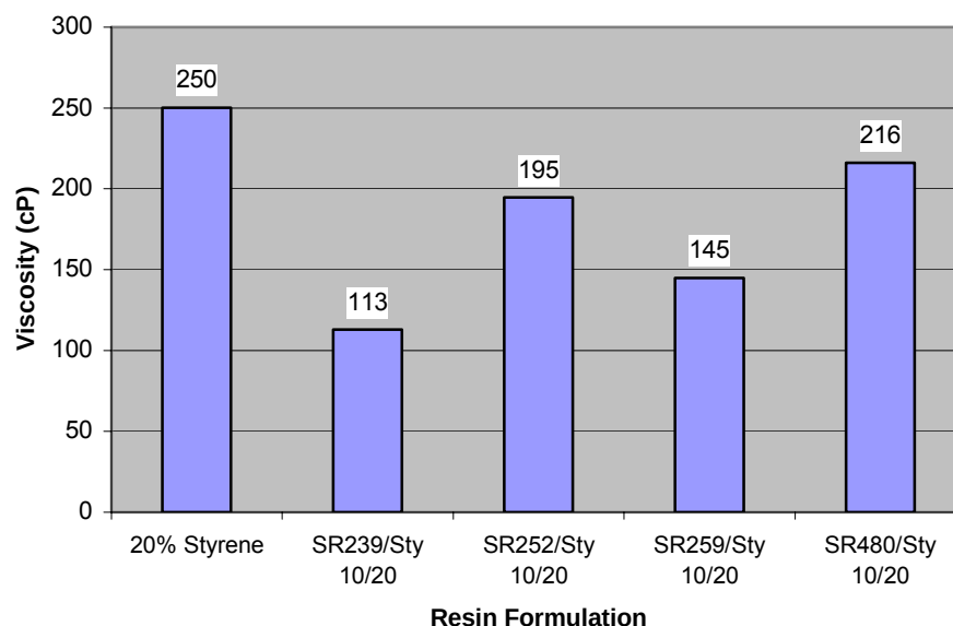
Figure 133. Viscosity as a function of di-functional resin formulation for resins with 55% CN151.
