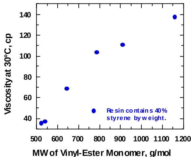
Figure 31. The viscosity of vinyl ester resins as a function of the molecular weight of the VE monomer.
