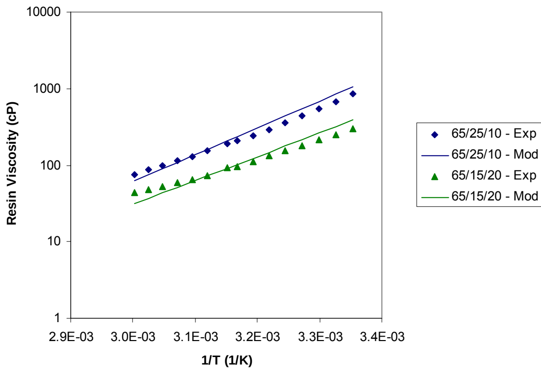
Figure 92. The experimental and model viscosities of VE/MLau/Styrene as a function of temperature.
