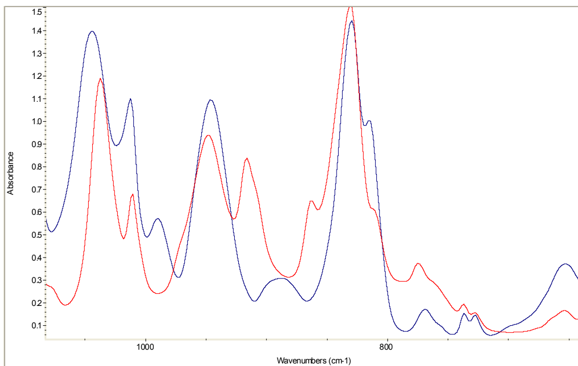
Figure 5. The FTIR spectra of Epon/methacrylic acid and the resulting vinyl ester formed after complete reaction.
