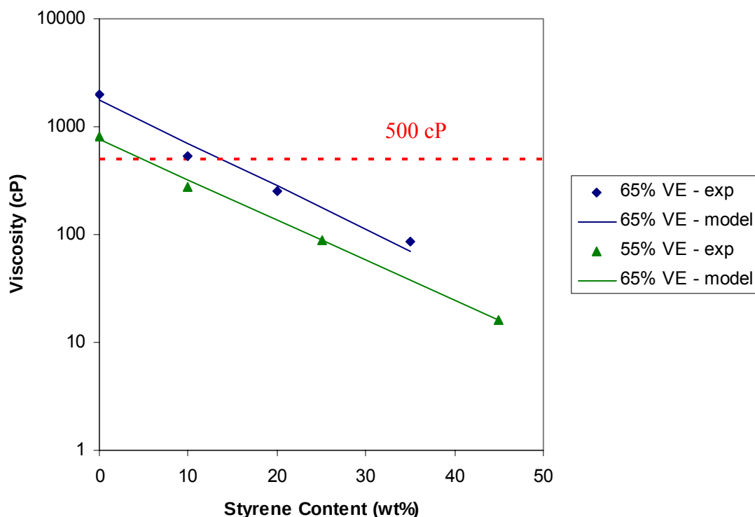
Figure 90. The viscosity of VE/MHex/styrene as a function of styrene content in the resin for resins containing 55 wt% and 65 wt% VE 828, along with model predictions.
