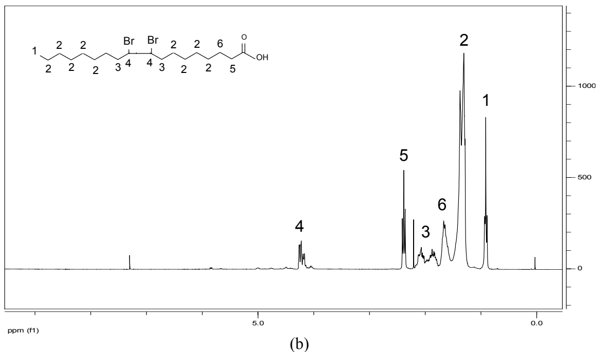
Figure 73. The ^1\text{H} -NMR spectra of (a) oleic acid (b) 9,10 di-bromo stearic acid(Di-BrSA).
