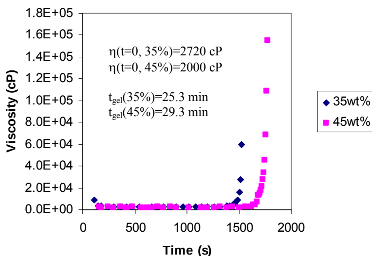
Figure 82. The viscosity of VE/GM-OA resins as a function of cure time.
