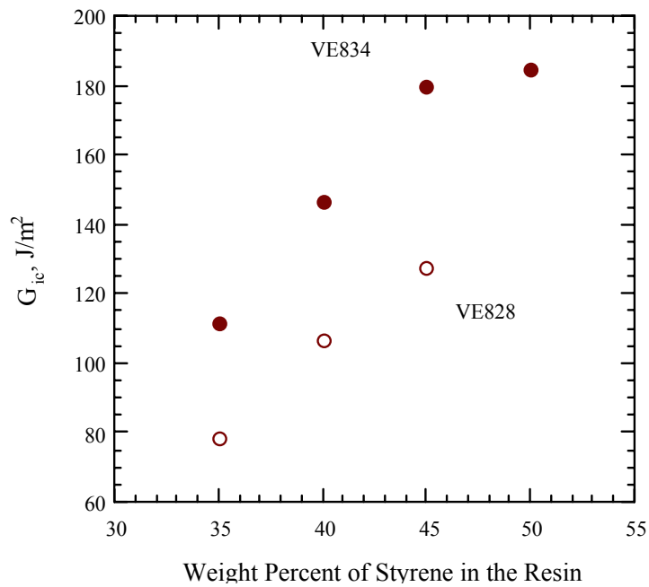
Figure 34. The fracture toughness as a function of styrene content for VE 834 and VE 828.
