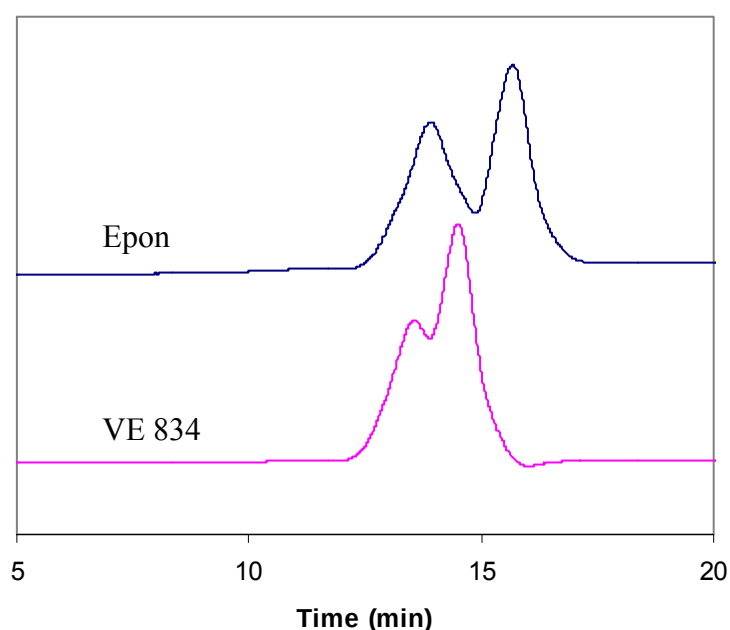
Figure 6. The SEC traces for Epon 834 and VE 834.
