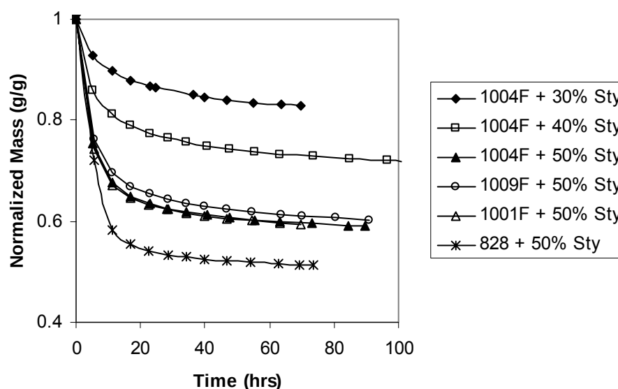
Figure 53. Total styrene emission curve for bimodal vinyl ester systems.
