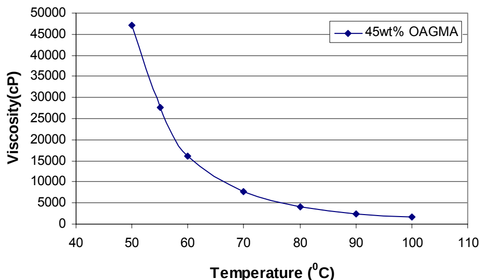
Figure 147. The viscosity of the of the 45 wt.% MOA-55 wt.% UP resin as a function of temperature.
