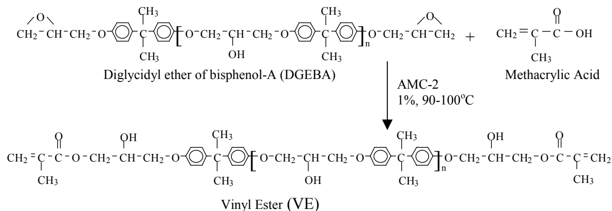
Figure 4. The reaction of methacrylic acid with Epon to form vinyl ester monomer.
