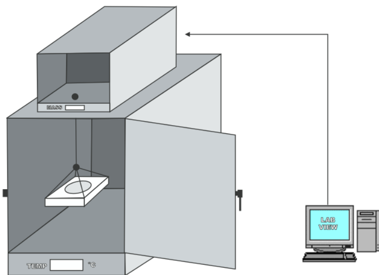
Figure 11. Emissions measurement setup used to measure VOC mass loss as a function of time and temperature.
