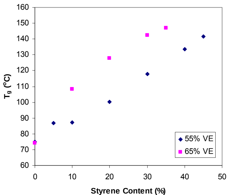
Figure 111. T g as a function of styrene content for VE/MOA/styrene blends.
