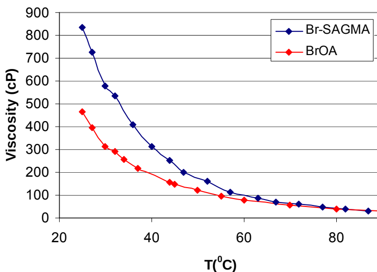
Figure 75. The viscosities of the Di-BrOA and Di-BrMSA as a function of temperature.
