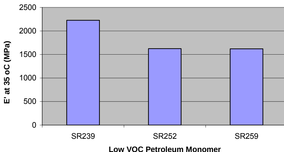
Figure 137. Modulus as a function of low VOC di-functional monomer for resins containing 55% CN151, 15% MLau, 10% low VOC petroleum monomer, and 20% styrene.
