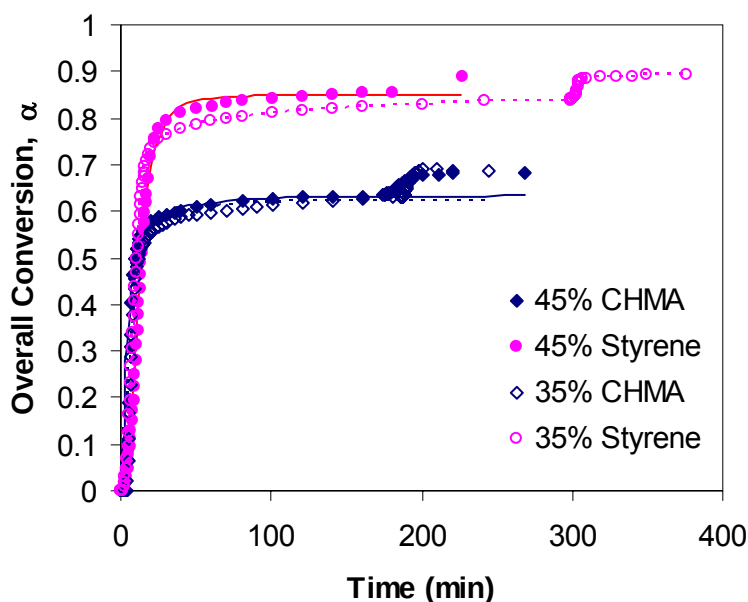
Figure 61. The overall conversion as a function of time for CHMA-based vinyl esters relative to styrene-based vinyl esters.
