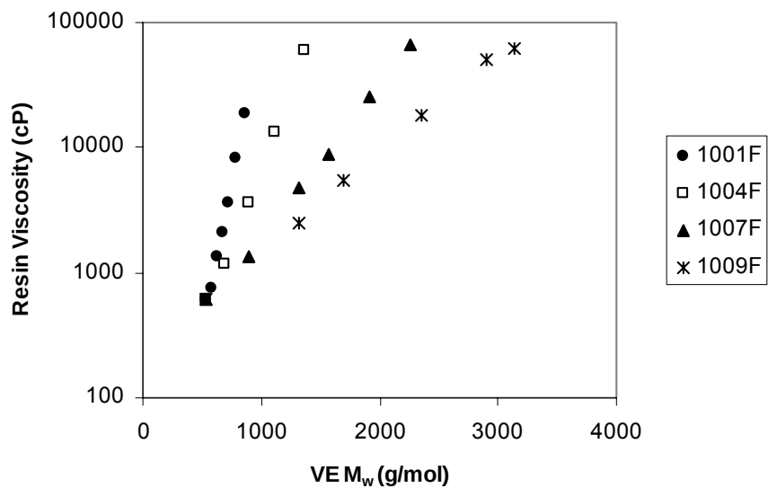
Figure 38. The resin viscosity as a function of VE M_w for resins containing 20 wt.% styrene, showing that resin viscosity is not normalized by VE M_w .
