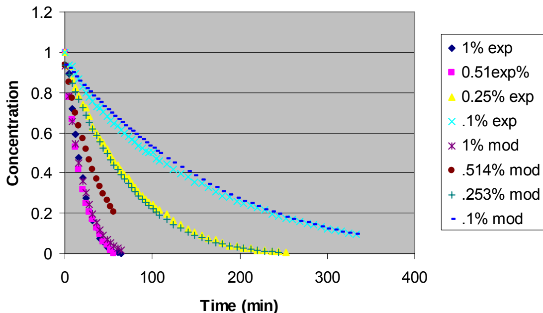
Figure 146. Plot showing a change in concentration [E] as a function of time for both model and experimental data at varying [C] for data obtained at 80°C.
