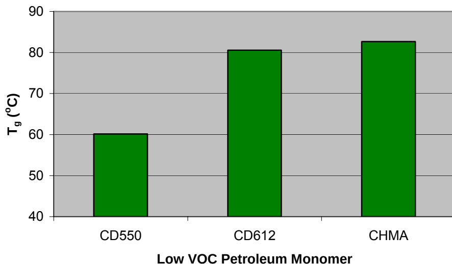
Figure 136. T g as a function of low VOC mono-functional monomers for resins with 55% CN151, 15% MLau, 10% low VOC petroleum monomer, and 15% Styrene.
