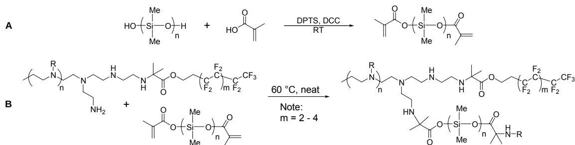
Figure 181. Preparation of PEI-PDMS suppressants.
