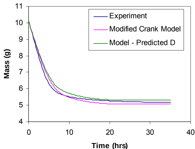
Figure 30. Model predictions vs. experimental results for styrene emissions from VE/styrene 50/50 at 60°C for an aspect ratio of l_0/D of 0.037.
