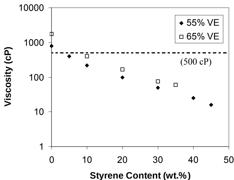
Figure 106. The viscosity of VE/MLau/styrene as a function of styrene content in the resin for resins containing 55 wt% and 65 wt% VE 828.
