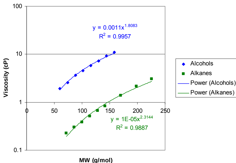
Figure 39. The bulk viscosities of C5-C16 alkanes and alcohols at 25°C dependence on molecular weight [26].
