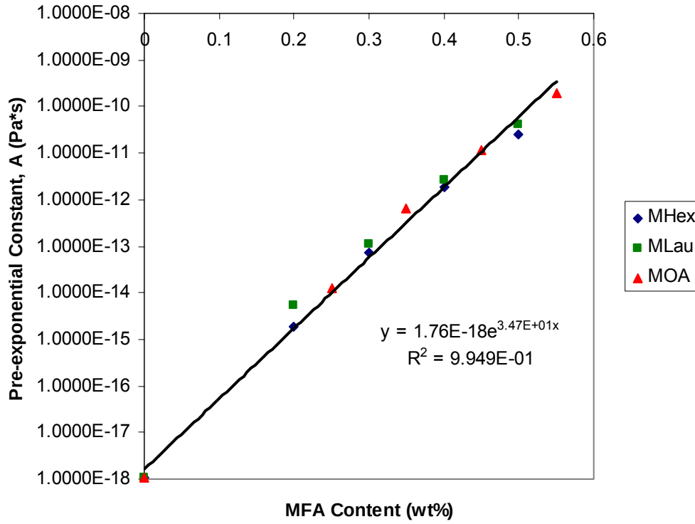
Figure 88. The pre-exponential constant as a function of diluent content and fatty acid type.
