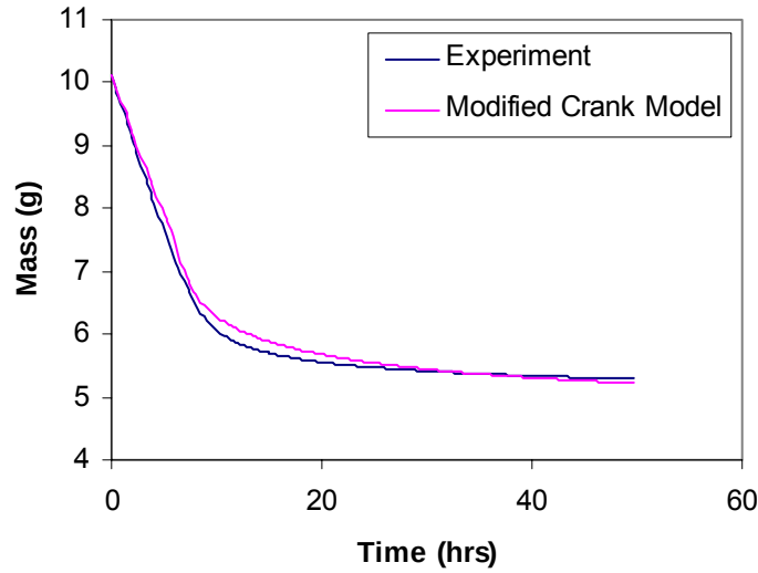
Figure 25. The length-scale modified Crank model accurately models the diffusion regime, as shown for VE 828/Styrene 50/50 at 40°C isothermal conditions.
