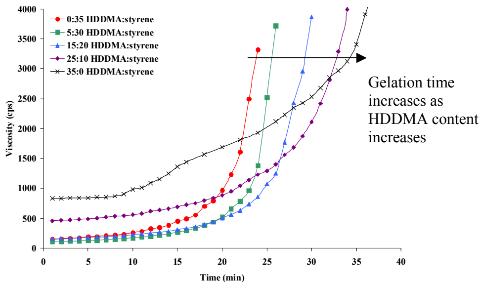
Figure 60. The viscosity as a function of gel time for VE/HDDMA/styrene blends at 30°C.
