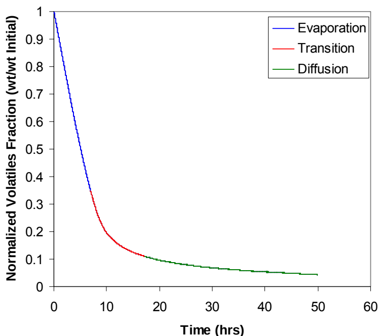
Figure 19. Styrene emission curve for a generalized VE resin system showing the three different regions.
