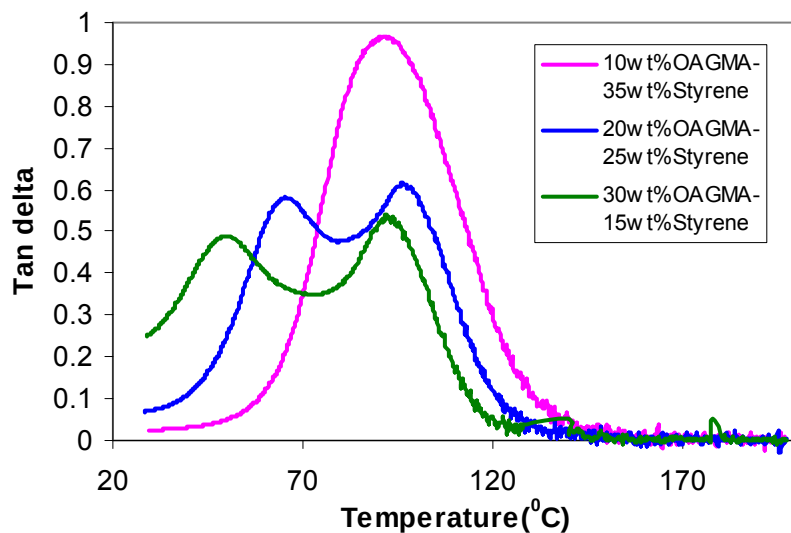
Figure 149. The tan delta curves of Viapal-MOA-Styrene polymers at 10-30 wt.% MOA content. (45 wt.% total comonomer content)
