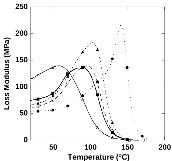
Figure 113. Loss modulus (MPa) behavior of 55 weight% VE and 45 weight% of methacrylated butyric acid and styrene combination. 45 wt% MBut (▲), 35 wt% MBut & 10 wt% Styrene (○), 30 wt% MBut 15 wt% Styrene (Δ), 25 wt% MBut & 20 wt% Styrene (■), 45 wt% Styrene (●).
