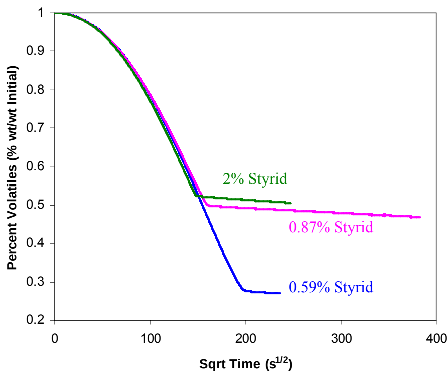
Figure 183. VOC Suppression as a function of Styrid concentration in 1:1 styrene-VE formulation.
