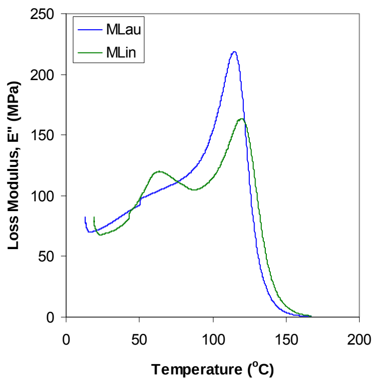
Figure 121. The loss modulus as a function of temperature for ternary blends of VE/MLau/Styrene and VE/MLin/Styrene with weight ratios of 65/15/20.
