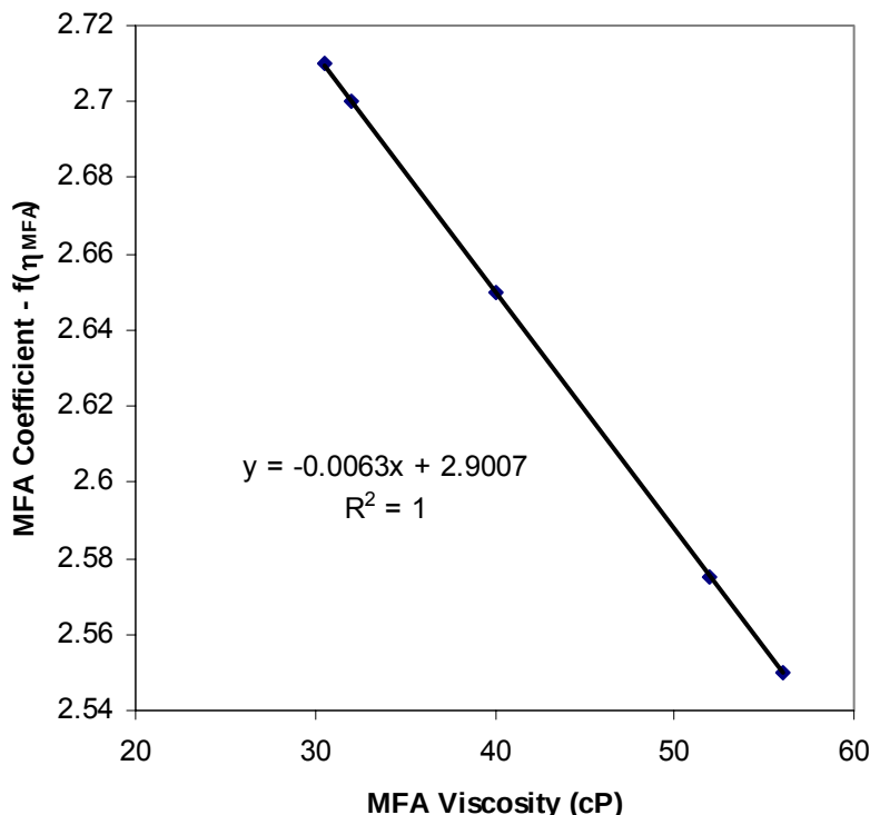
Figure 86. The MFA coefficient in Eq. 18 is a linear function of MFA viscosity.
