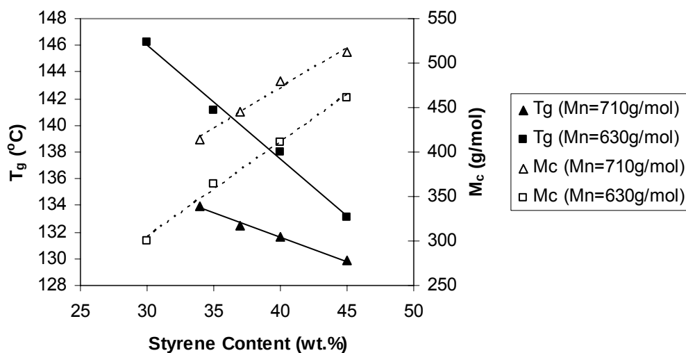
Figure 52. T_g and M_c as a function of styrene content for bimodal VE 828/1001F 48/52 ( M_n = 710 g/mol) and VE 828/1009F 84.9/15.1 ( M_n = 630 g/mol).
