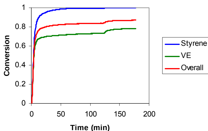
Figure 127. Component and overall cure of VE/MFA/Styrene 65/15/20.
