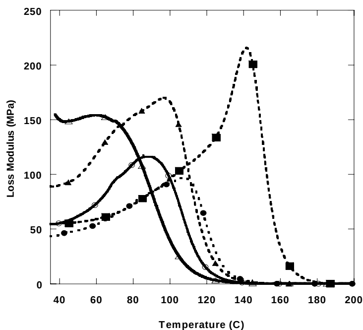
Figure 115. Loss modulus (MPa) behavior of 55 weight% VE and 45 weight% of methacrylated caproic acid and styrene combination. 45 wt% MHex ( \Delta ), 35 wt% MHex & 10 wt% Styrene ( \blacktriangle ), 30 wt% MHex 15 wt% Styrene ( \circ ), 25 wt% MHex & 20 wt% Styrene ( \bullet ), 45 wt% Styrene ( \blacksquare )
