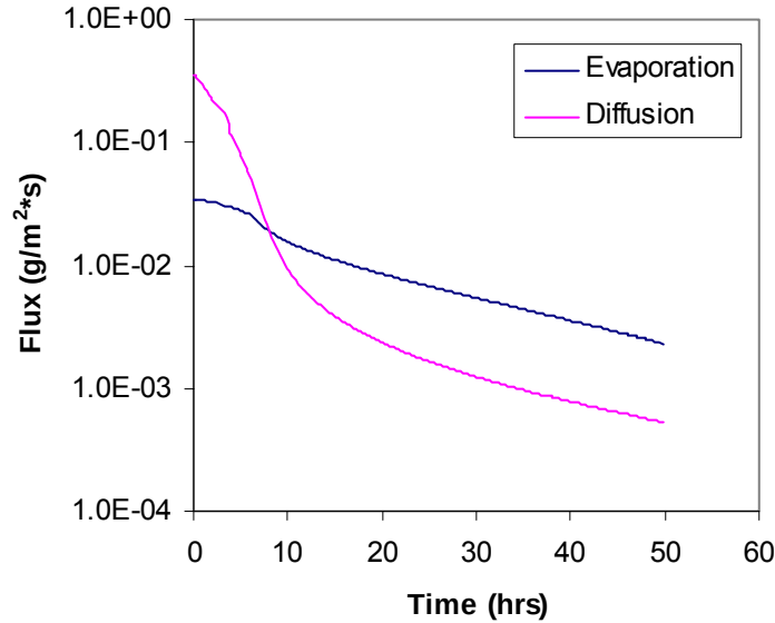
Figure 22. Plot of evaporation flux and diffusion flux for VE 828/Styrene 50/50 as a function of time under 40°C isothermal conditions for finding the cross-over point.
