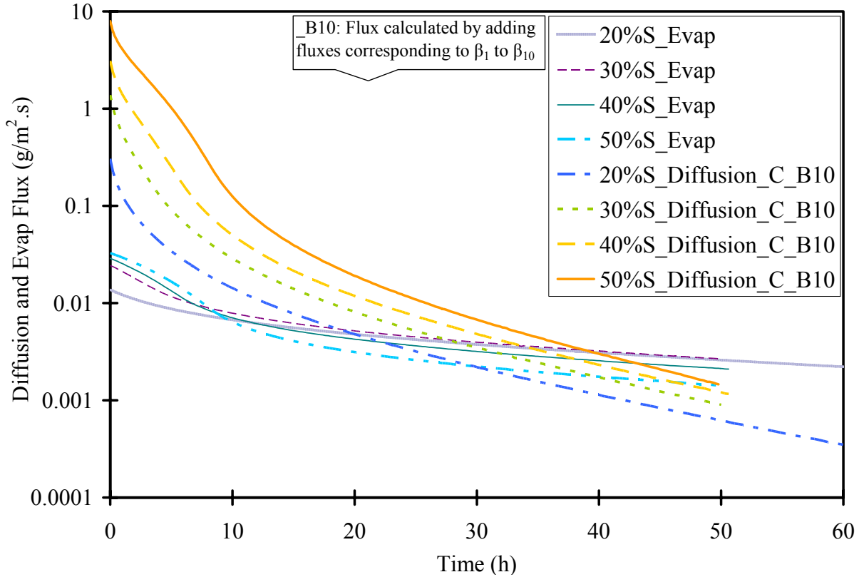
Figure 23. Plot of evaporation flux and diffusion flux with time for finding cross-over point (for \beta_{10} ) in the study of styrene variation of VE 828 resin system under 40°C isothermal conditions. Suffix ‘_Evap’ designates the curves corresponding to evaporation flux. Suffix ‘_Diffusion_C_B10’ designates the curves corresponding to diffusion flux obtained by considering first ten terms ( \beta_1 through \beta_{10} ) of the expansion series.
