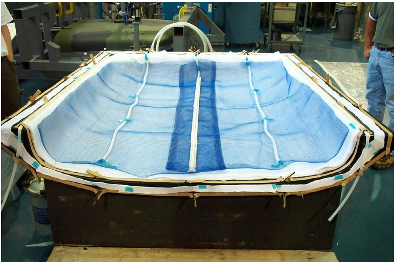
Figure 171: The composite hood lay-up showing the three inlet lines and two vacuum lines.
