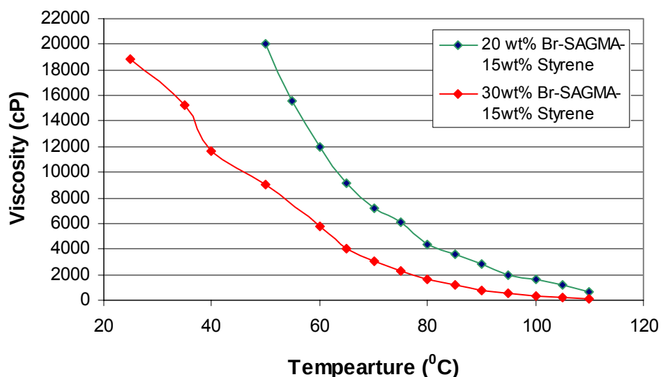
Figure 148. The viscosity of the of the 20 wt.% Br-MSA-15wt% Styrene-55wt% UPE resin and the 30 wt.% Br-MSA-15wt% Styrene-55wt% UP Eas a function of temperature.
