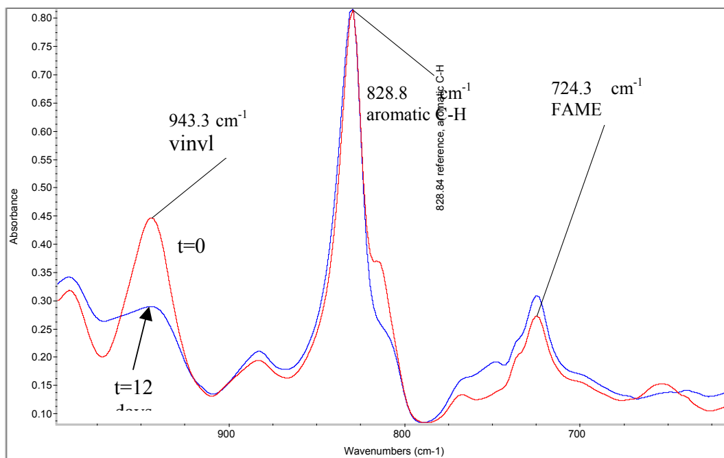
Figure 79. The FTIR spectra at t=0 and t=12 days for the induced cure of VE in the presence of FAME and CoNap.
