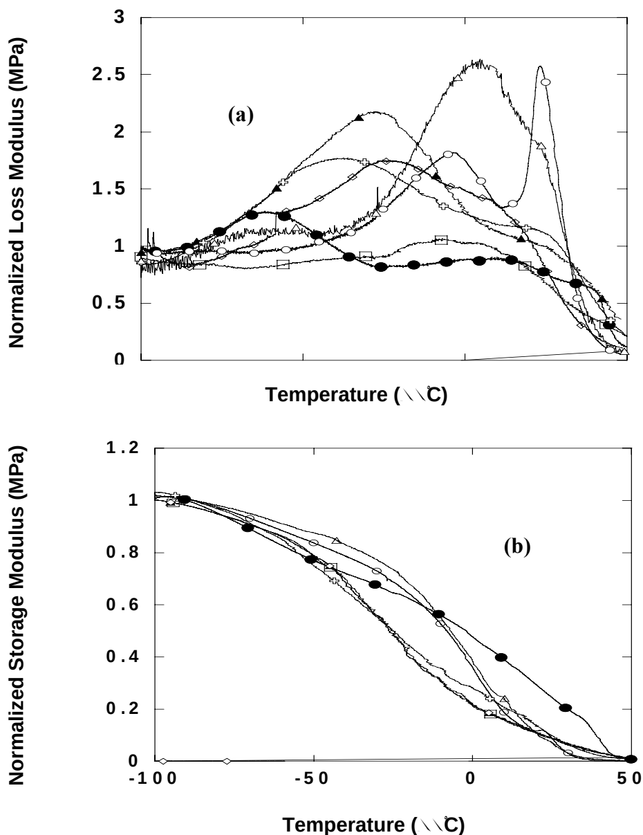
Figure 97. Normalized Loss (a) and storage modulus (b) behavior of Methacrylated Fatty Acids (MFA) as a function of fatty acid chain length. Methacrylated Palmitic acid (●), Methacrylated Myristic acid (□), Methacrylated Lauric acid (▲), Methacrylated Decanoic acid (⊕), Methacrylated Octanoic acid (◇), Methacrylated Hexanoic acid (Δ), Methacrylated Butyric acid (O).
