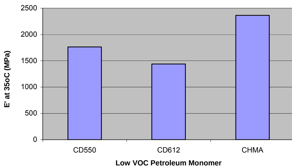
Figure 135. Storage modulus as a function of mono-functional monomers for resins with 55% CN151, 15% MLau, 10% low VOC petroleum monomer, and 15% Styrene.
