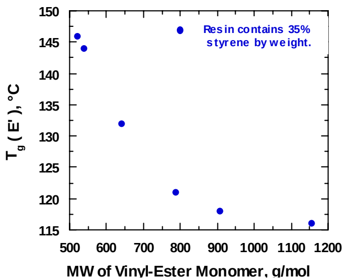
Figure 35. T_g as a function of vinyl ester molecular weight for samples with 35% styrene.
