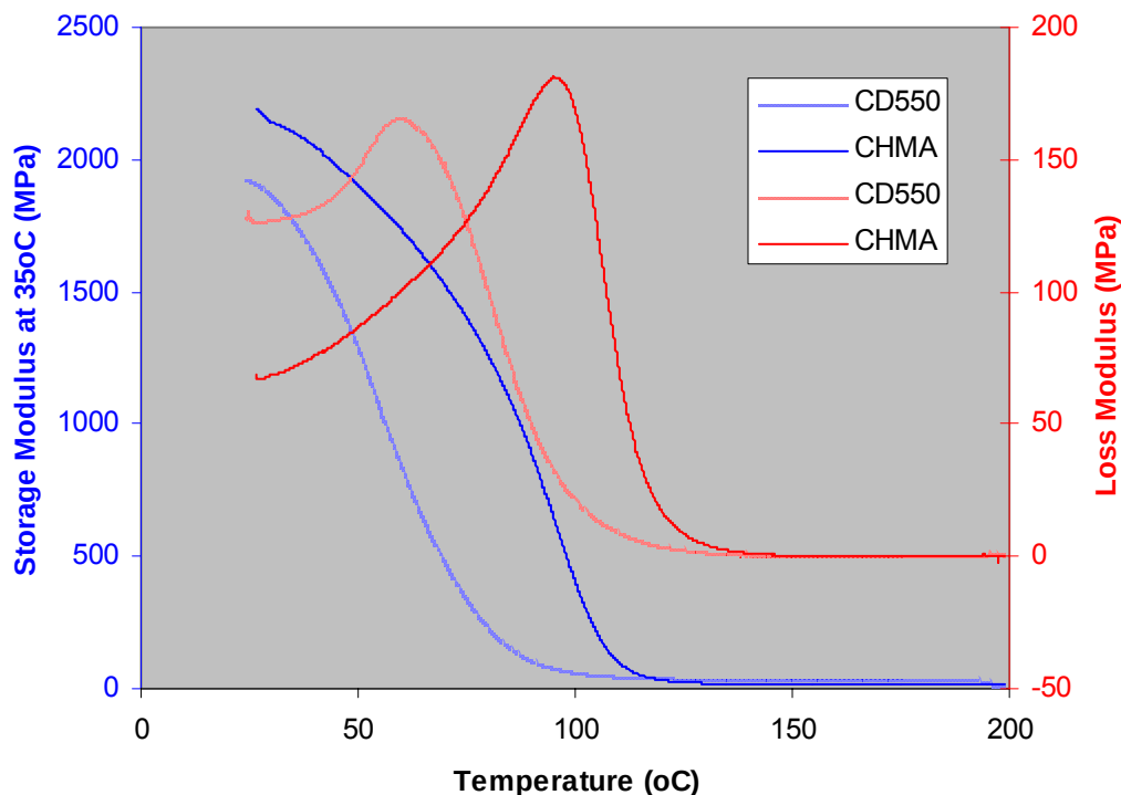
Figure 134. The storage modulus and loss modulus as a function of temperature for VE/MLau/Styrene/CHMA 55/15/15/15 and VE/MLau/Styrene/CD550.
