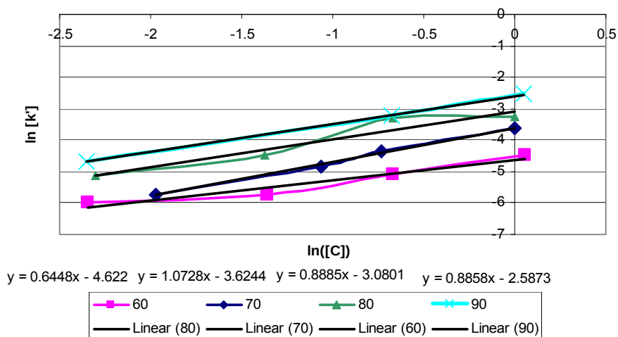
Figure 143. Plot of \ln[k'] versus \ln[C] for the four temperatures investigated.
