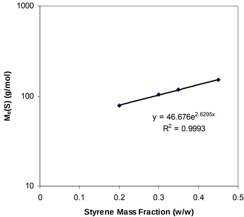
Figure 41. The dependence of M_e(S) on the styrene weight fraction in bimodal blends of VE resins.
