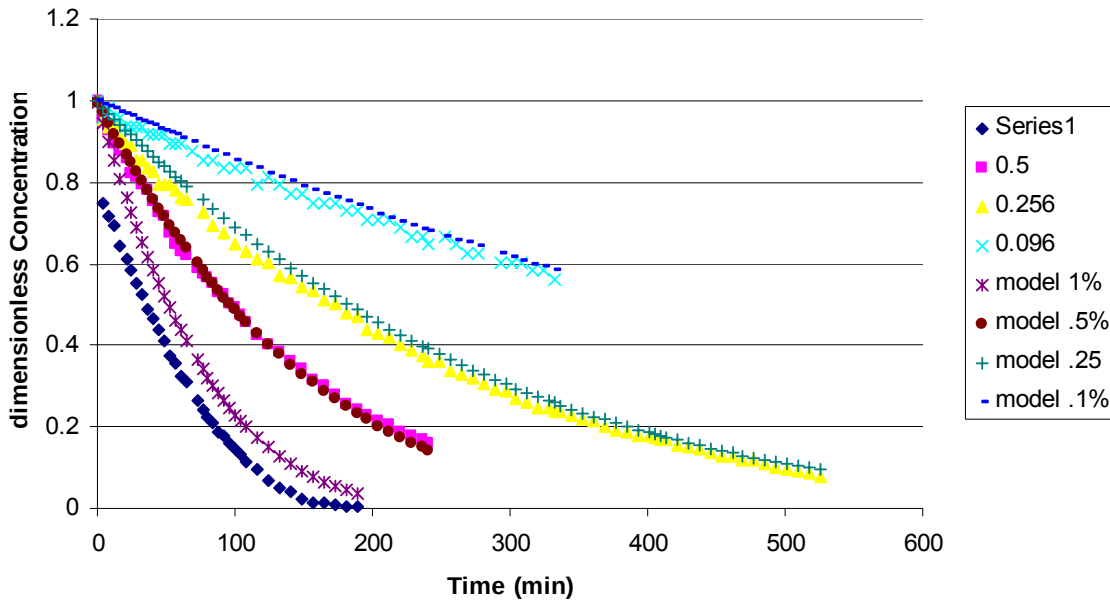
Figure 145. Plot showing a change in concentration [E] as a function of time for both model and experimental data at varying [C] for data obtained at 60°C.
