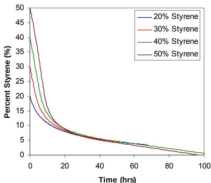
Figure 15. Percentage of styrene as a function of emission time.
