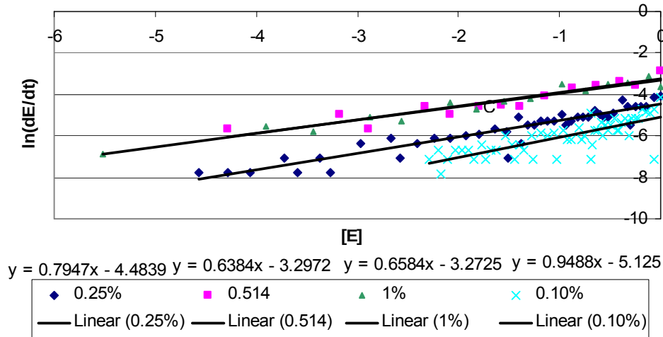
Figure 142. Representative plots of \ln(dE/dt) vs. [E] for experiments conducted at 80°C for four catalyst concentrations.
