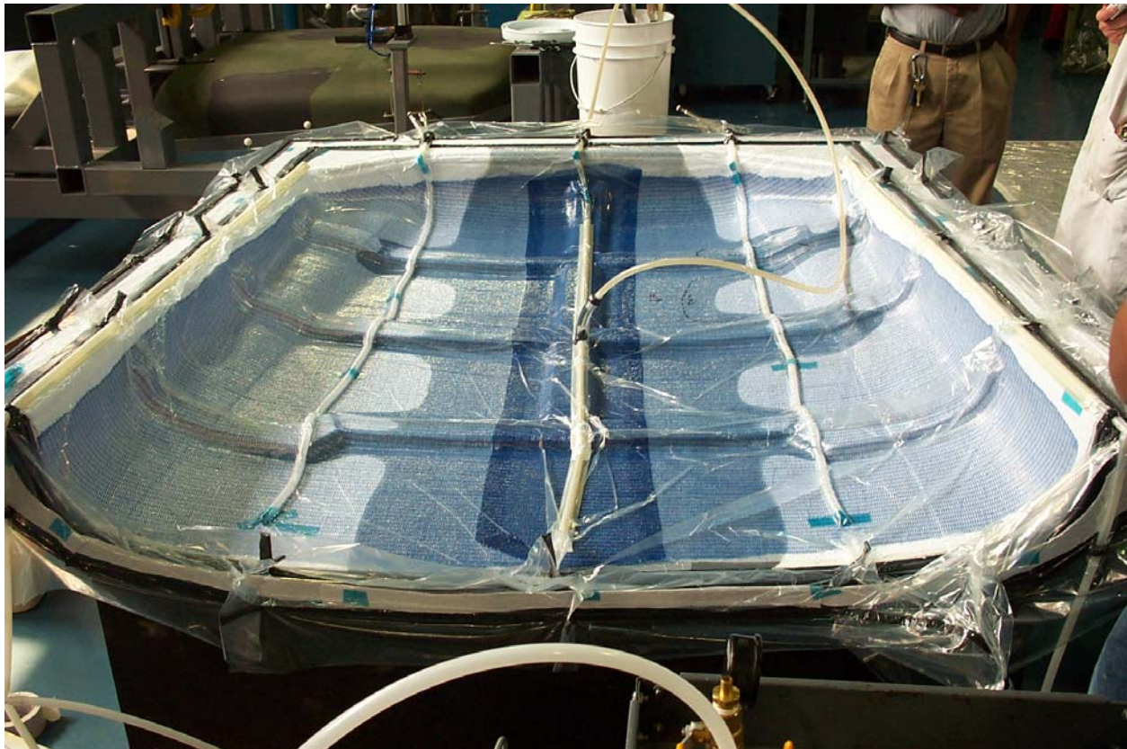
Figure 173. The resin infused fairly uniformly except that it race-tracked at the foam stiffeners.
