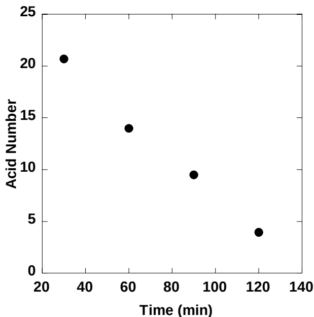
Figure 68. Acid number measurements during reaction at 90°C for the synthesis of Methacrylated Lauric Acid (MLau)
