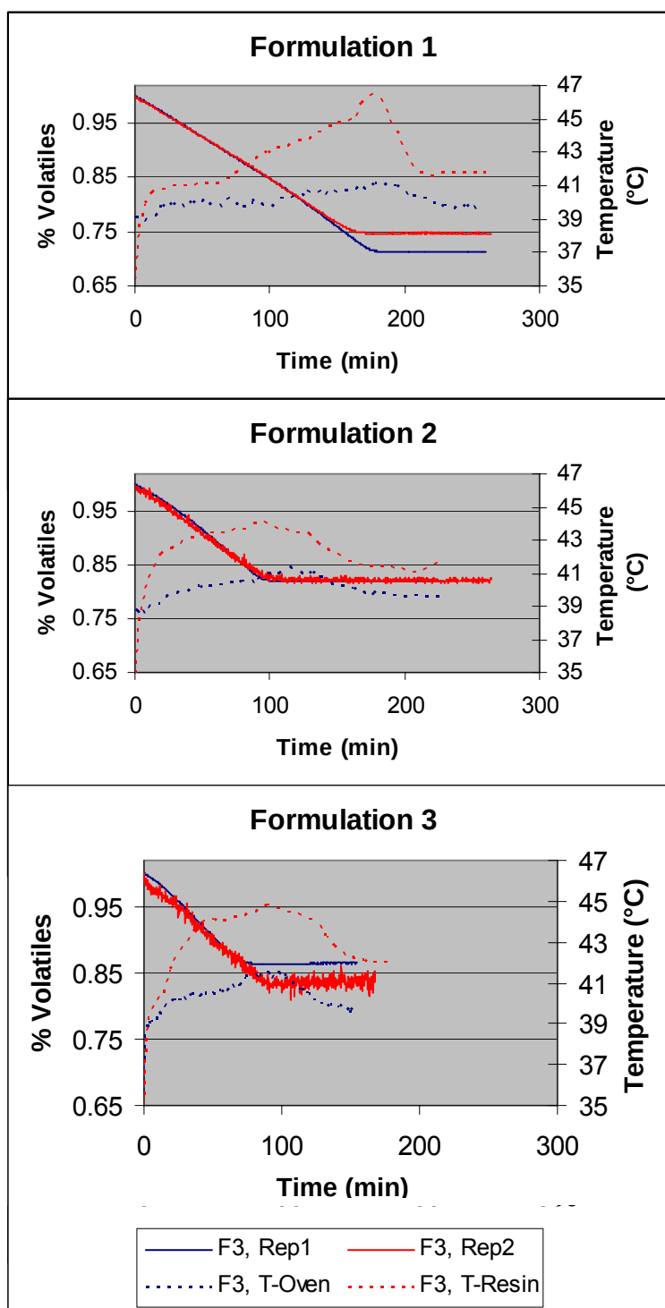
Figure 18. Percent volatiles and temperature as a function of cure time.
