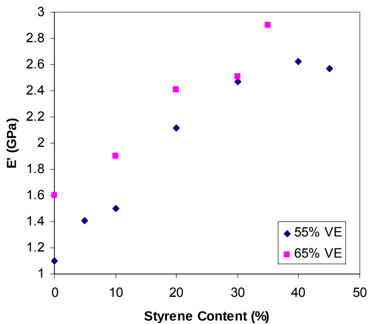
Figure 110. The storage modulus as a function of styrene content for VE/MOA/styrene blends.
