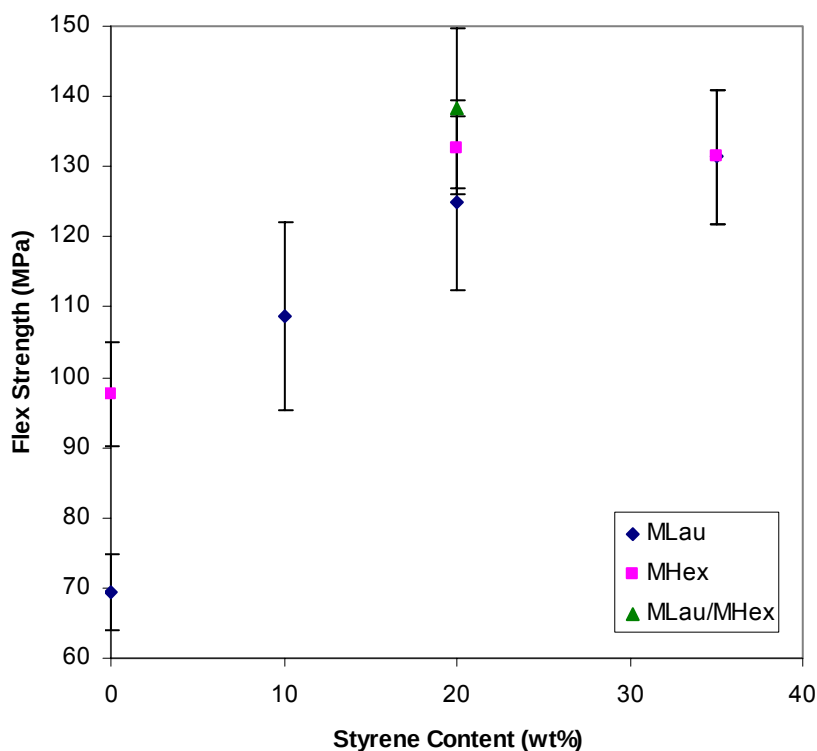
Figure 130. The flexural strength as a function of styrene content for MHex and MLau-based resins.
