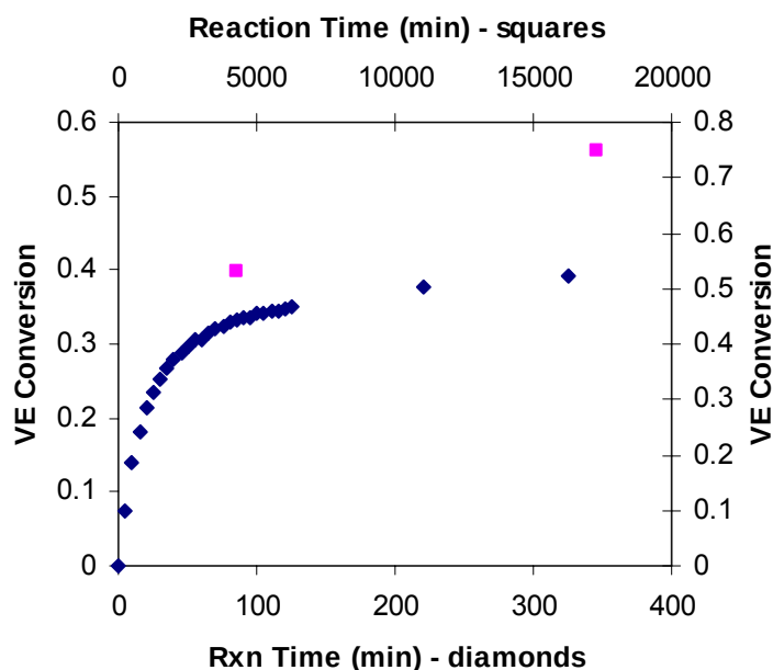
Figure 80. The extent of cure of VE as a function of time in the mixture of VE, FAME, and CoNap. There are two x-axes in order to show both the short-term VE cure and the long-term VE cure.
