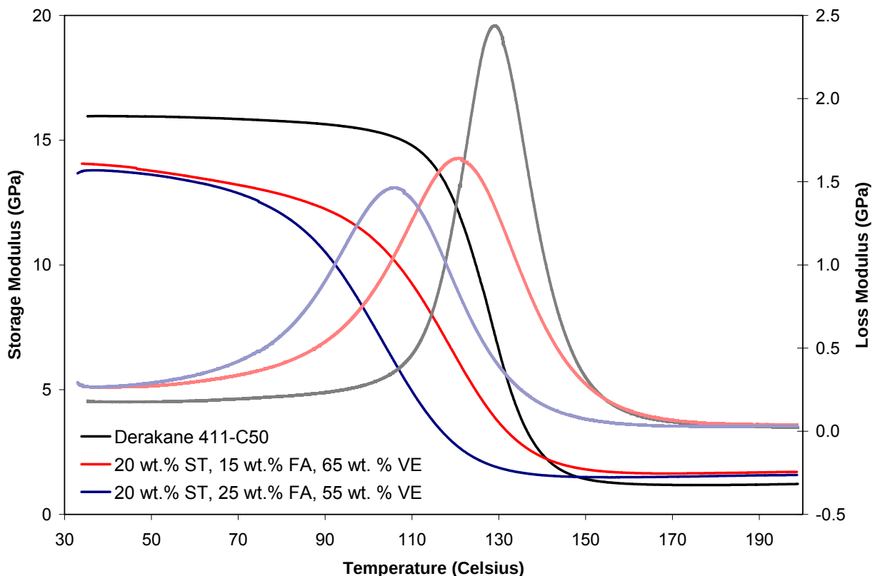
Figure 165. DMA scans of composites with G'-sized AS4 carbon composites with low VOC resins and Derakane 411-C50.
