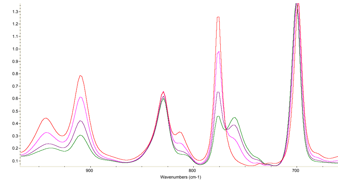
Figure 10. The FTIR spectrum of VE/styrene as a function of cure time.
