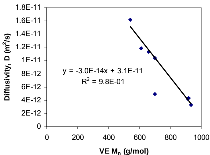
Figure 54. The diffusivity as a function of vinyl ester molecular weight for bimodal systems.
