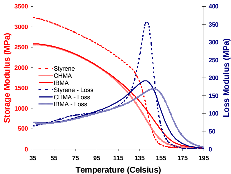
Figure 65. The DMA behavior of VE/CHMA and VE/IBMA resins relative to VE/styrene.
