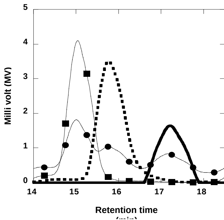
Figure 69. Reaction of Lauric Acid with Glycidyl Methacrylate to form MLau. Methacrylated lauric acid (MLau) (●) 0 min, (■) 90 min (—), Glycidyl methacrylate, (□) Pure lauric acid.
