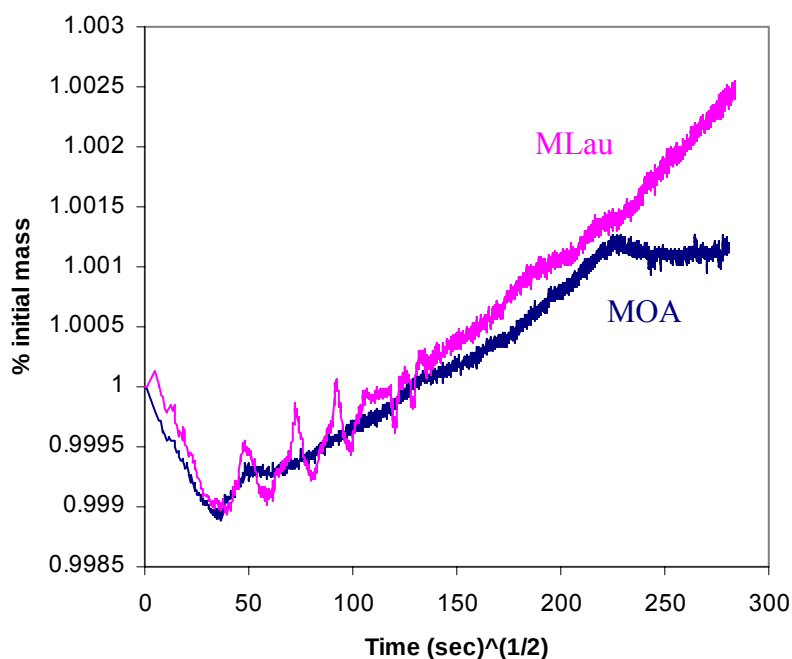
Figure 139. The percentage mass change as a function of time for MFA monomers.
