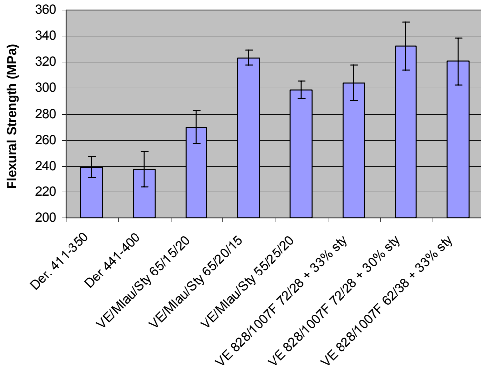
Figure 163. Flexural strength for commercial resins and low VOC formulations using 9 oz glass fiber reinforcement.
