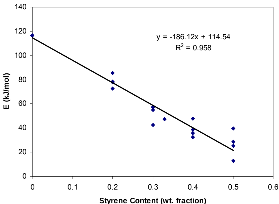
Figure 43. The activation energy for viscous flow as a function of styrene content in VE resins.
