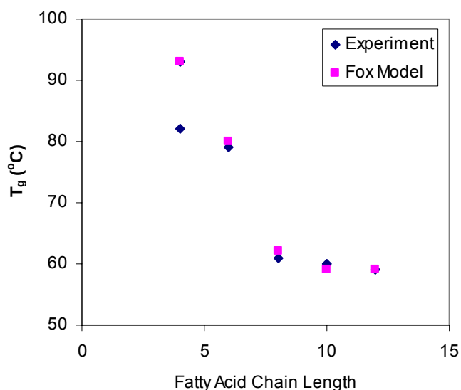
Figure 100. Glass transition temperature behavior changes with increasing chain length of VE samples with 45 wt% MFA as determined by experiment and as predicted by the Fox Model.
