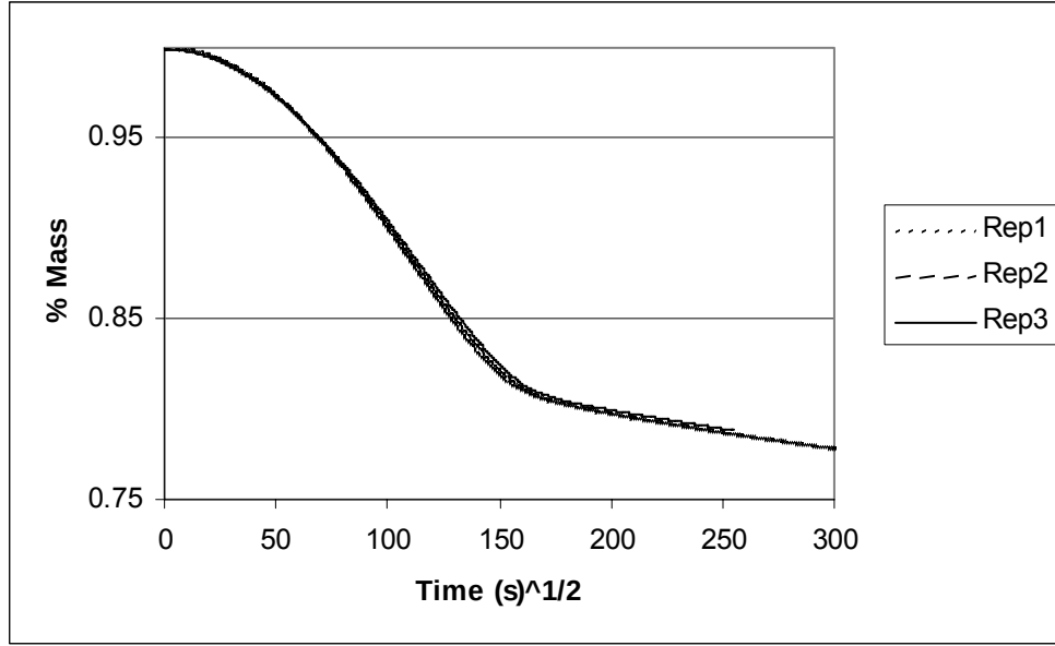
Figure 12. Reproducibility of macro-TGA analysis, 40°C, Derakane 470-300 resin.
