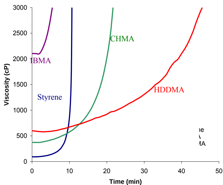
Figure 58. The viscosity of VE resins as a function of gel time and comonomer. VE/HDDA results are very similar to VE/HDDMA results and are omitted for clarity.
