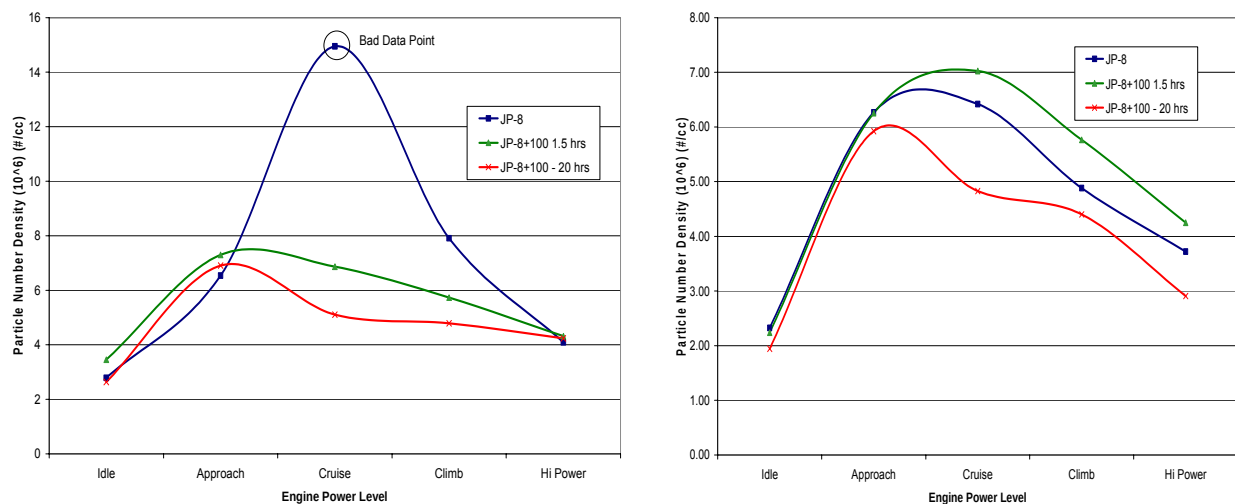
Figure 192. PND as a Function of Power Setting for T-43 Engines 608 and 636.
