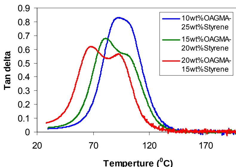
Figure 151. The tan delta curves of Viapal-MOA-Styrene polymers at 10-20 wt.% MOA content. (35 wt.% total comonomer content)
