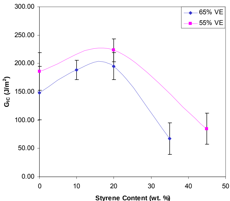
Figure 118. G_{IC} of VE/MLau/styrene as a function of styrene content in the resin for resins containing 55 wt% and 65 wt% VE 828.
