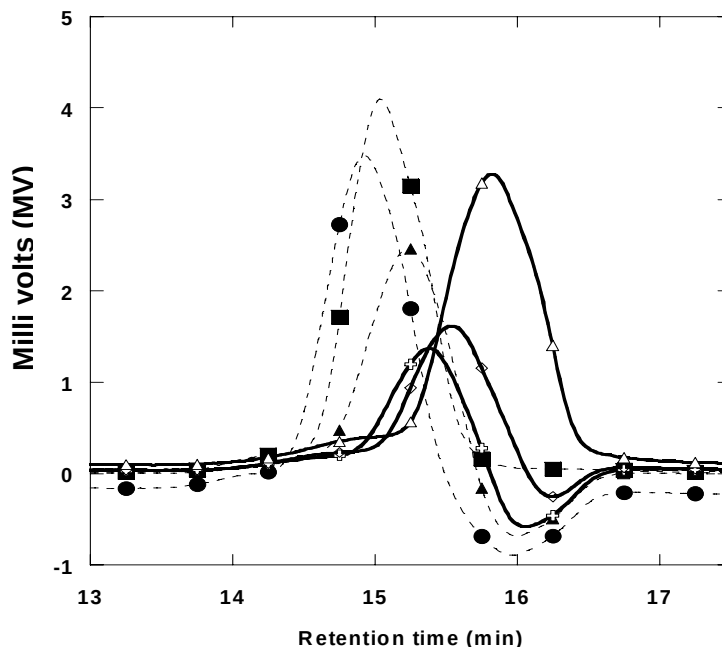
Figure 71. The peak shift of the Methacrylated fatty acids (MFA) with increasing chain length of fatty acids, methacrylated Myristic acid (●), methacrylated lauric acid (■), methacrylated capric acid (▲), methacrylated caprylic acid (◆), methacrylated caproic acid (◇), methacrylated butyric acid (△).
