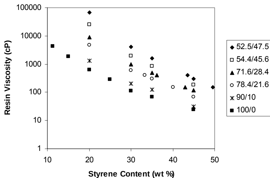
Figure 36. The resin viscosity as a function of styrene composition for various bimodal VE compositions of VE 828/1007F.
