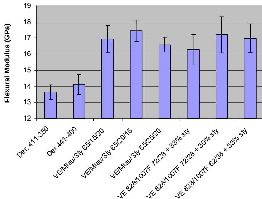
Figure 162. Flexural modulus for commercial resins and low VOC formulations using 9 oz glass fiber reinforcement.
