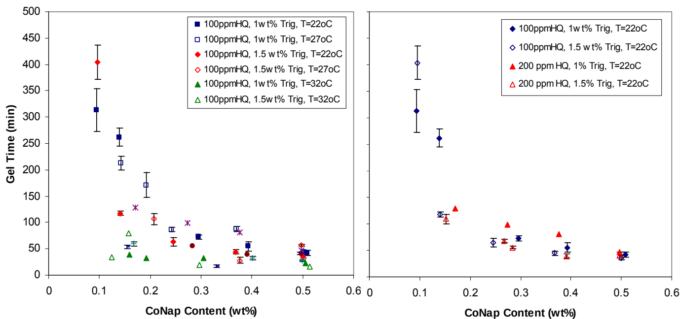
Figure 161. The gel time for CN-151/MLau/Sty 65/15/20 as a function of cure temperature, inhibitor, initiator, and catalyst contents.
