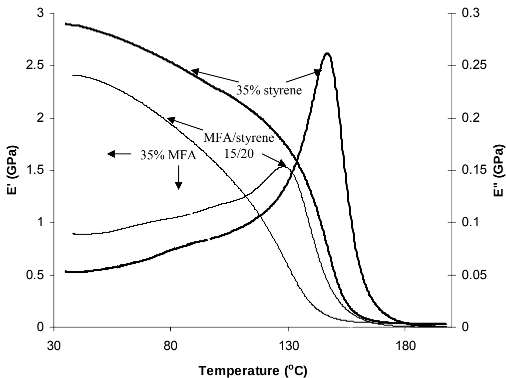
Figure 109. DMA behavior of VE/MOA/styrene with 65 wt% VE 828.
