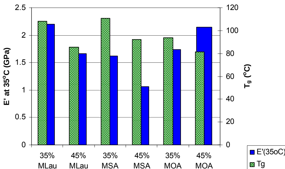
Figure 105. The storage modulus and T_g of fatty acid-based vinyl esters cured thermally and via E-beam.
