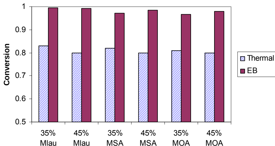
Figure 103. The extent of cure of fatty acid-based vinyl esters, comparing thermal cure to E-beam.
