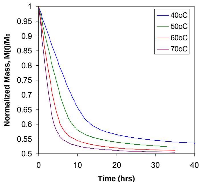
Figure 16. Fractional mass loss of styrene in the VE 828 resin system having 50% styrene under different isothermal conditions in the study of temperature variation.
