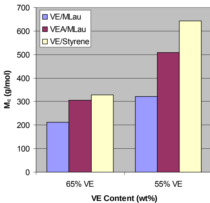
Figure 124. The molecular weight between cross-links for VE/MLau, VEA/MLau, and VE/styrene polymers.
