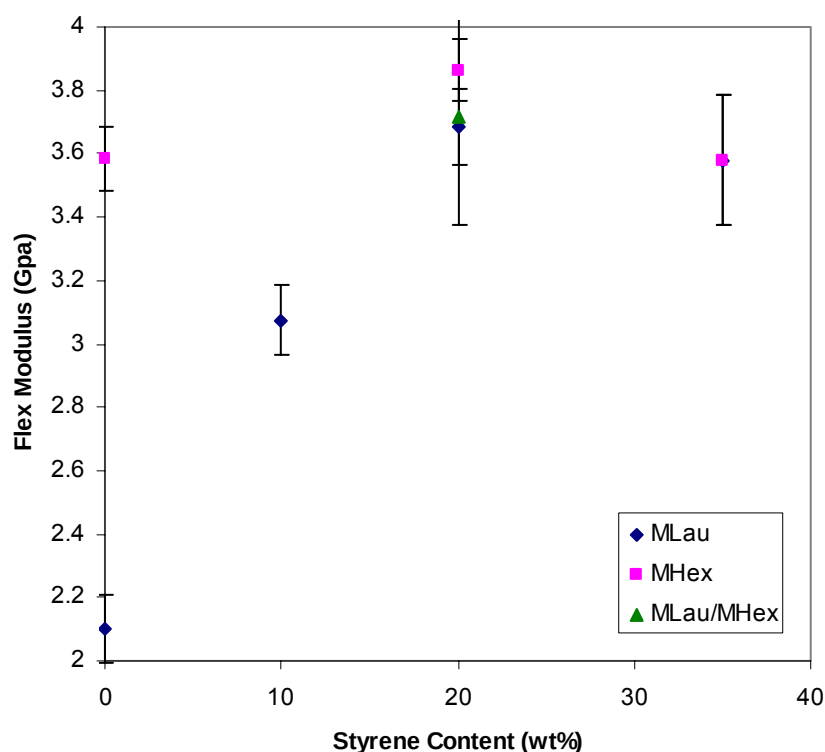
Figure 131. The flexural modulus as a function of styrene content for MHex and MLau-based resins.
