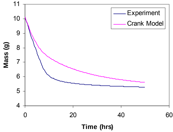
Figure 24. Comparison of model and experimental values of mass loss behavior of styrene through VE 828/Styrene 50/50 resin system under 40°C isothermal conditions.
