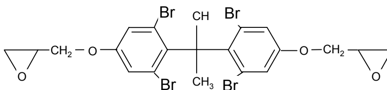
Figure 119. The chemical structure of ortho- tetra bromo-diglycidyl ether of Bisphenol A (DGEBA).
