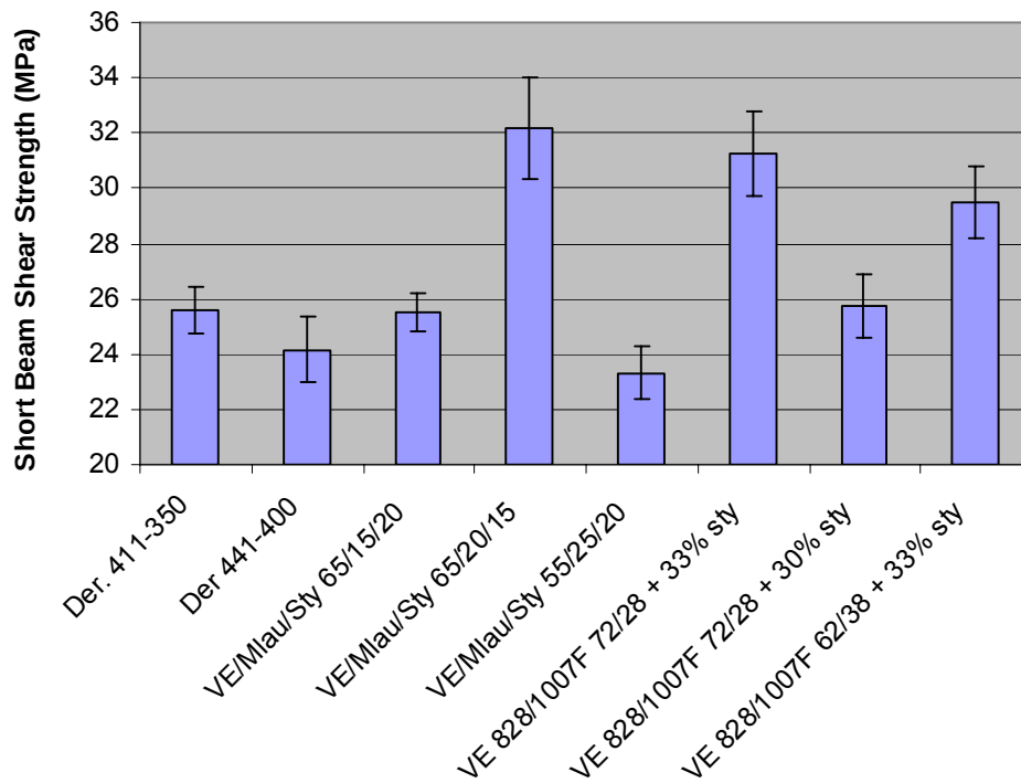
Figure 164. Short beam shear strength for commercial resins and low VOC formulations using 9 oz glass fiber reinforcement.
