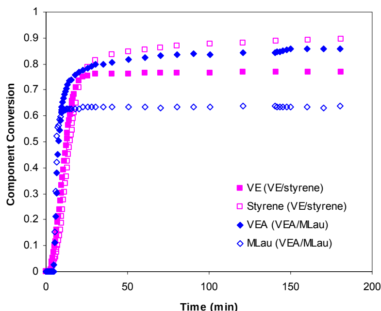
Figure 96. The individual cure kinetics of the components of VE/styrene and VE/MLau, each containing 45% reactive diluent.
