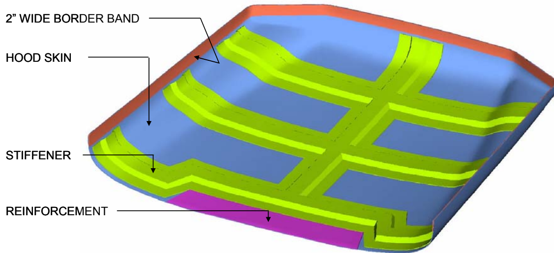
Figure 167. Bottom view of the hood with the stiffeners.
