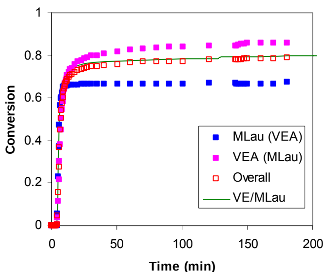
Figure 125. The overall conversion of VE/MLau is similar to that of VEA/MLau for resins containing 45 wt% MLau.
