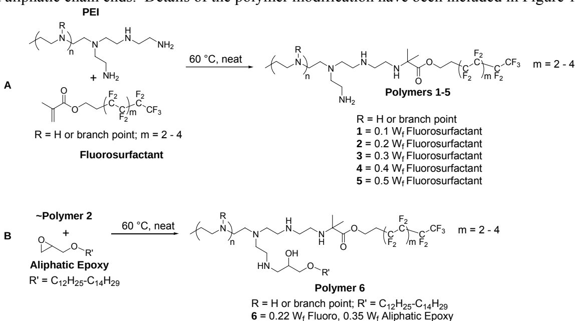
Figure 180. Synthetic scheme for modification of branched PEIs
