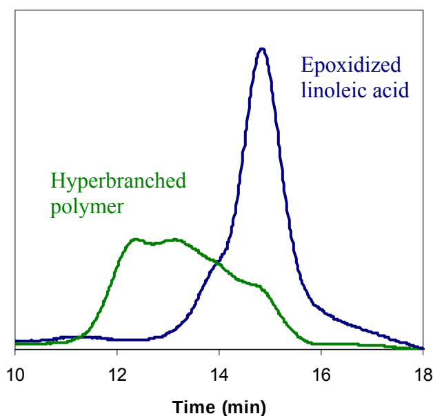
Figure 191. The SEC traces of epoxidized linoleic acid compared to that of hyperbranched polymers derived from epoxidized linoleic acid and epoxidized soybean oil.
