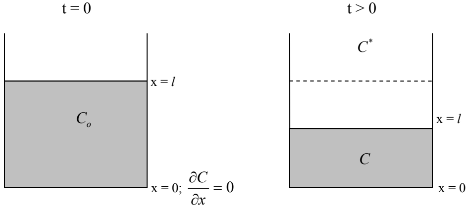
Figure 20. An illustration of a VE system initially (left) and the VE after a long time (right).
