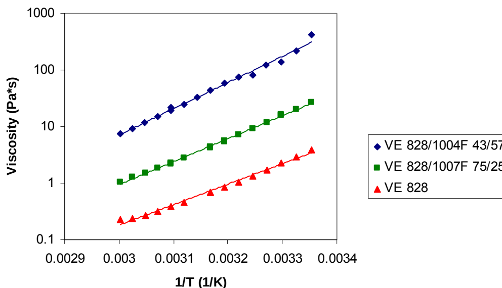
Figure 42. The viscosity-temperature dependence is Arrhenius for VE resins with 20 wt% styrene.
