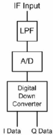
Figure 47. OSU/ESL Digital Down Converter (DDC) Radar Receiver Architecture.
