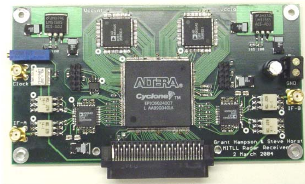
Figure 49. OSU/ESL Dual Channel Digital Receiver.
