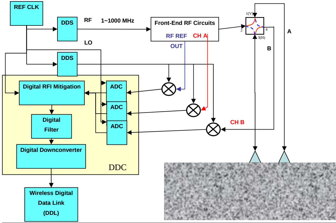
Figure 44. New OSU/ESL GPR System Block Diagram.
