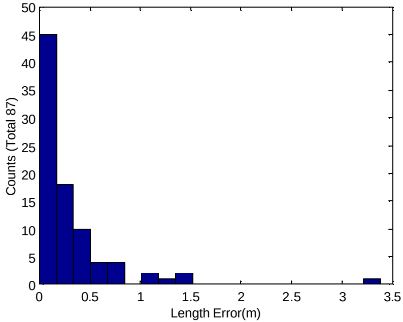
Figure 35 Histogram of the length estimation error for the total 87 UXO-like targets.
