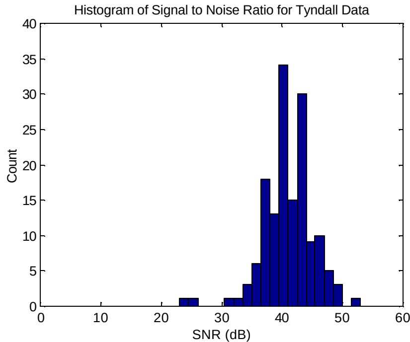
Figure 21 Histogram of the SNR for Tyndall targets.
