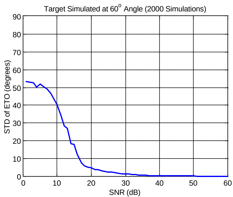
Figure 25 STD of the estimated ETO in random Gaussian noise.
