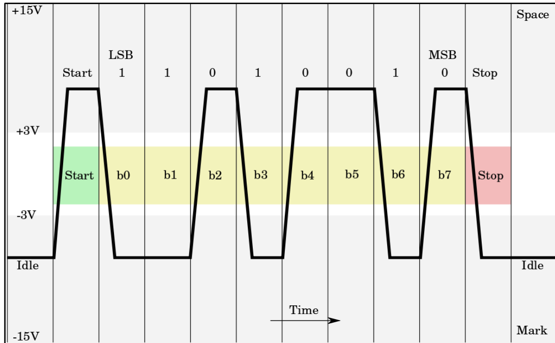
Figure 23. RS-232 Data Transmission.
