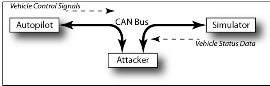
Figure 21. Simulated attack configuration.
