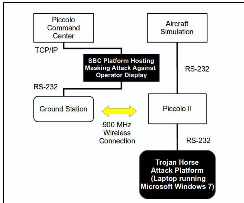
Figure 15. Embedded attack platform for masking the operator display on a SBC.
