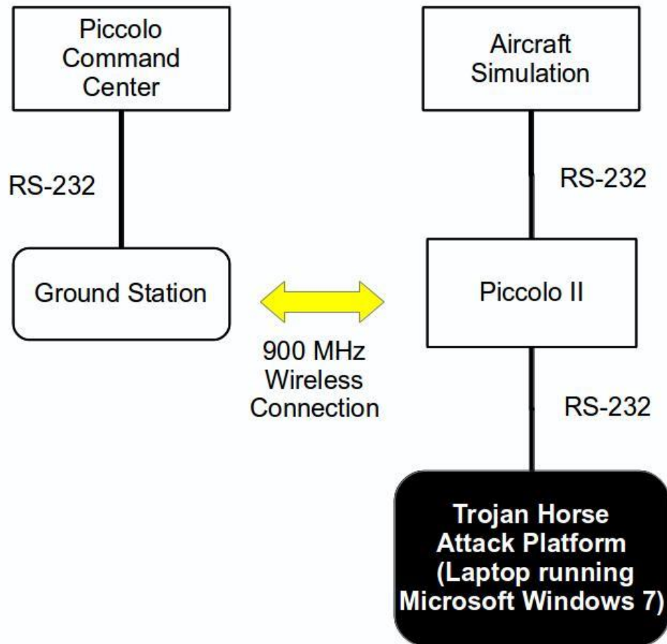
Figure 14. Piccolo II HiL configuration with an Embedded Attack Platform to dynamically direct the UAV to a specified waypoint during flight. The Embedded Attack Platform is a laptop connected to the Piccolo II autopilot via a serial connection using the RS-232 protocol.
