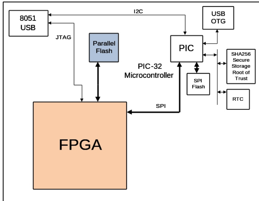
Figure 40. UAV SHIELD block diagram for the the FPGA with supporting cryptographic HW.
