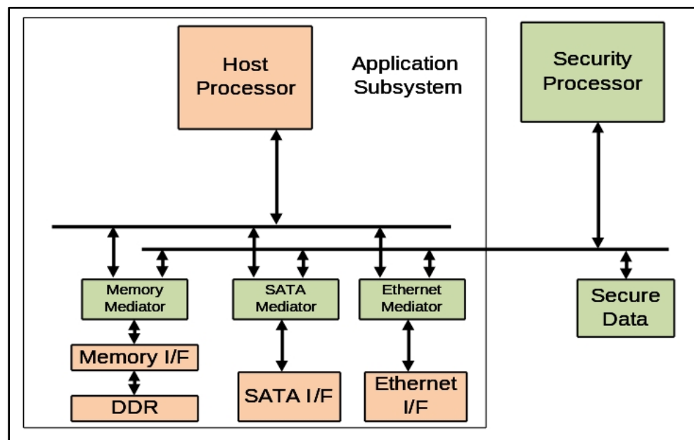
Figure 42. Block diagram of the NetFPGA-7 mediators.
