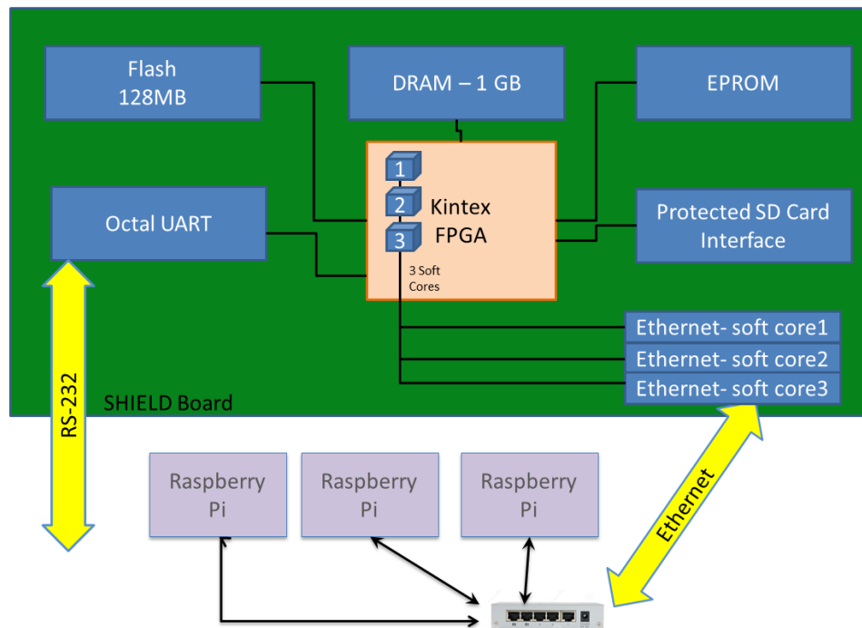
Figure 43. Block Diagram of the UAV SHIELD board.
