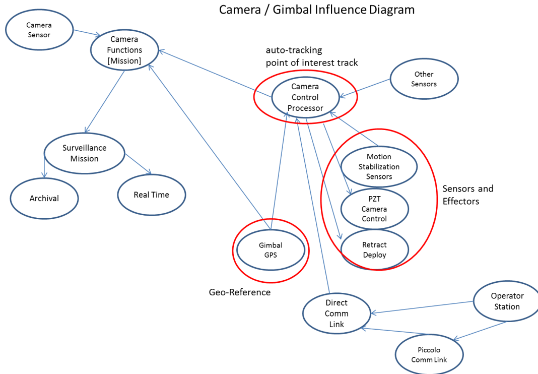
Figure 7. Influence diagram used to understand the relationship between the UAV subsystems used for gathering surveillance data.
