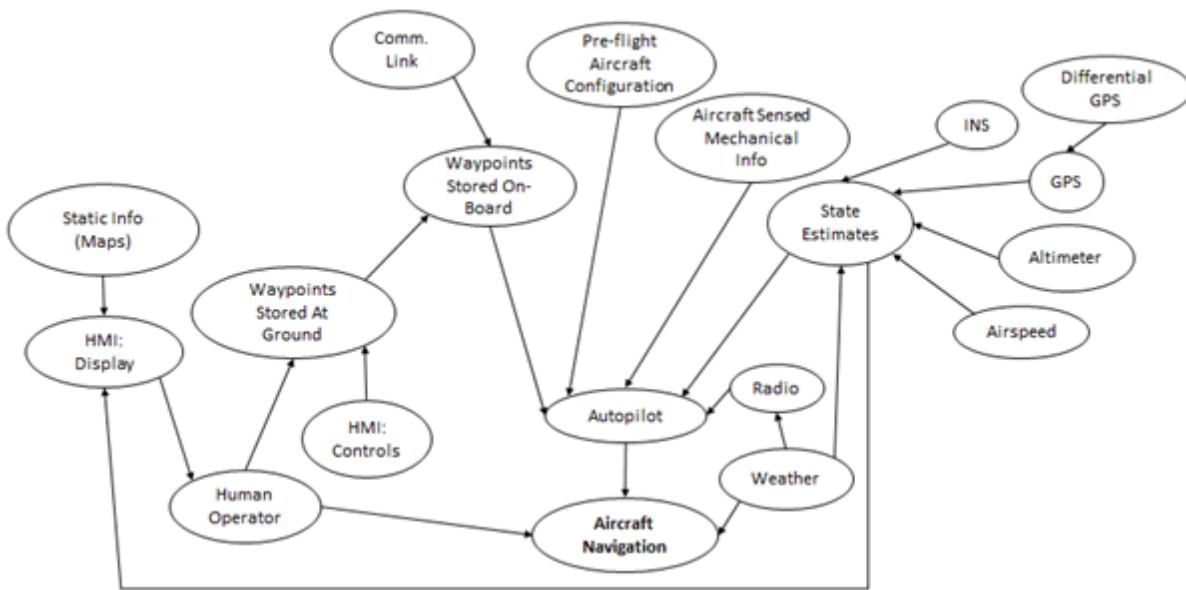
Figure 6. Influence diagram for used to understand the relationship between the UAV subsystems used for navigation.
