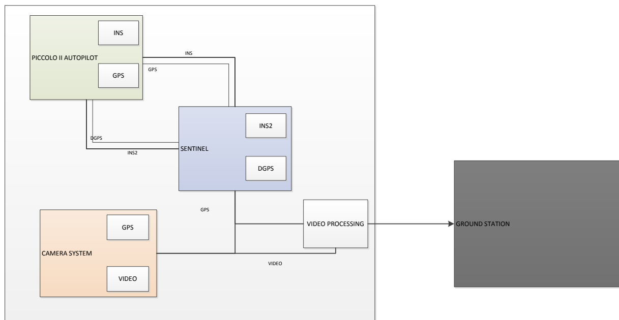
Figure 32. Architecture for camera system.
