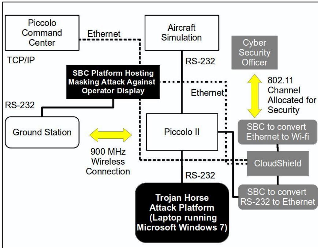
Figure 30. CloudShield Sentinel monitors Piccolo Command Center interface for integrity violations.
