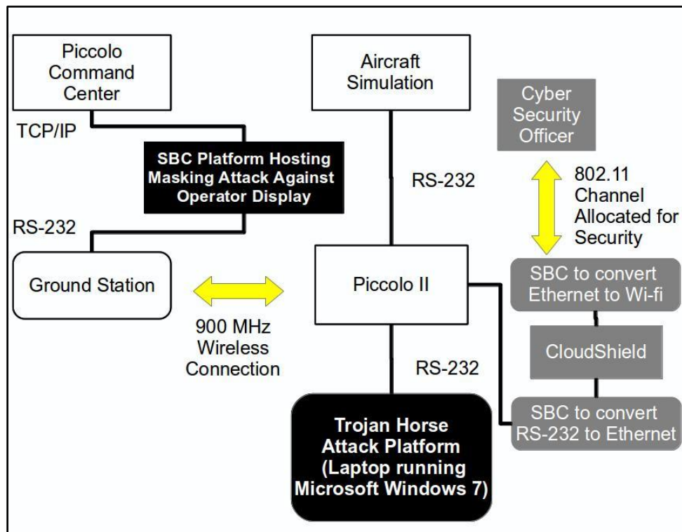
Figure 29. Sentinel (CloudShield) using SBC to convert data from RS-232 to TCP/IP.
