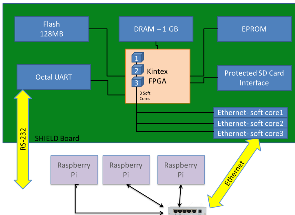
Figure 38. Proposed UAV SHIELD architectural block diagram.
