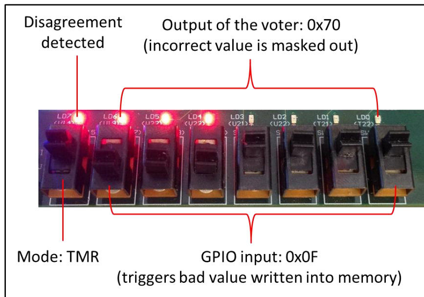
Figure 36. TMR Detects and Masks Deviated Operation.
