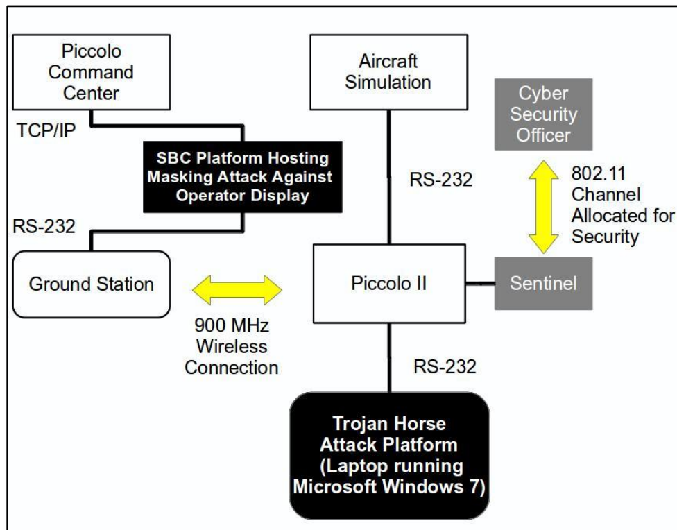
Figure 28. Super secure smart Sentinel for protection with a designated cyber security officer.
