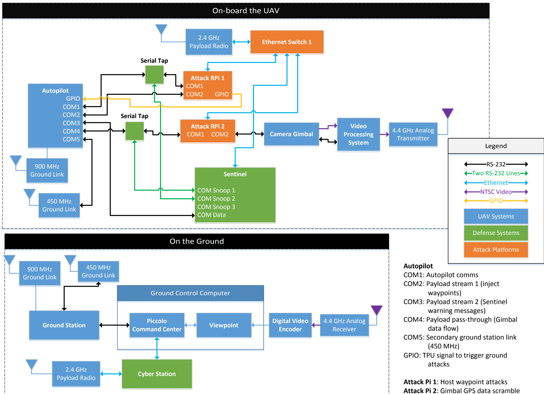
Figure 37. Architectural block diagram illustrating how the UAV SHIELD Sentinel will be integrated into the GTRI's GAUSS platform.
