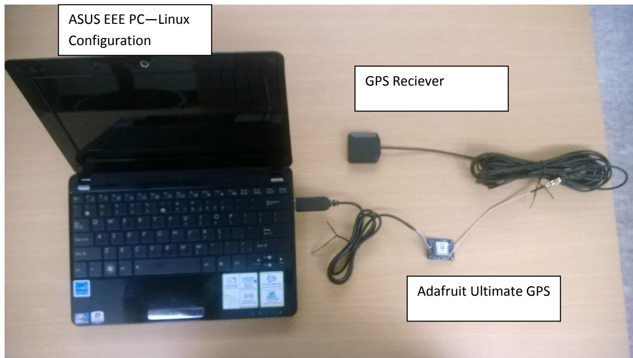
Figure 34 – Ground-based Navigation Experimental Environment
