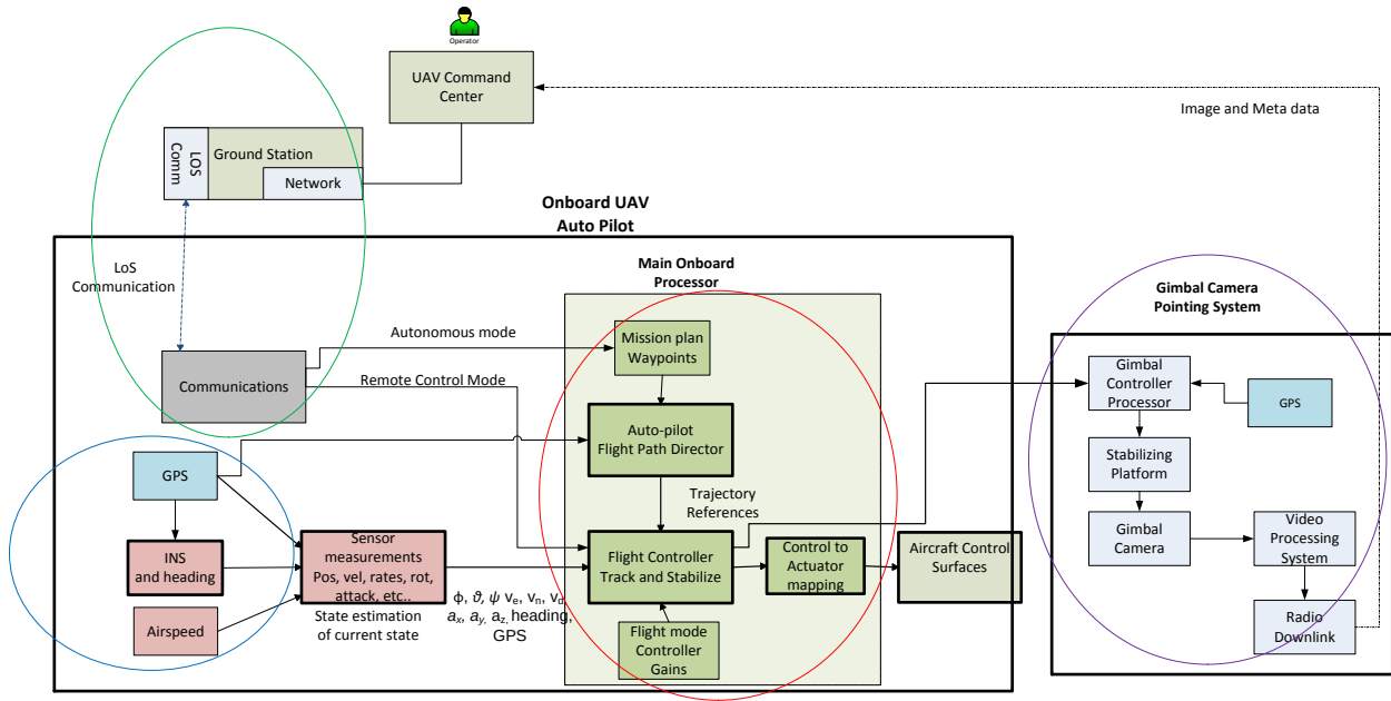
Figure 5. UAV Onboard Systems showing the four major system groups.
