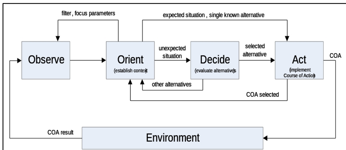
Figure 41. OODA Real-time controller that implements the OODA loop on the SHIELD Coprocessor.
