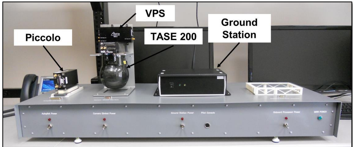
Figure 2. The GTRI HiL emulation environment.
