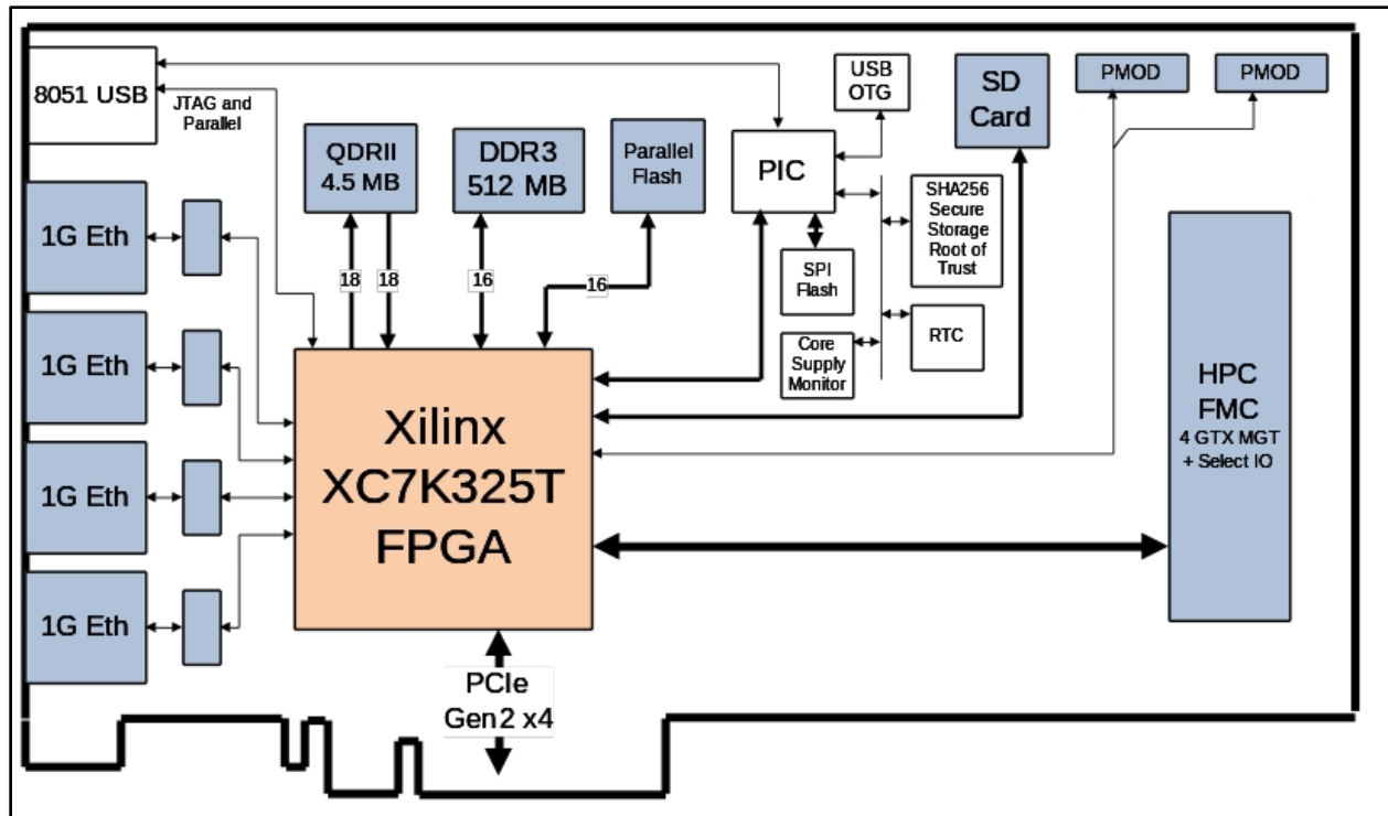
Figure 39. NetFPGA-7 architectural block diagram.
