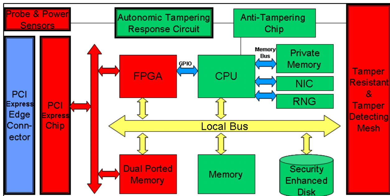
Figure 27. Block diagram of the Sicore SHIELD Coprocessor.
