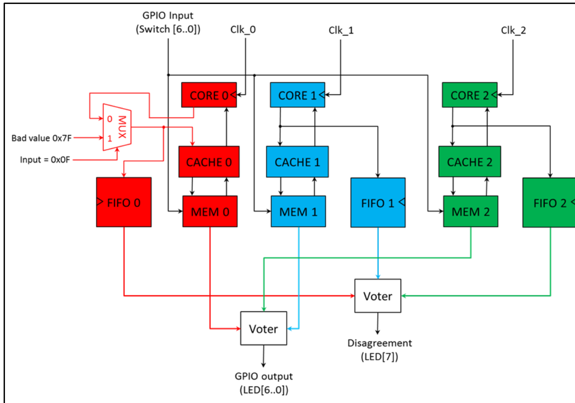
Figure 35. Block diagram of a FPGA configured to provide detection and recovery with TMR.
