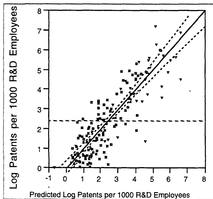
Figure 5.5—"Whole Model" Leverage Plot for Table 5.16 regression for the entire data set
