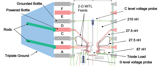
Figure 2. Diagram of the rod-bottle interface and vacuum load configuration with vacuum inductances for the A, B, C, and D levels indicated.
