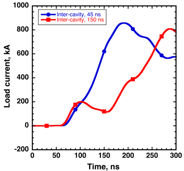
Figure 5. Pulse shaping with delay times comparable to the cavity rise time.
