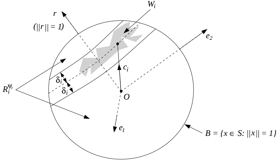
Figure 1: An illustration of the class assumption for a low dimensional example, S = \mathbb{R}^3 . The subspace, L_i , is the 2 dimensional subspace spanned by the vectors, \{e_1, e_2\} . Every vector in W_i can be approximated to within an error, \delta_i , by the linear combination of c_i and a vector in L_i . The rejection vector, r , is a unit vector orthogonal to the subspace L_i . The rejection domain, R_i^{\psi_r} , of the derived rejector, \psi_r , consists of all points, x \in B , which have a projection in the direction of the rejection vector, r , at least \delta_i away from the projection of c_i .
