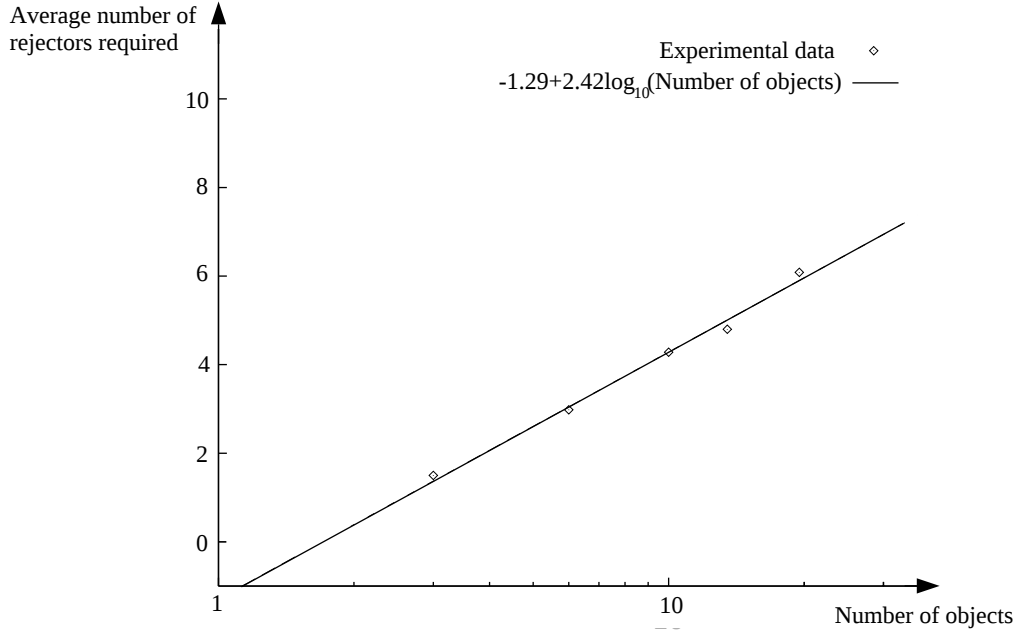
Figure 7: A graph of the number of objects against the average number of simple rejectors required to completely discriminate between objects. The graph is plotted using a log scale on the abscissa, implying a logarithmic growth rate in the time complexity.
