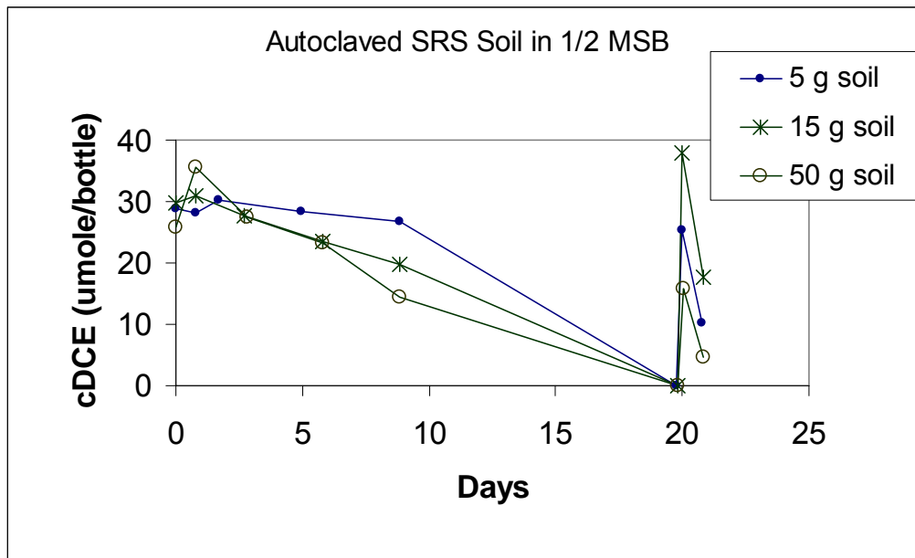
Figure 4.8. Autoclaved SRS Soil Inoculated with JS666 and Amended with ½ MSB and 10 mM Ethanol. Results for 5, 15, and 50 grams of soil. Duplicates behaved similarly (not shown).
