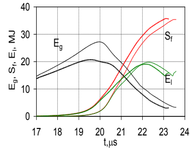
Figure 5. Simulated FOS voltage U_f ( a ), power W_f ( a ) and electromagnetic energy flux S_f delivered through FOS to the load, magnetic energies E_g and E_l in DEMG and in the load ( b ), - for the system with foil thicknesses of 0.12 and 0.15 mm (thick and thin lines, systems 1 and 2 with I_0 = 7\text{MA} , Table 1).
