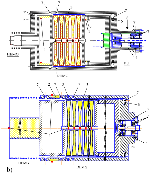
Figure 1. Schematic drawings of the systems and their diagnostic suites in ALT-1,2 [1] (a) and in [4] (b). 1 – detonators; 2 – ECS; 3 – FOS; 4 – liner; 5 – CMU; 6 and 7 – Faraday and B-dot probes; 8(a) – radiographic equipment; 8(b) – place to install ECS in the load.
