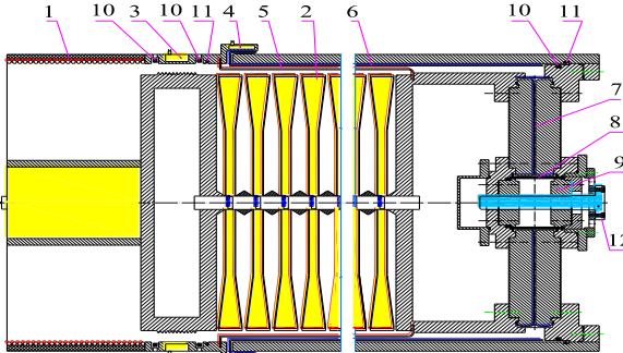
Figure 2. Schematic drawing of the ALT-3 system and its diagnostic suite.
