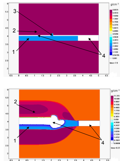
Figure 3. Density isolines from 2D MHD simulations of the connection between the Al liner (1) and the Cu return conductor (2) in the initial state (top) and \sim 10 \mu s after reaching the peak current of \sim 66 MA (bottom). 3 – Al contact ring, 4 – vacuum gaps.
