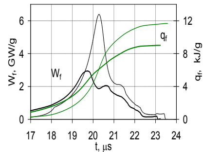
Figure 6. Simulated squared current density j_f^2 and effective relative resistivity \Omega_f/\Omega_0 ( a ), specific power w_f and Joule heating of the FOS Cu foil q_f ( b ), - for the system with foil thicknesses of 0.12 and 0.15 mm (thick and thin lines, systems 1 and 2 with I_0 = 7\text{MA} , Table 1).
