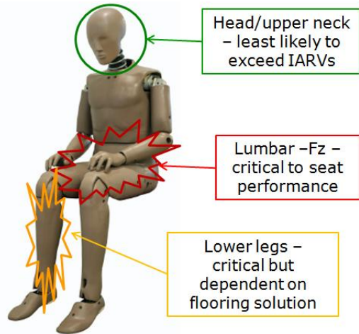
Figure 6. Schematic of ATD with body segments marked in order of importance.
