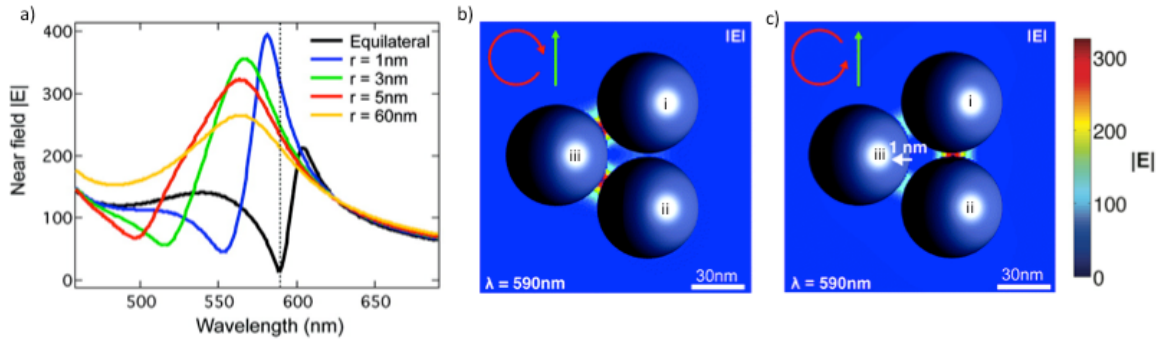
Figure 2 Near-field properties of the tangentially excited trimer as a function of the perturbation parameter, r . (a) The near-field amplitude between particle i and ii as a function of r . The vertical dotted line marks \lambda = 590 nm. (b) Near-field amplitude map, calculated at all points in the dielectric medium between the particles of the equilateral trimer at \lambda = 590 nm. (c) Near-field amplitude map for the isosceles trimer with r = 1 nm at \lambda = 590 nm.
