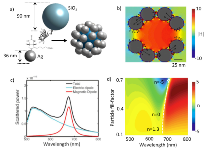
Figure 3. (a) Meta-molecule design. (b) The near-field properties of the metamolecule at the magnetic dipole resonance frequency (668 nm). The cross-sectional colormap shows the near-field magnetic enhancement, while the overlaid arrows display the displacement current between the silver nanoparticles. The strong magnetic field enhancement across the middle of the metamolecule and the circulating displacement currents are a signature of the magnetic dipole mode. (c) Multi-polar decomposition of the scattered fields into the electric and magnetic dipolar contributions. (d) Effective refractive index as a function of wavelength and fill factor.
