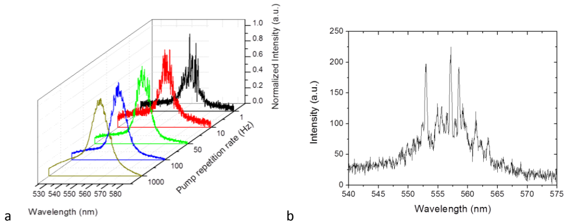
Fig. 4 – (a) Lasing spectrum obtained at different repetition rates; (b) Lasing spectrum at 1Hz. The pump excitation and pump area were 50μJ and 2.8 \times 10^{-3} \text{ cm}^2 , respectively.
