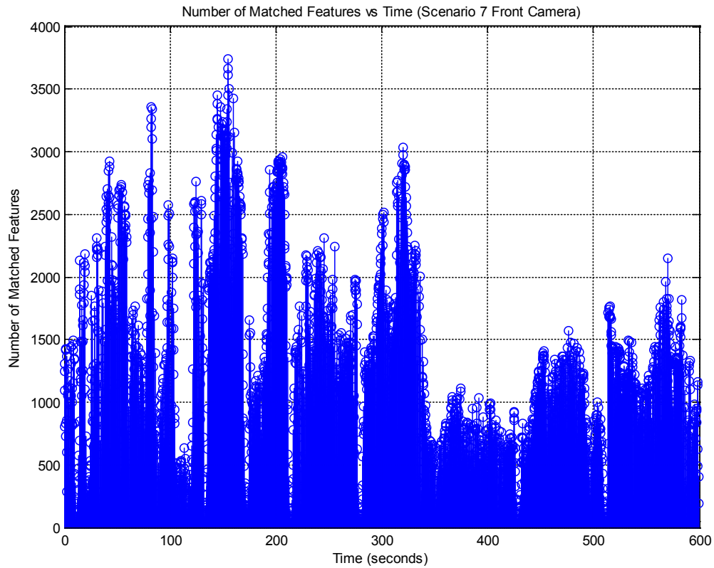
Figure 27. Number of Matched Features Found from Scenario 7 Front Camera Images. There are at least 42 matched features between all the 2399 successive pairs of images. This is the only set of photos where there are measurements from all the images.
