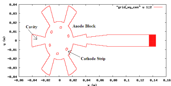
Figure 2. Grid plot of the transparent cathode with A6 magnetron.
