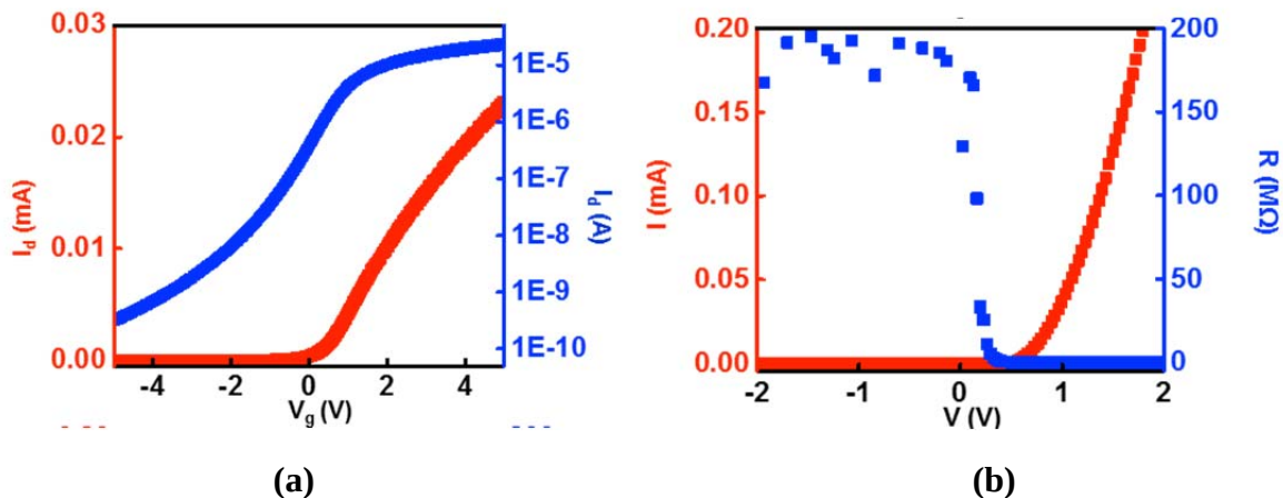
Figure 12. Electrical Characteristics of a N-MOSFET and a PIN Diode Fabricated on PPA (a) Transfer curve of a transistor on PPA shows that the mobility (linear regime) and on/off ratio are \sim 350 \text{ cm}^2 \text{ V}^{-1} \cdot \text{s}^{-1} and \sim 10^5 , respectively. (b) The I-V curve of the diode shows defined diode characteristics
