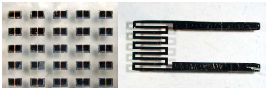
Figure 2. Transient Electronics Deposited on PPA Films
