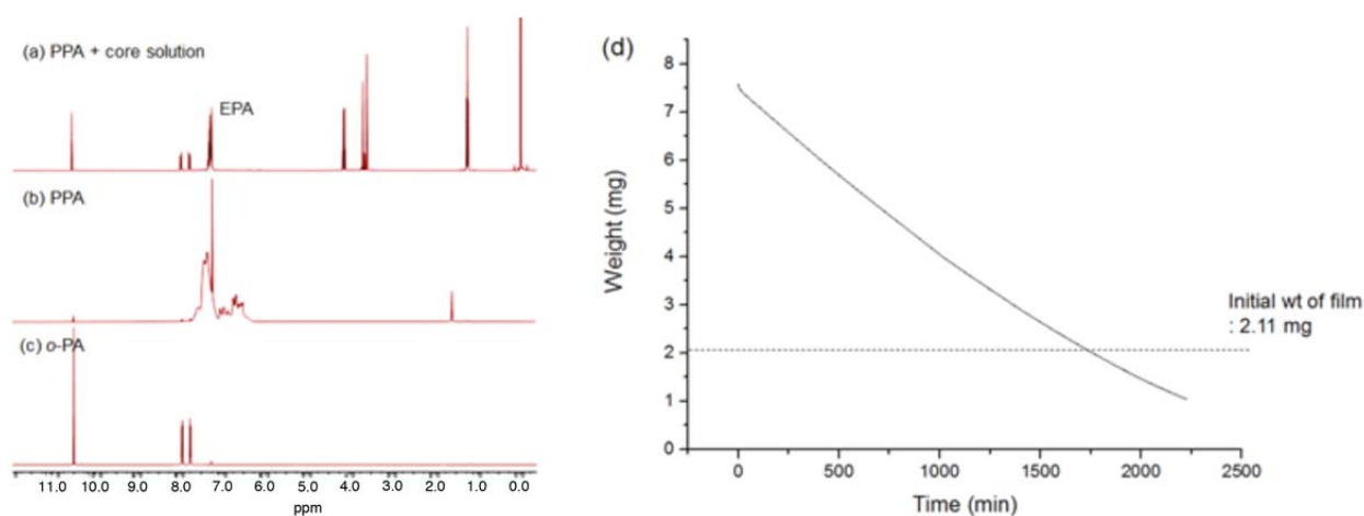
Figure 19. Characterization of PPA Degradation Triggered by Acid Microcapsules NMR spectra of (a) PPA film treated with the acid core solution, (b) PPA film, and (c) o -PA, monomer of PPA. (d) An isothermal TGA trace of PPA film treated with the acid core solution at 25 ^{\circ}\text{C} after 38 h.
