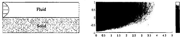
FIG. 1.33. Left: Computational domain for motivational example. Right: Temperature fields within the fluid and the solid.
