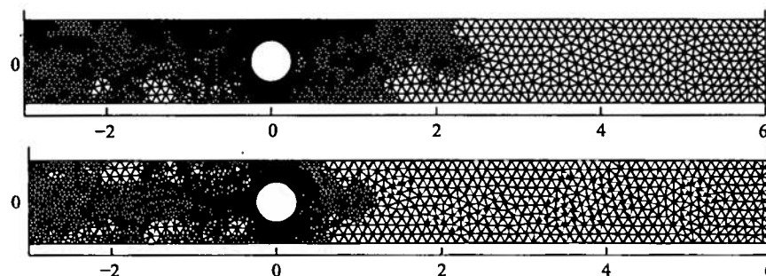
FIG. 1.31. Upper: Final adaptive mesh in the fluid when the quantity of interest is the temperature in a small region in the wake above the cylinder. Lower: Final adaptive mesh in the fluid when the quantity of interest is the temperature in a small region in the center of the solid.
