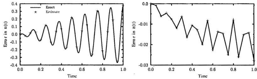
Fig. 5. Time history of the error for solving (35). Left: x(t) . Right: z(t) . The time steps \Delta t = 0.05 , \Delta s_1 = \Delta t/128 , \Delta s_2 = \Delta t .
