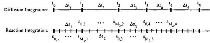
FIG. 1.4. Discretization of time used for multiscale operator splitting
