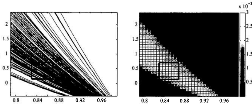
FIG. 4.2. Illustration of an application of Algorithm 1. Left: We determine which contours are contained in an event A \subset \Lambda and how much of each contour is inside the event. Right: We estimate the probabilities of small cells contained in the event and use an inner and outer estimate to obtain an approximation of the probability of the event A .
