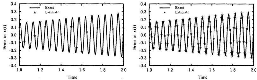
Fig. 10. Time history of error in x for solving (34). Left: \Delta t = 0.05 , \Delta s_1 = \Delta t/1600 , \Delta s_2 = \Delta t/32 . Right: \Delta t = 0.00625 , \Delta s_1 = \Delta t/200 , \Delta s_2 = \Delta t/4 .
