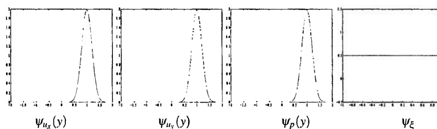
FIG. 12. Adjoint data profiles for Case 3. The plots of \psi_{u_x} , \psi_{u_y} , and \psi_p are shown in one dimension because they have no variation in the x -direction, and \psi_\xi is a one dimensional function defined on the interface.
