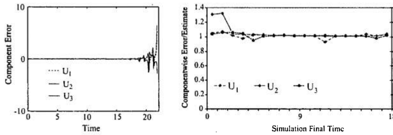
FIG. 1.16. Left: We plot an approximate error in each component of a numerical solution of the Lorenz problem computed by taking the difference between solutions with estimated error .001 and .0001 at many times. Right: we plot the pointwise error/estimate ratios for each component versus time at many time points.
