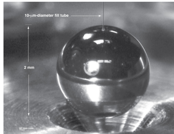
Figure 3. Beryllium capsule and fill tube.
