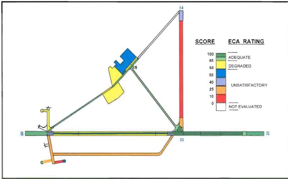
Figure 3.1.1 The condition of the hard surfaces of the airfield determined by the Comprehensive Range Plan Avon Park Air Force Range, Florida, October 2006.
