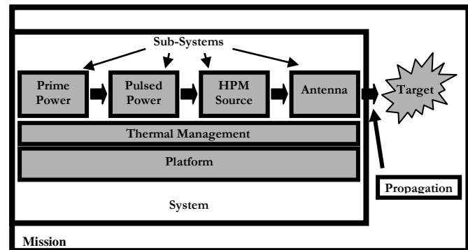
Figure 1. Conceptual structure of the HEIMDALL system model.
