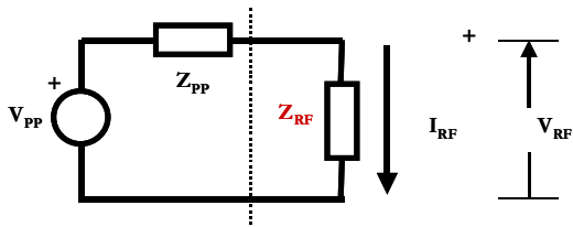
Figure 4. Electrical model of the Pulsed Power and RF Source connection. The dashed line shows the division between the Pulsed Power to the left and the RF Source to the right, with V_{PP} and Z_{PP} the open-circuit voltage and output impedance of the Pulsed Power and V_{RF} and I_{RF} the voltage across, current through, the RF Source impedance Z_{RF} .
