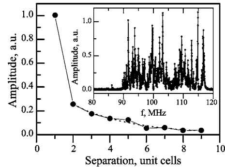
FIG. 3. The inset shows an acoustic band in the vibration spectrum of the 20 \times 20 array of coupled resonators. The excitation was provided at the center of the array and the detection laser was positioned 5 unit cells away. Solid circles in the main plot demonstrate spatial decay of the average acoustic energy of vibrations as a function of separation distance between the drive and detect laser spots. The dotted line shows an exponential fit for the decay.
