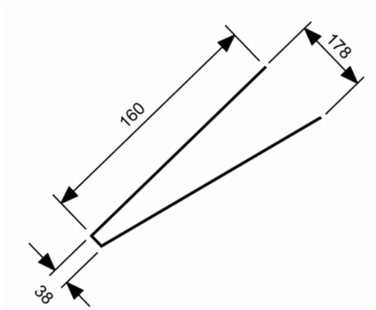
Figure 5.5 Quest bilge keel dimensions
