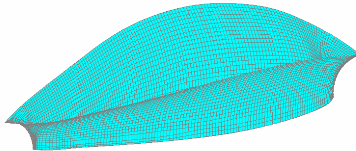
Figure 5.20: CPF sonar dome mesh
