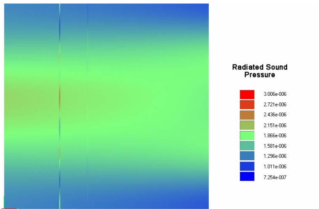
Figure 2.20 . Manta_419Hz_0e-3Damping
