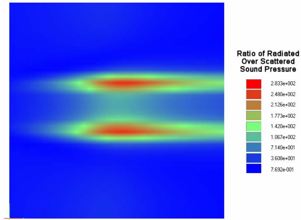
Figure 2.32 . Manta_365Hz_0e-3Damping.RAT
