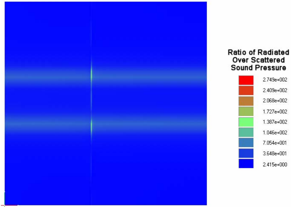
Figure 2.33 . Manta_379Hz_0e-3Damping.RAT
