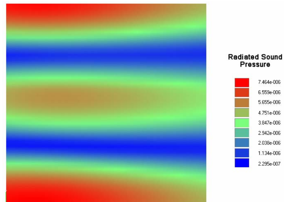
Figure 2.26 . Manta_545Hz_0e-3Damping
