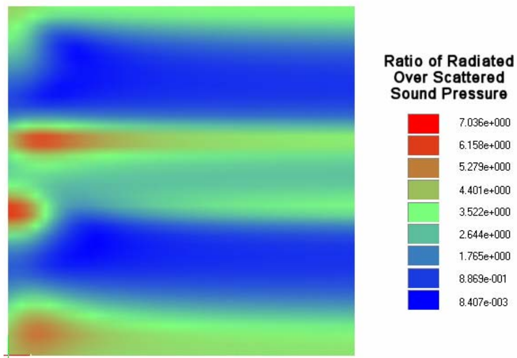
Figure 2.44 . Manta_900Hz_0e-3Damping.RAT
