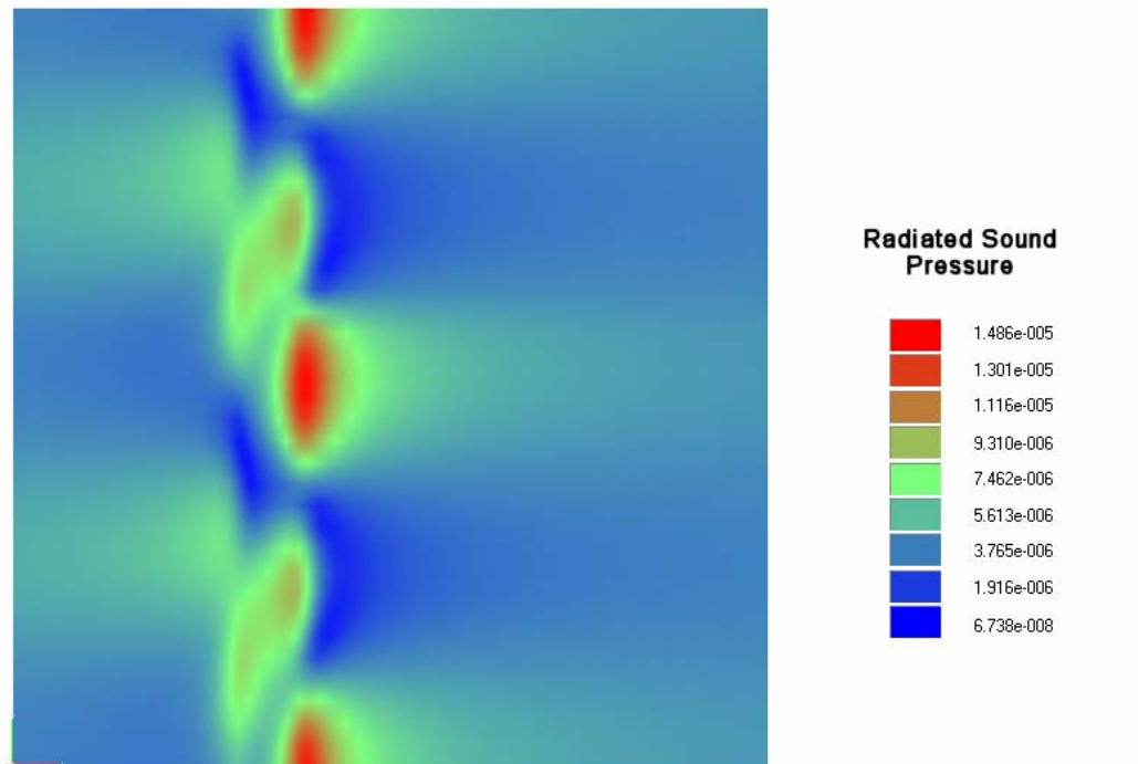
Figure 2.19 . Manta_396Hz_0e-3Damping
