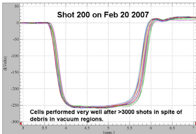
Figure 7. Cells 9-31 were fired at 250 kV for 200 shots at conclusion of the Scaled Accelerator Tests.
