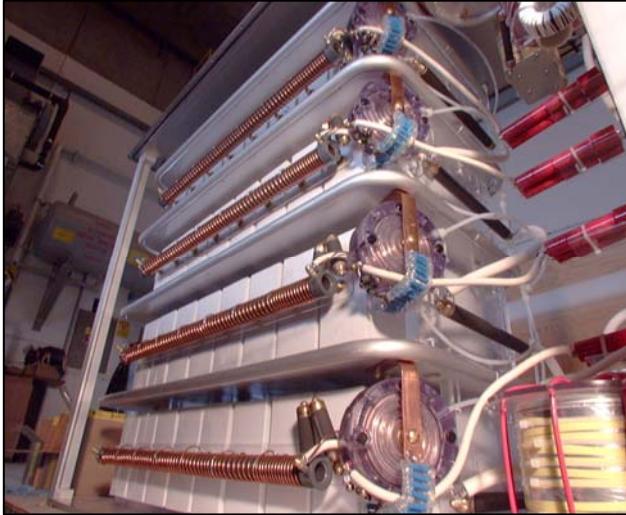
Figure 2. Each cell is driven by an independent PFN/Marx. Each stage is an 8 section PFN.
