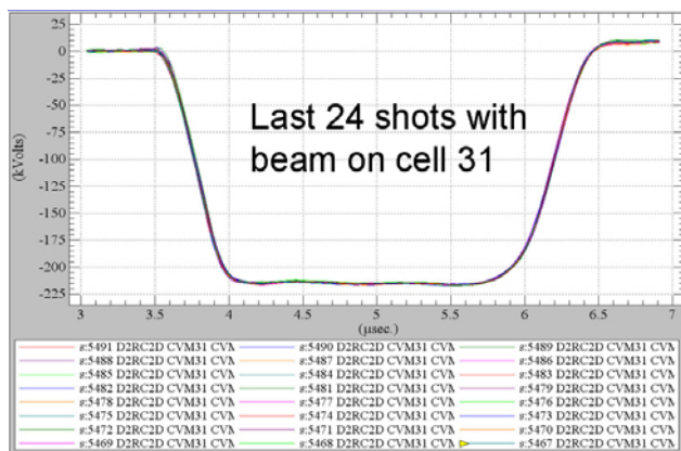
Figure 5. The spread in PFN erection was less than 30ns and the voltage top flat to \pm 1\% for each cell.
