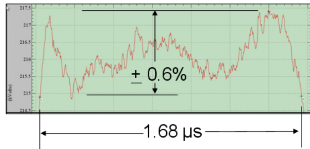
Figure 4b. The average cell voltage on the Scaled Accelerator Test exceeded the design goal of flatness to \pm 1.0\% .
