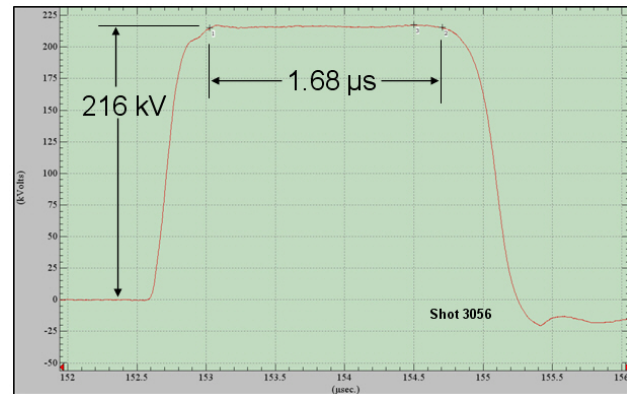
Figure 4a. The average cell voltage on the Scaled Accelerator Test exceeded the design goal of 200 kV per cell.
