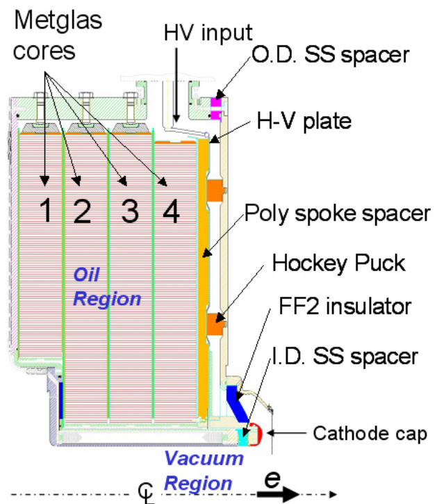
Figure 1. Cross-section of the upgraded DARHT II induction cell.
