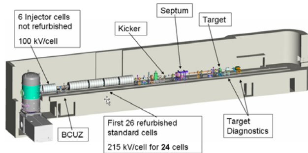
Figure 3. Configuration of the Scaled Accelerator.
