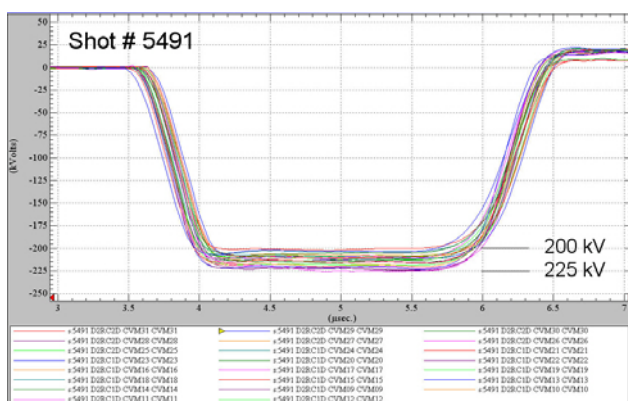
Figure 6. The 24 refurbished cells operated between 200 and 225 kV.
